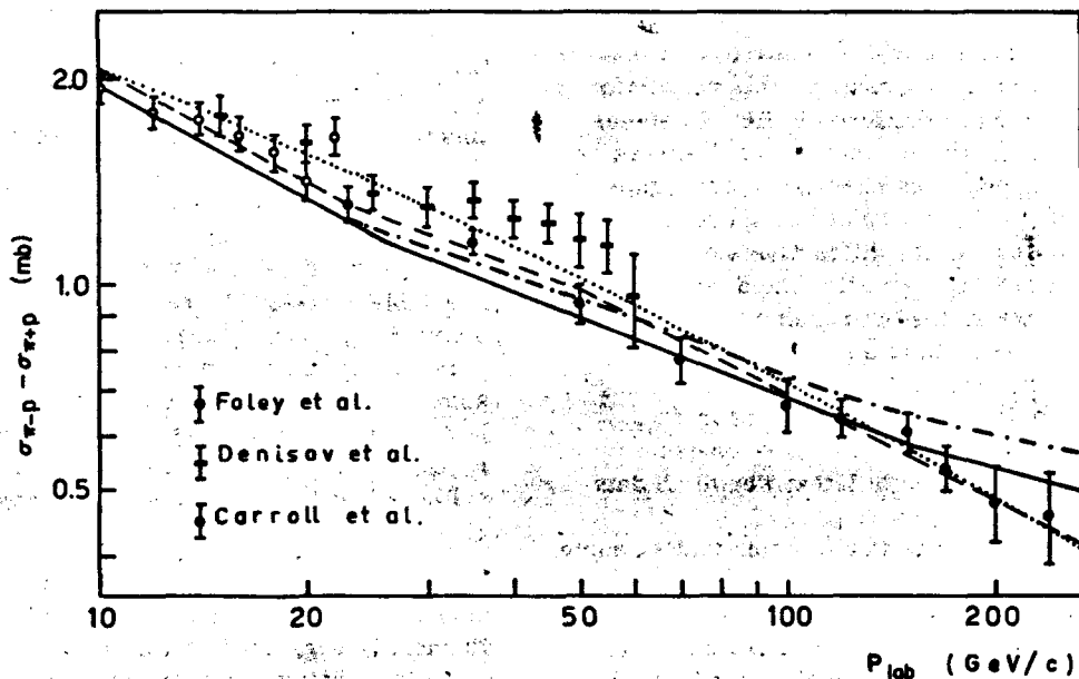
FIG. 1. Difference of \pi^+p and \pi^-p total cross sections (Ref. 5); three-stepped fit of Ref. 1 (solid line), result from Eq. (1) (dashed-dotted line); fit with model of Ref. 10 (dotted line), result from Eq. (1) with one-loop correction of \rho propagator added (dashed line).
