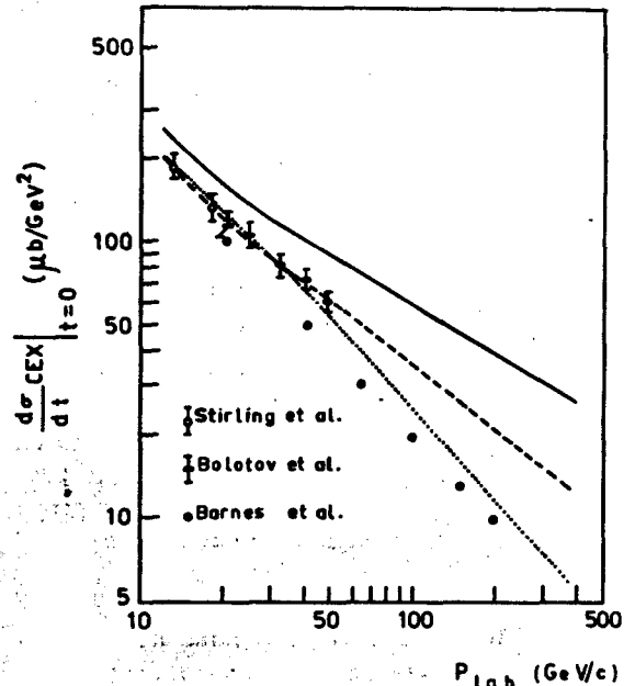
FIG. 2. Forward \pi N charge-exchange differential cross section (Ref. 8); prediction of the model of Ref. 1 with \alpha_p^{(2)}=0.71 asymptotic behavior (solid line), prediction of the same model with \alpha_p=0.5 for p_{\text{lab}}>500 GeV/c (dashed line), prediction of the model of Ref. 10 (dotted line).
