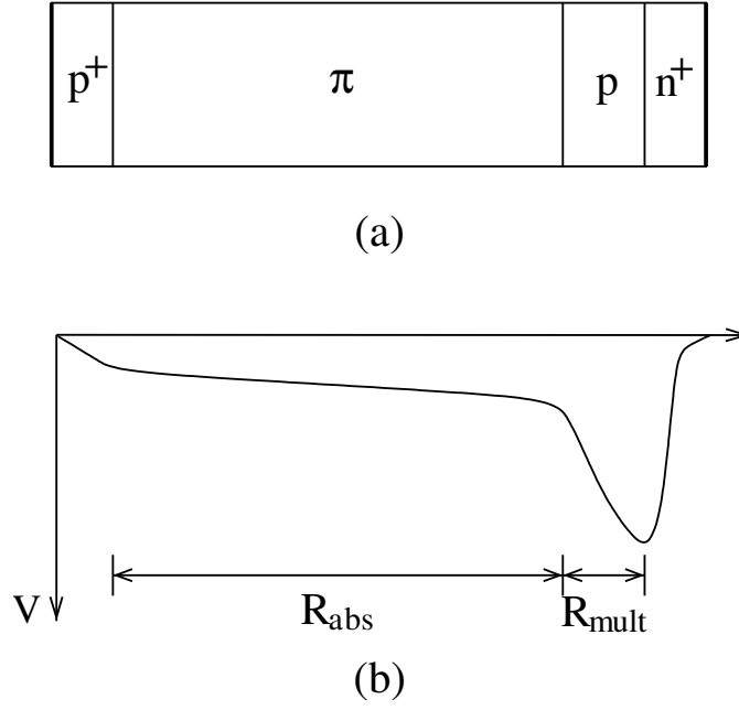
Figure 5.6: (Top) schematics of APD design. \pi represents either a lightly doped p-material or intrinsic material while the superscript (+) refers to heavy doping. P-type region is rich in holes while n-type region is which in electrons. (Bottom) electric field profile of the structure shown in the top panel after applying a reverse bias voltage between n^+ and p^+ [207].
