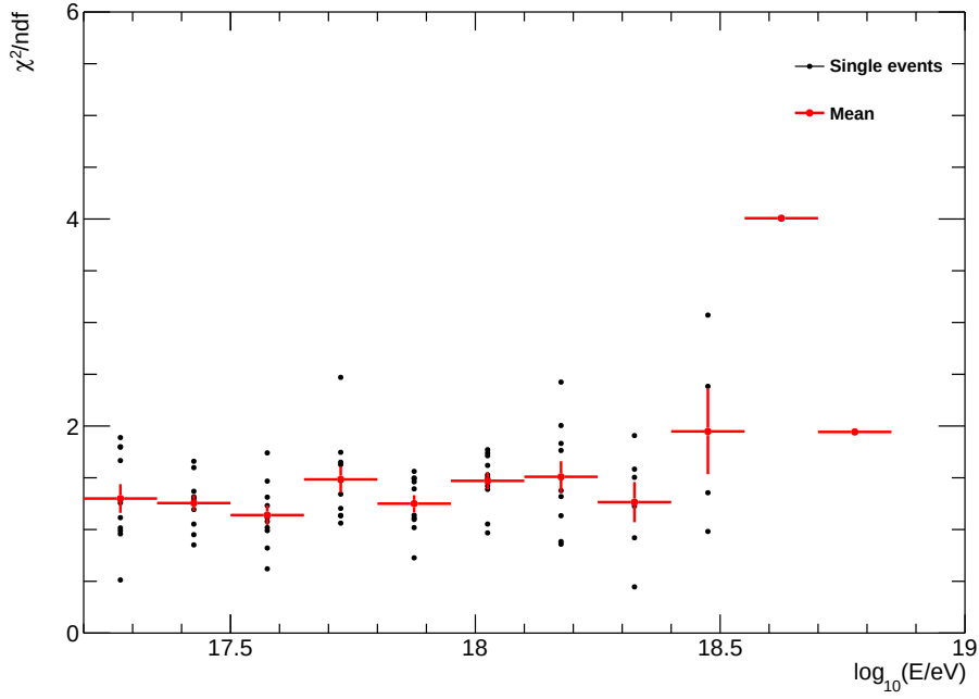
Figure 6.8: The reduced chi-square of the selected MLDFs in terms of the primary energy.
