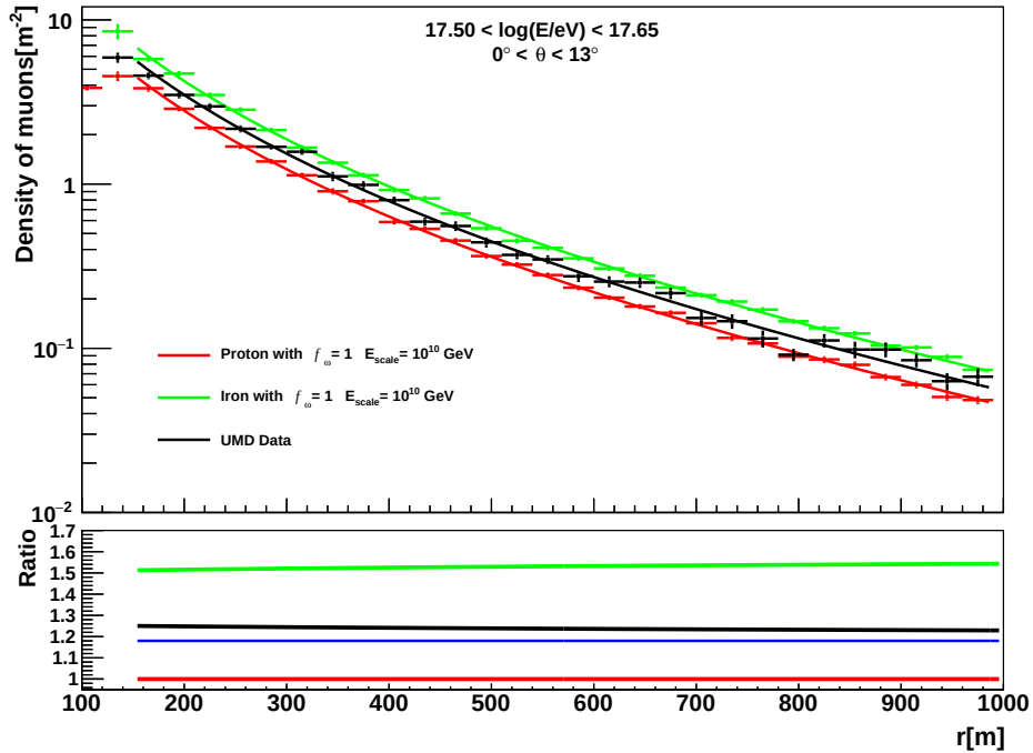
Figure 6.30: Plot analogous to Fig. 6.29 but proton and iron showers are simulated with the conservative core-corona scenario f_{\omega} = 1 and E_{scale} = 10^{10} GeV.
