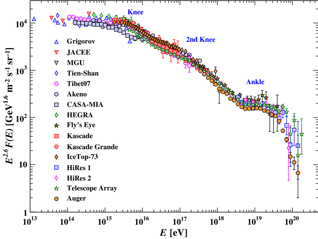
Figure 1.1: Energy spectrum of cosmic rays with the signaling of the knee, the second knee and the ankle [21].
