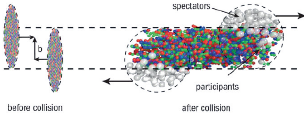
Figure 2.8: A schematic representation of the collision centrality. The ions may collide head-on or may only partially overlap at the collision stage. In the overlap region there are conditions that facilitate QGP formation. [109]
