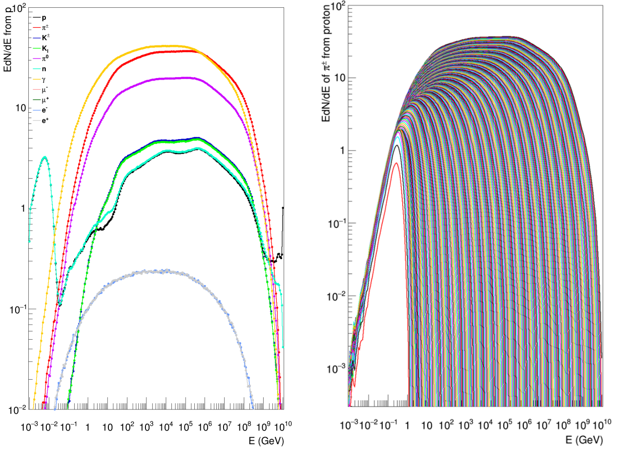
Figure 3.1: Energy spectra in CONEX for EPOS LHC. Left: Spectra of secondary particles in p +air interactions at 10^{19} eV. Right: \pi^\pm spectra in p +air interactions for all proton energies.
