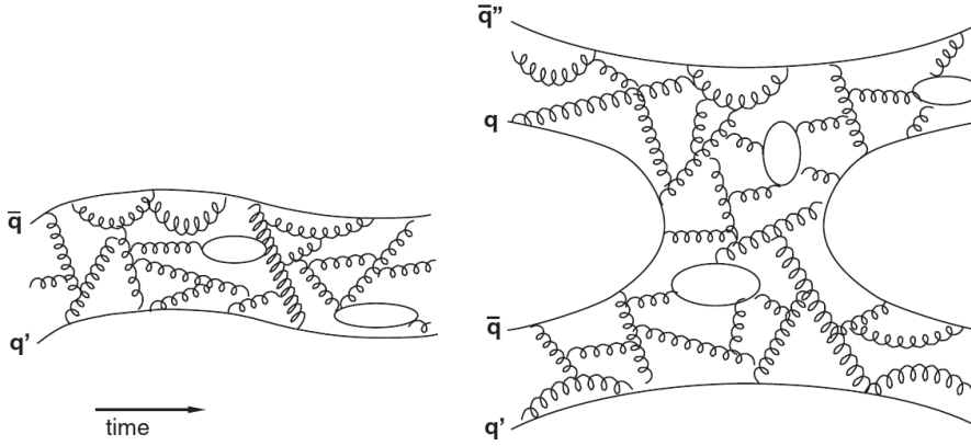
Figure 2.9: Planar diagrams for meson propagation in time (left) and meson–meson interaction (right)
