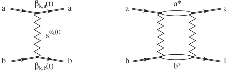
Figure 2.3: Reggeon exchange diagrams. The Regge amplitude is interpreted as a coupling constant together with a reggeon propagator (left). Multiple reggeon exchanges (right).
