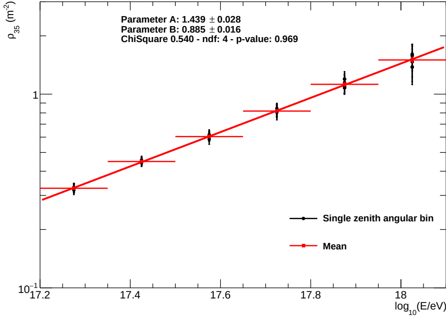
Figure 6.22: Muon densities \rho_{35} as a function of the energy fitted by Eq. 6.8.
