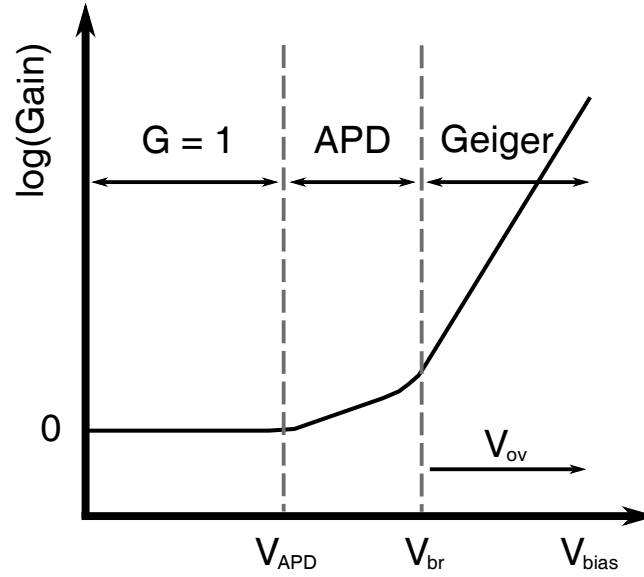
Figure 5.7: Illustration of APD operation modes.[203]
