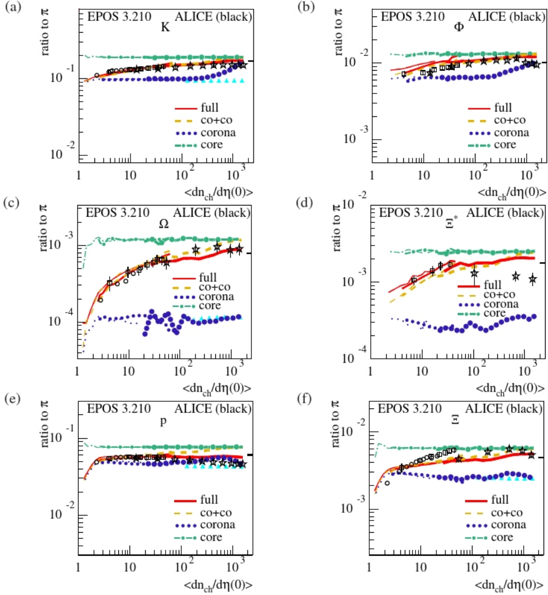
Figure 2.12: Particle to pion ratio for different particle species versus multiplicity, for different contributions for EPOS 3.210 simulations and for the systems pp, pA, AA (slim, medium and thin lines). ALICE data is also plot for the same systems pp, pA, AA (open circles, open squares, open stars). The contribution co-co is for core-corona and full is the core-corona with hadron-hadron rescatterings. Figure from [160].
