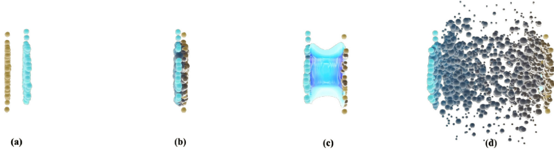
Figure 2.7: Four stages of a heavy-ion collision and its evolution. (a) Shows the two Lorentz contracted heavy-ions moving towards each other in the CM frame, then (b) shows the overlapping nuclei at the collision stage. (c) Just after the collision the heavy-ions travel across each other and generate a volume of high temperature and energy density and finally in (d), the system expands and cools down, eventually fragmenting into hadrons that travel to the detector. [109]
