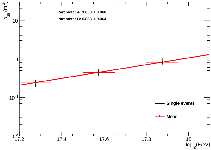
Figure 6.27: Muon densities \rho_{35} as a function of the energy for proton showers.
