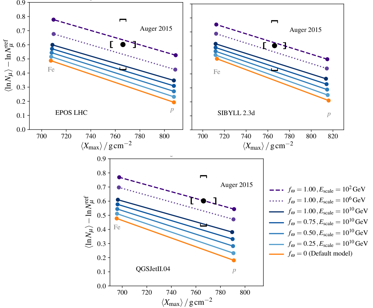
Figure 4.6: Comparison of different core-corona mixing scenarios, as described in the text, on air shower simulations at 10^{19} eV using EPOS LHC (top-left), SIBYLL 2.3D (top-right) and QGSJETII.04 (bottom) in the X_{\text{max}}\text{-}\ln N_\mu plane. The solid lines represent changes in the scale f_\omega , while the dashed lines also indicate the effect of changing E_{\text{scale}} . The default model corresponds to the corona-only simulations. The datum is from the Pierre Auger Observatory [70]. Each model line represents all values that can be obtained for any mixture of cosmic nuclei from proton (bottom right) to iron (top left).
