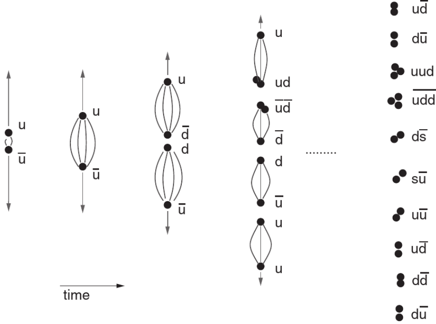
Figure 2.10: Illustration of string fragmentation of a quark–antiquark pair.
