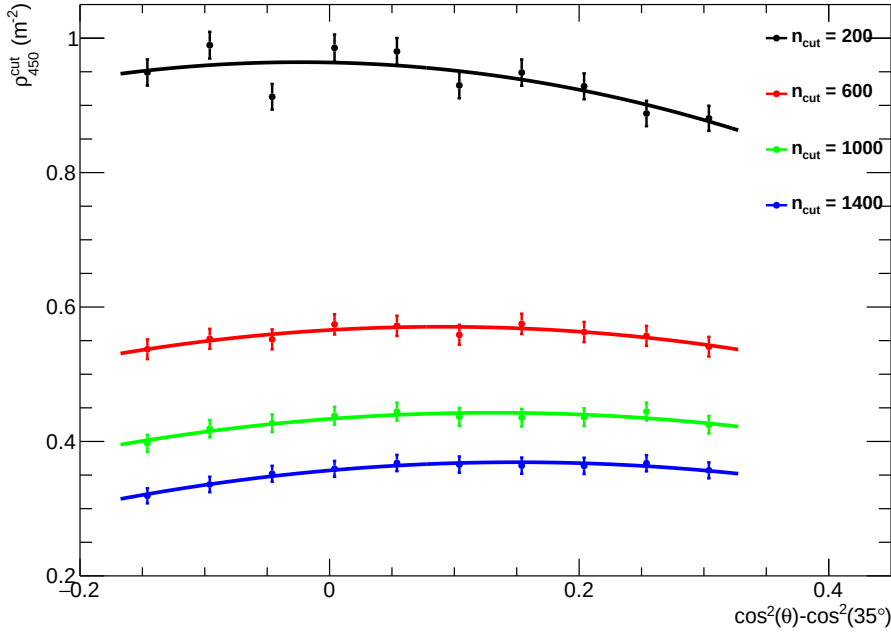
Figure 6.17: The threshold \rho_{450}^{cut} at different constant intensity cuts n_{cut} as a function of \cos^2\theta - \cos^2 35^\circ .
