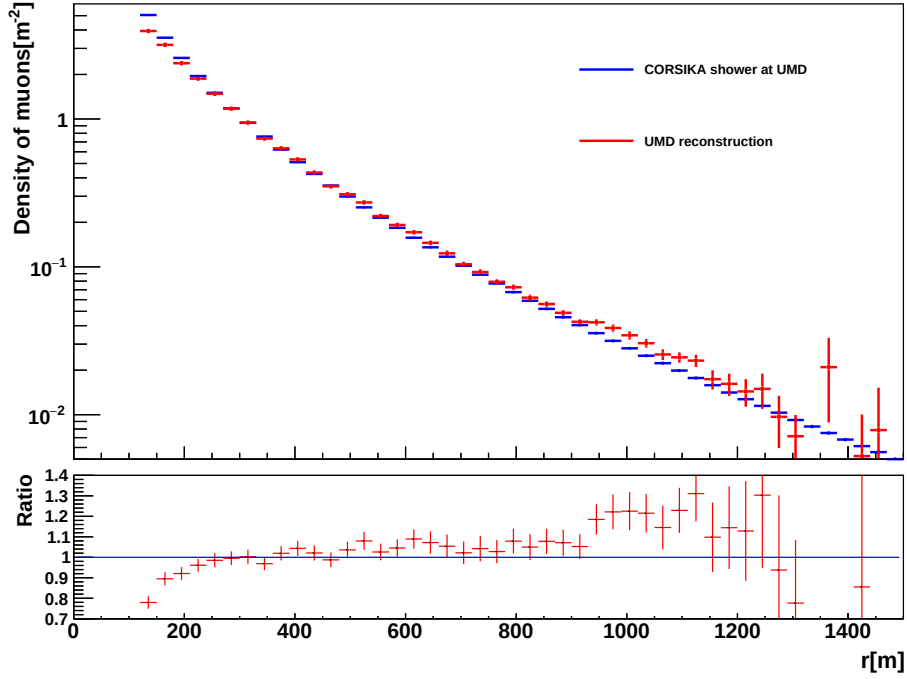
Figure 5.15: MLDF of full MC showers at UMD depth (blue line) and after UMD reconstruction (red line).
