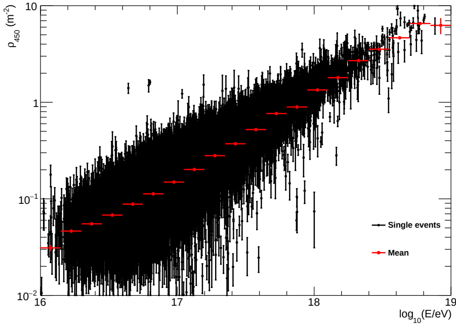
Figure 6.14: The muon density at 450 m from the shower axis obtained from the reconstructed event- wise MLDF using the slope parametrization from Eq. 6.2
