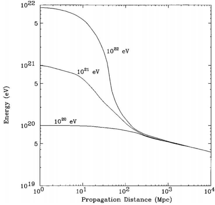
Figure 1.2: Average energy of protons as a function of the distance traveled through the CMB for different initial energy [23].
