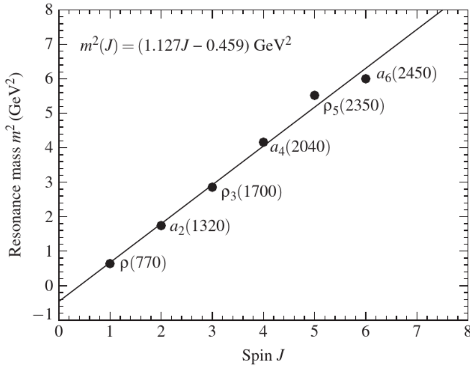
Figure 2.2: Chew–Frautschi plot for the resonances belonging to the \rho(770) trajectory (isospin I=1 , natural parity).
