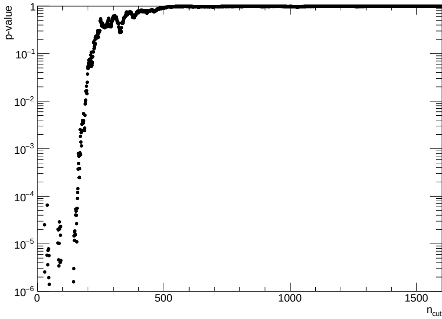
Figure 6.19: The p-value of the quadratic fits to \rho_{450}^{cut} with \cos^2\theta - \cos^2 35^\circ profiles.
