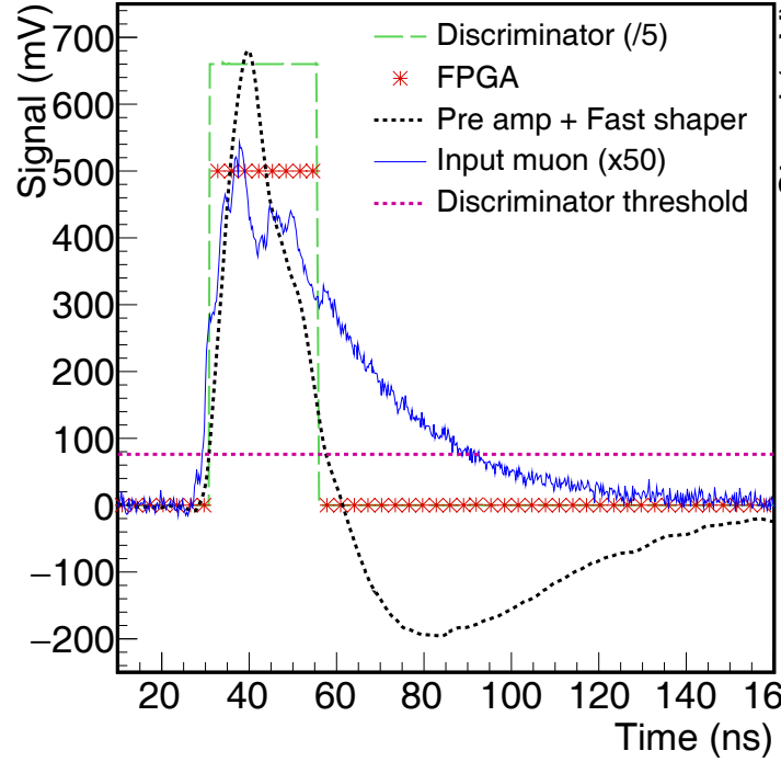
Figure 5.8: A simulated single-muon trace in the binary mode. The signal from the SiPM and the discriminator pulse are re-scaled for illustration. The FPGA outputs a “1”-bit in the binary trace when the fast-shaper output is above the discriminator threshold. [203]
