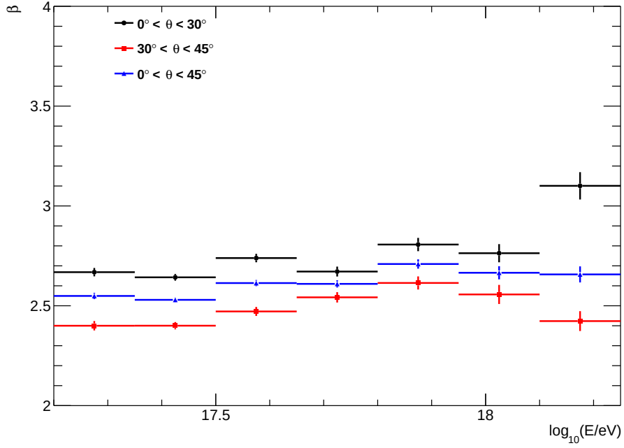
Figure 6.12: The evolution of the weighted average MLDF slope \beta as a function of the primary energy considering all zenith angles together and discriminating by angular bands.
