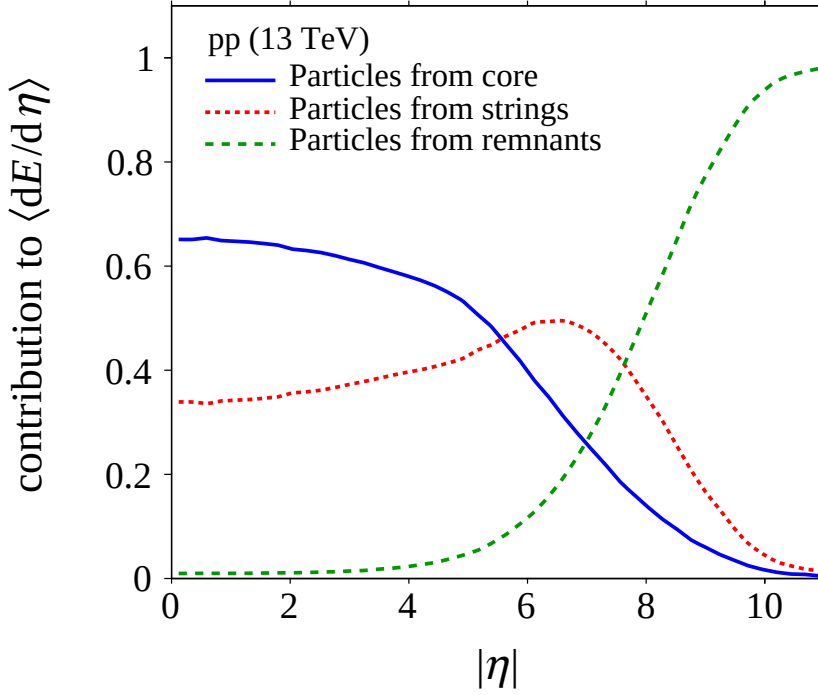
Figure 4.3: Fractional contribution of particles originating from different production mechanisms to the total energy density dE/d\eta as predicted by EPOS LHC as function of |\eta| [192].
