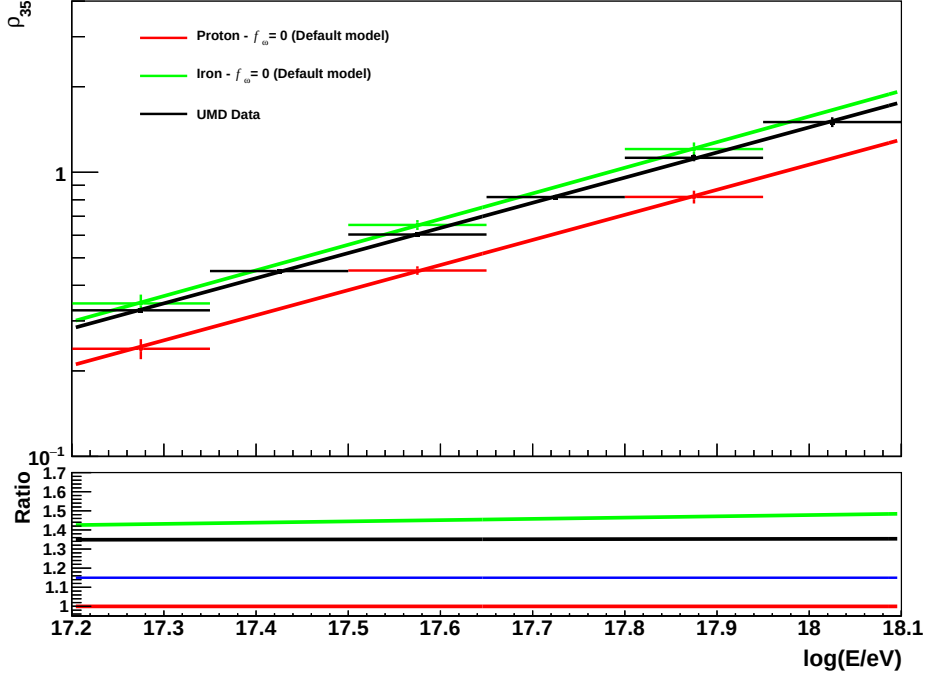
Figure 6.31: Mean \rho_{35} as a function of the energy for UMD data and shower simulations of a primary proton and iron with the default EPOS LHC model. Blue line in the bottom plot is the expected data ratio from mass composition measurements.
