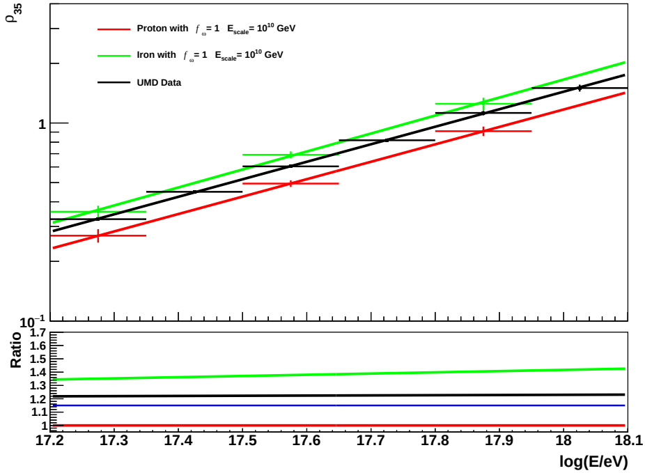
Figure 6.32: Mean \rho_{35} as a function of the energy for UMD data and shower simulations of a primary proton and iron with the EPOS LHC model in a conservative core-corona mixing scenario. Blue line in the bottom plot is the expected data ratio from mass composition measurements.
