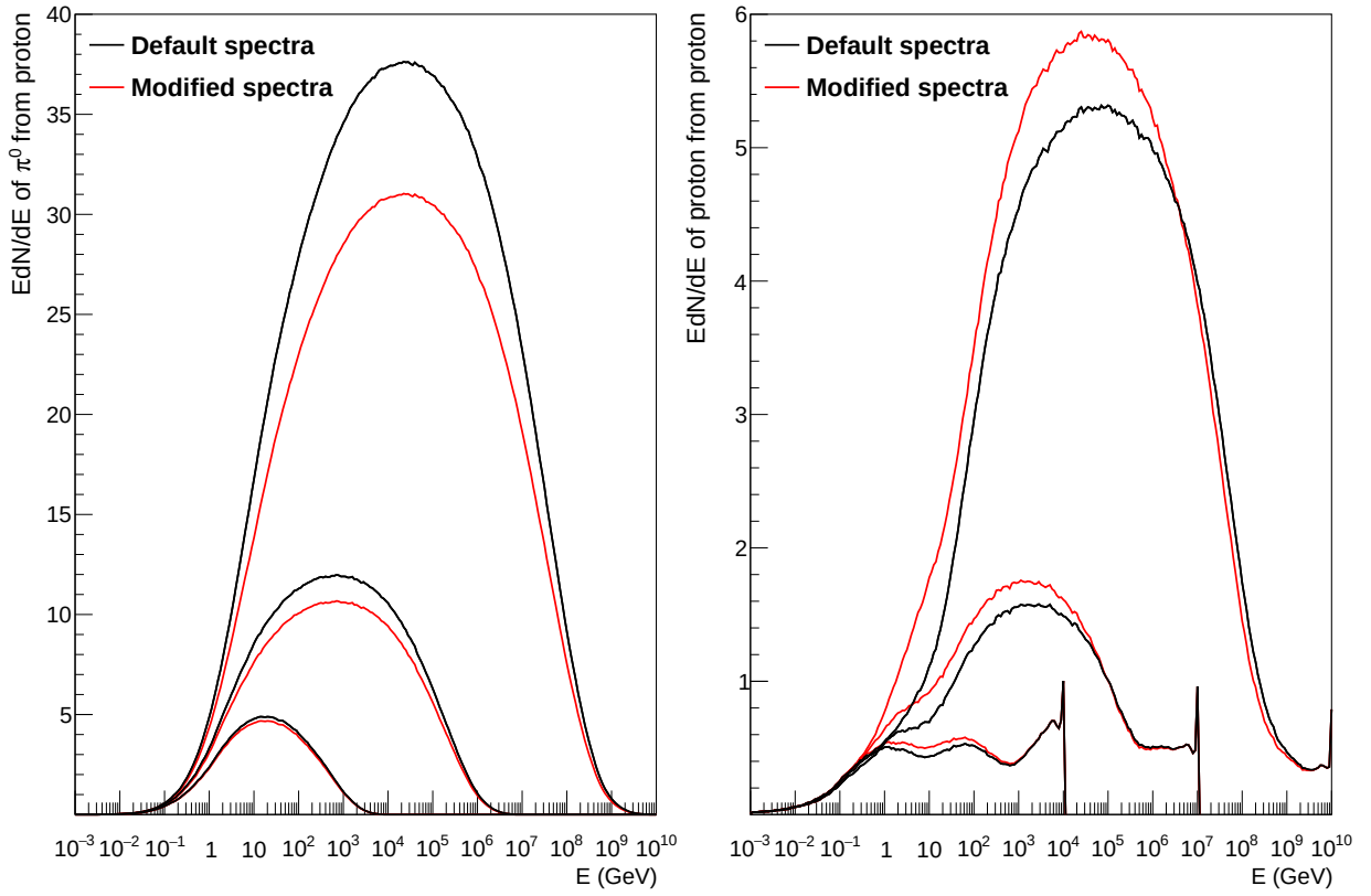
Figure 3.8: Default and modified spectra of secondary \pi^0 (left) and proton (right) at three different proton-projectile energies for QGSJETII.04.
