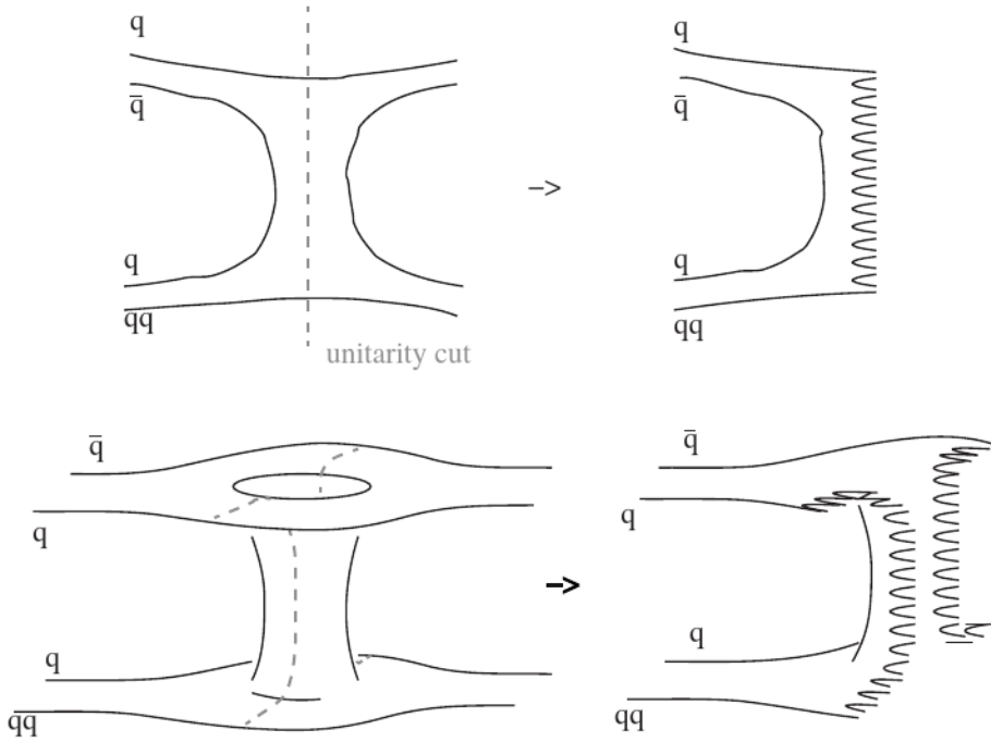
Figure 2.4: Color flow topologies of elastic scattering due to reggeon (top left) and pomeron (bottom left) exchange and the expected particle distributions (right) for inelastic interactions.
