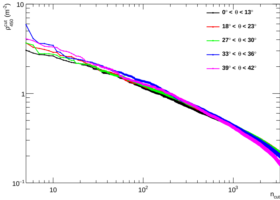
Figure 6.16: The threshold \rho_{450}^{cut} as a function of the constant intensity cut n_{cut} .
