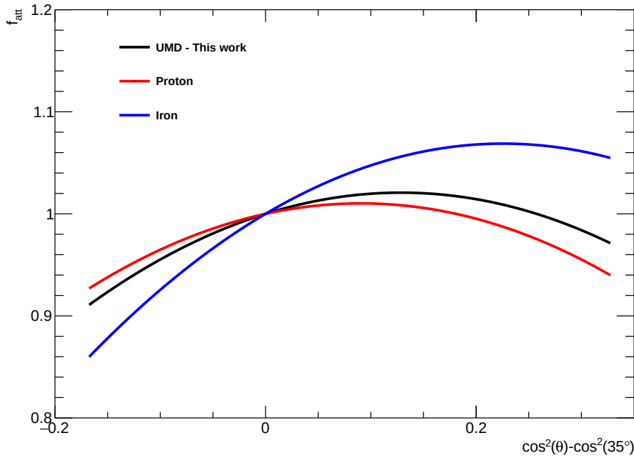
Figure 6.26: Comparison of the attenuation curve obtained in the UMD data analysis and the corresponding for proton and iron simulations.
