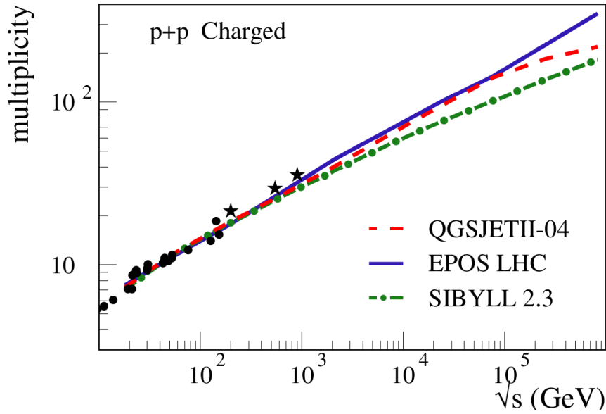
Figure 4.5: Averaged multiplicity as a function of center of mass energy. Lines are simulations and points are data [194].
