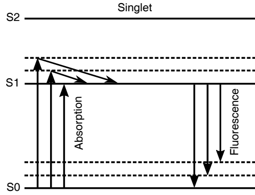
Figure 5.2: Schematics of the fluorescence mechanism in organic scintillators. The incident radiation transfers energy to electrons in the material, which are promoted from the ground state S_0 to vibrational levels of the singlet S_1 . Before the electrons return to the ground state S_0 , they lose part of the energy absorbed and go from the vibrational levels to fundamental level of S_1 . Then, by emitting fluorescence photons, the electron relaxes to the ground state. Diagram adapted from [206].
