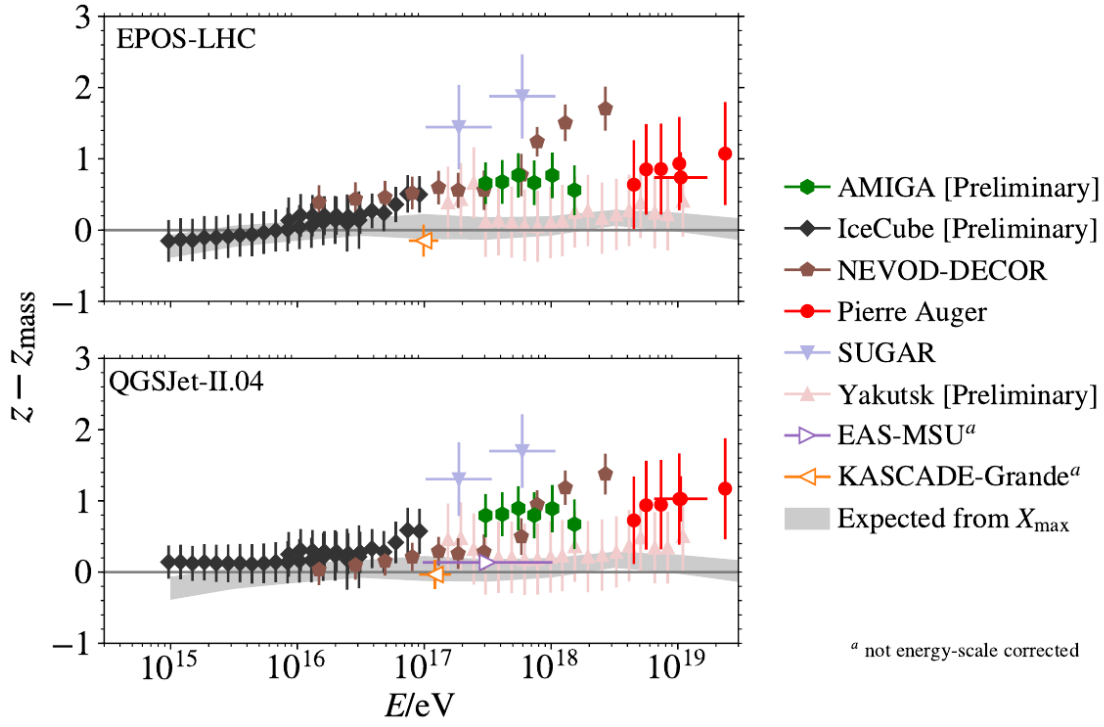
Figure 1.15: Data from Fig. 1.14 after subtracting z_{mass} . The points for KASCADE-Grande and EAS-MSU cannot be cross-calibrated and are only included for comparison.[80]
