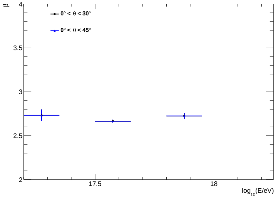
Figure 6.24: The evolution of the weighted average MLDF slope \beta as a function of the primary energy considering all zenith angles together and discriminating by angular bands for simulated proton showers.
