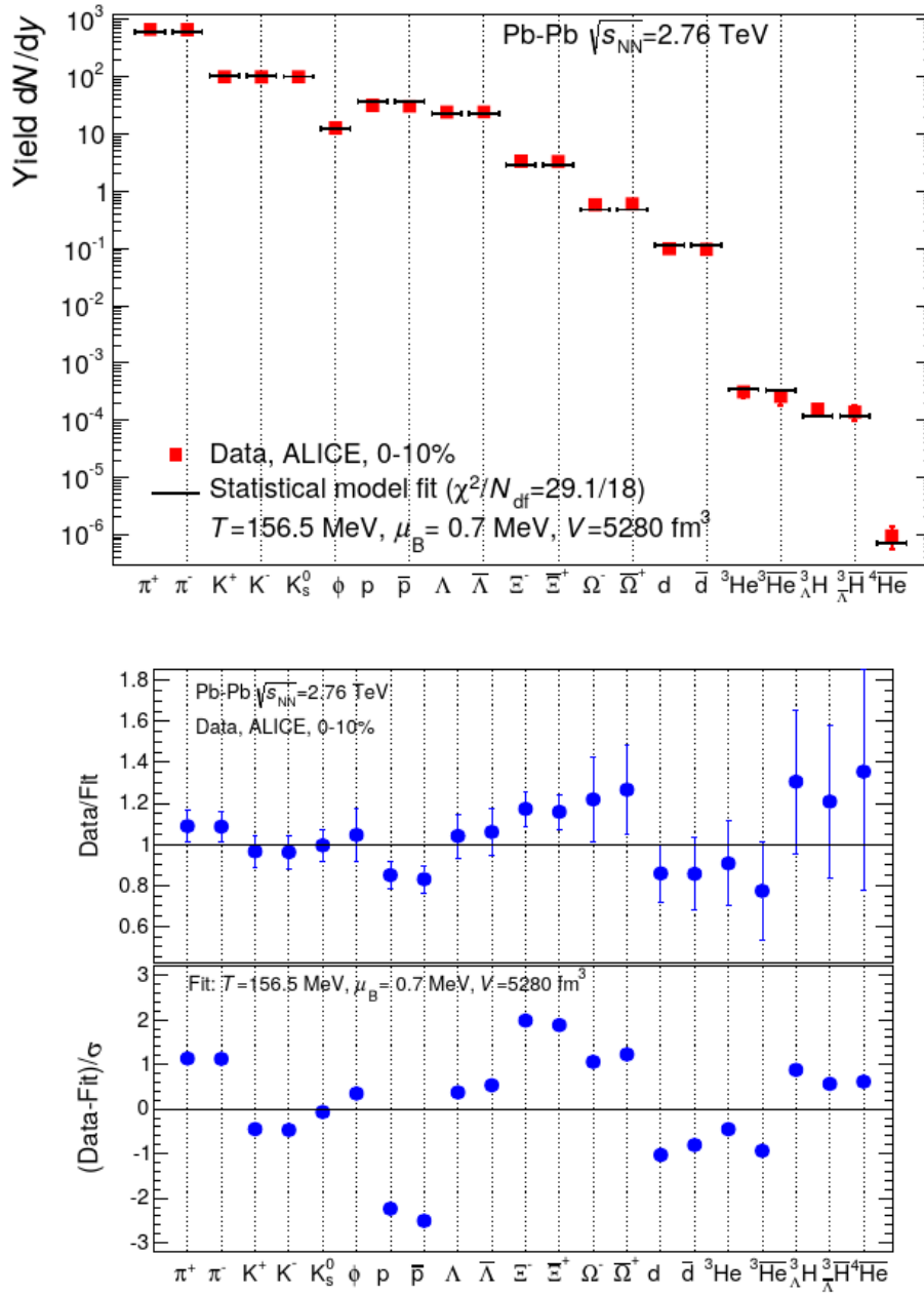
Figure 2.11: Hadron multiplicities in central (0-10%) Pb-Pb collisions at the LHC and best fit. The lower panels show the ratio of data value to fit and the difference between data and model fit in units of the experimental uncertainty. Fig. from [131].
