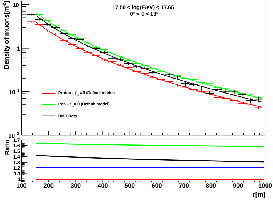
Figure 6.29: MLDF of proton and iron showers for the default EPOS-LHC model, i.e. f_{\omega} = 0 , with UMD reconstruction and UMD data. Blue line in the bottom plot is the expected data ratio from mass composition measurements.
