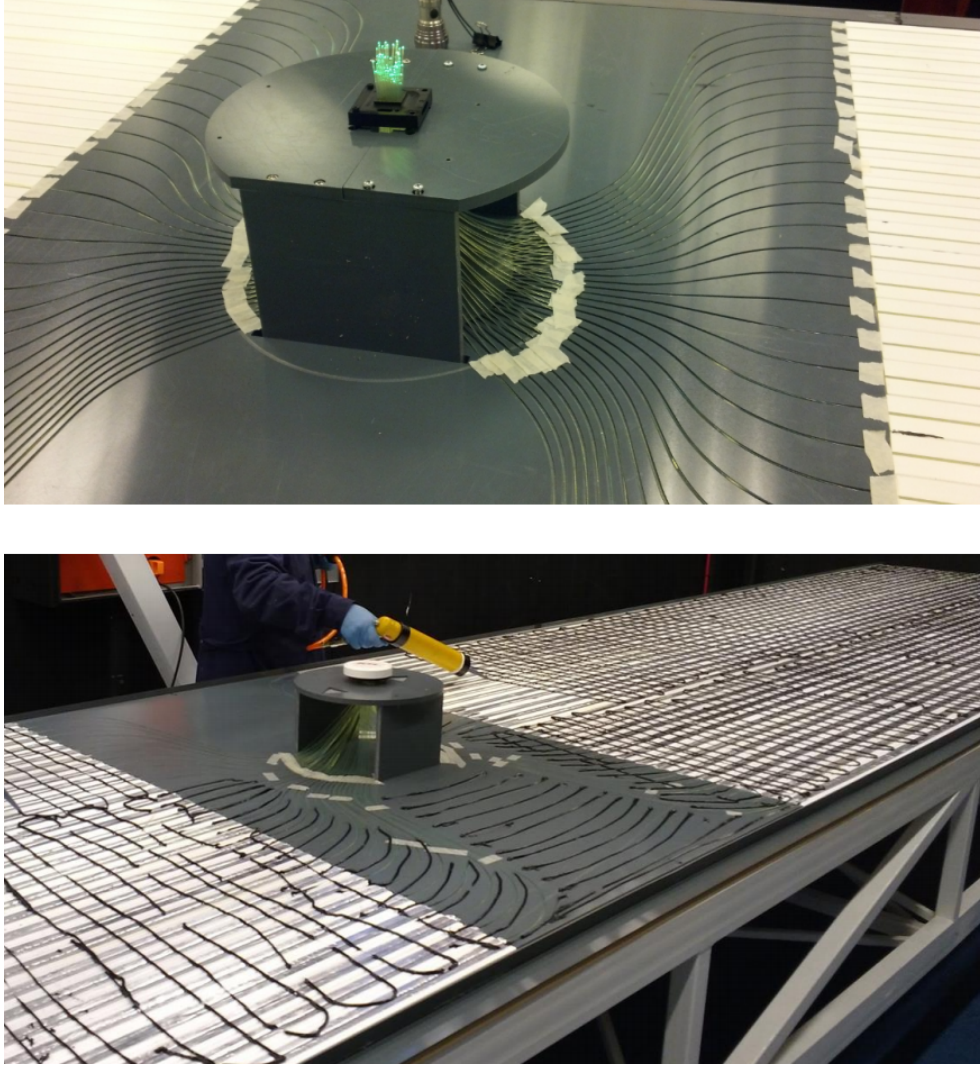
Figure 5.1: UMD module under construction. (Top) the optical connector with wavelength-shifting optical fibers, before polishing, is displayed. (Bottom) 64 plastic scintillator strips are shown, before closing the PVC casing.[203]
