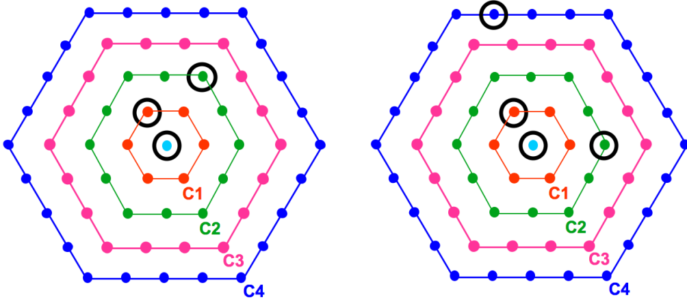
Figure 1.6: Example of T3 configurations: the 3-fold T3 mode ToT2C1&3C2 is shown on the left and the 4-fold mode 2C1&3C2&4C4 on the right (see text for the definitions). C1, C2, C3, C4 indicate the first, second, third and fourth sets of neighbors, respectively, at 1.5, 3, 4.5 and 6 km from a given detector
