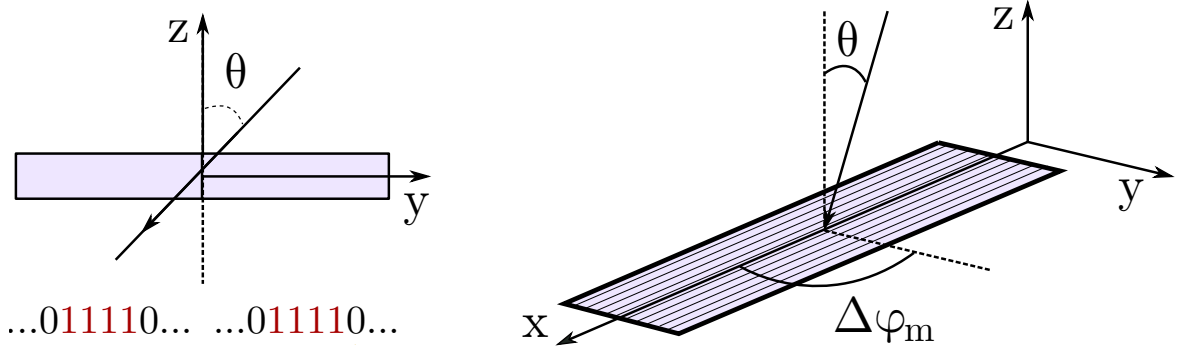
Figure 5.14: (Left) schematic of frontal view of two scintillator strips and an impinging muon depositing energy in both. An example of the binary output of the binary mode for this event is also shown. (Right) schematic of the geometric dependency of corner clipping muons. The probability of finding the muon signal in two adjacent strips depends both on the zenith angle of the shower axis ( \theta ) and on the difference between the azimuth angle of the shower axis and the orientation of the UMD module ( \Delta\phi_m ) [203]
