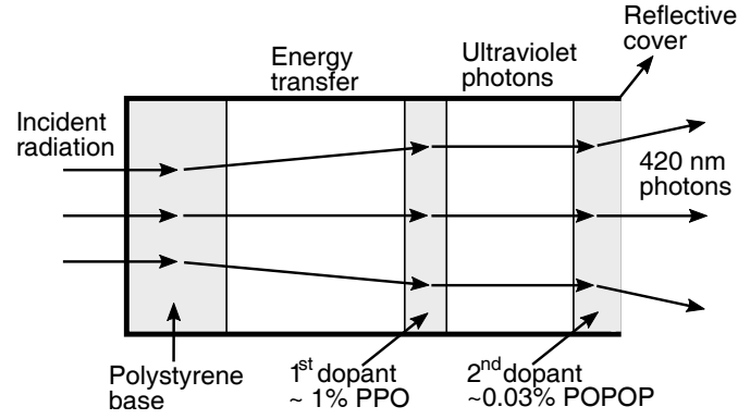
Figure 5.3: Diagram of mechanisms inside a plastic scintillator. Two dopants are mixed homogeneously in a plastic base. Picture adapted from [207].
