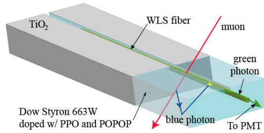
Figure 5.4: Schematic of the UMD scintillator with embedded optical fiber. Plastic scintillators emit blue photons in response to the passage of a particle. Then, the blue photons are absorbed with the WLS optical fiber and re-emitted into green photons that are propagated towards a photo-detector [209].
