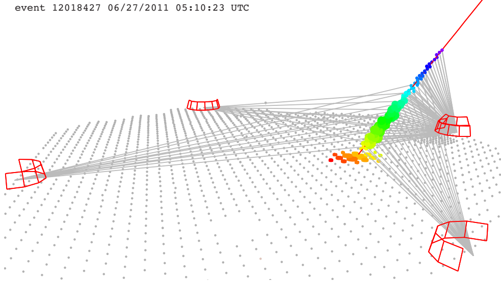
Figure 1.4: Example of an event simultaneously measured by both the SD and the FD at the Pierre Auger Observatory [40]. Colors denote different shower times at both shower axis and ground. The size of the markers correspond to the magnitude of measured signals at the ground and of the reconstructed energy at the shower axis. Red squares illustrate the field of view of the 27 fluorescence telescopes, the viewing directions of triggered pixels are shown as gray lines. The surface detector stations are displayed as gray dots. The obtained energy and X_{\max} from FD data was: E = (4.7 \pm 0.1) \times 10^{19} eV and X_{\max} = (730 \pm 3) g/cm 2 .
