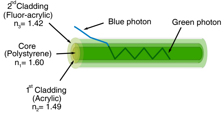
Figure 5.5: WLS optical fiber diagram. The core and the two claddings are illustrated.[203]
