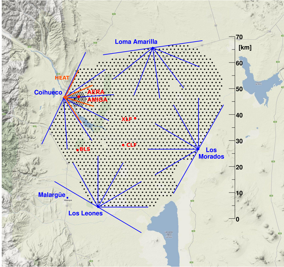
Figure 1.3: Map of the hybrid detector at the Pierre Auger Observatory. Each black dot corresponds to one of the 1660 surface detector stations (see section 1.4.2). The 24 fluorescence detector enclosures are shown, each with a 30^\circ field of view distributed in four buildings (see section 1.4.4). The location of the low-energy enhancements are also displayed (see section 1.4.5)
