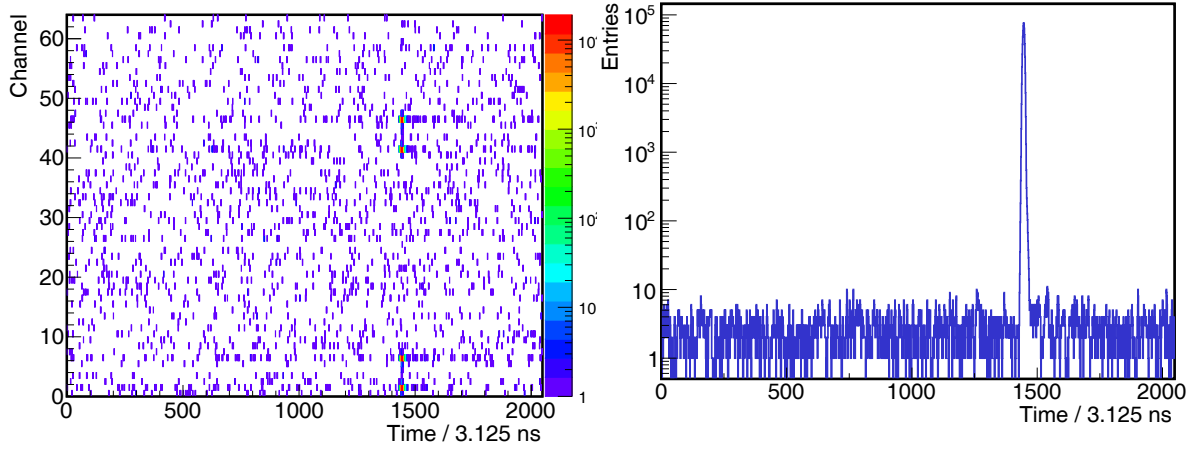
Figure 5.12: (Left) Number of events per channel and time bin for a discriminator threshold of 2.5 PE. Channels 2, 7, 42 and 47 are coupled to optical fibers; positive samples are accumulated around the trigger bin. Channels 4, 25, 44 and 59 have no positive samples as they were off. (Right) time projection of positive samples in all channels per time bin. The peak at the trigger bin can be seen, along with the background noise.[203]
