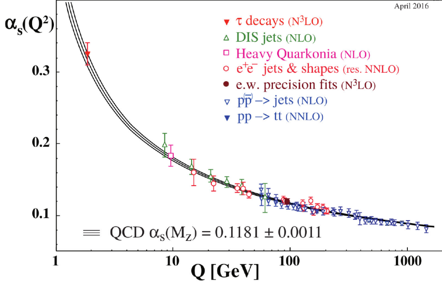
Figure 2.5: Measurements of \alpha_s as a function of the energy scale Q , as reported in the Quantum Chromodynamics review of the Particle Data Group [106]. From each set of experiments, there is a value of \alpha_s that has been extracted using different levels of QCD perturbation theory, which are indicated in brackets
