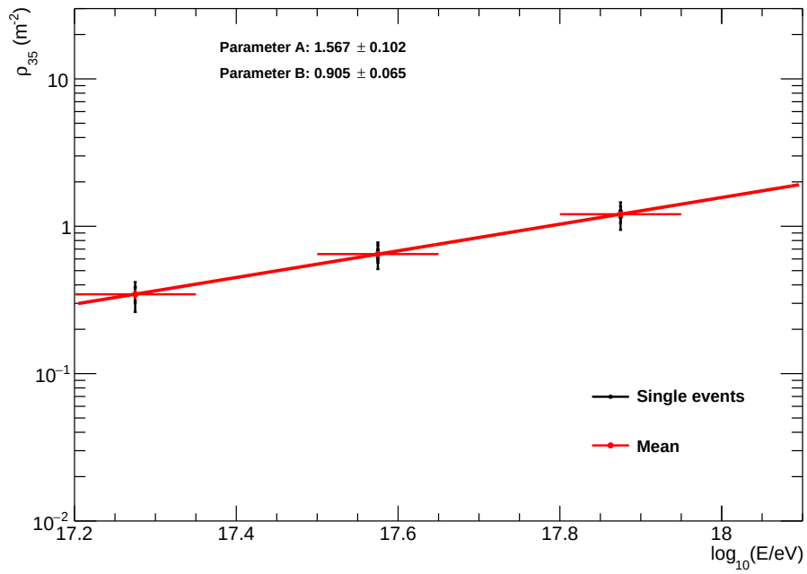
Figure 6.28: Muon densities \rho_{35} as a function of the energy for iron showers.
