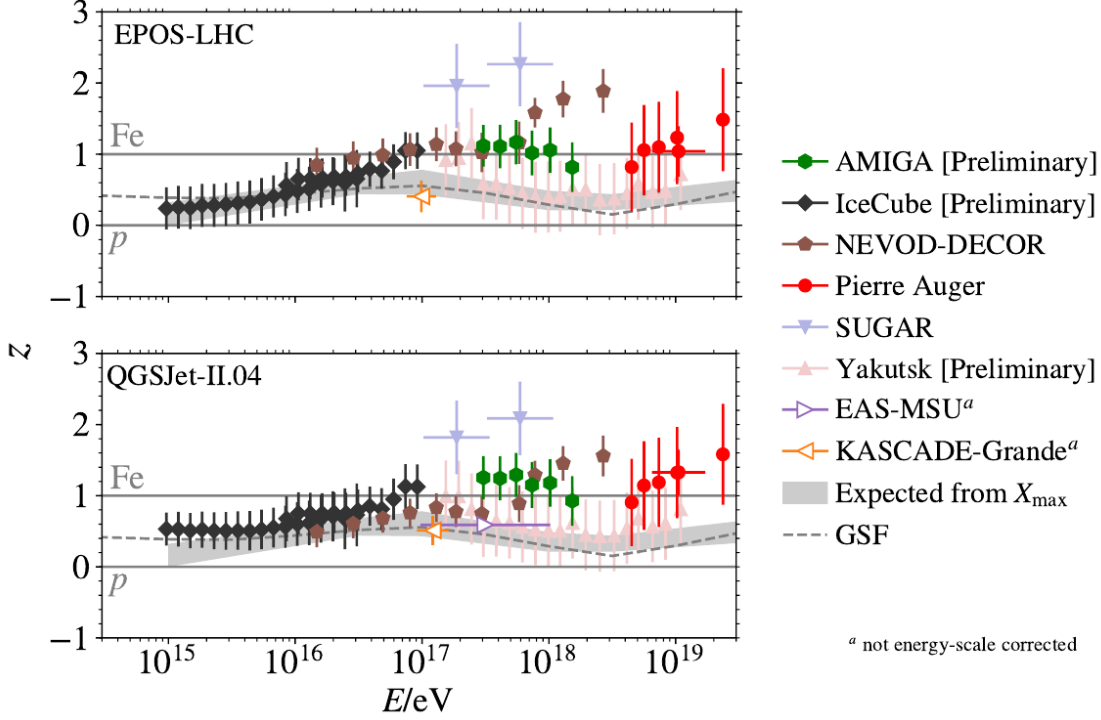
Figure 1.14: Data from Fig. 1.13 after applying energy-scale cross-calibration. The points for KASCADE-Grande and EAS-MSU cannot be cross-calibrated and are only included for comparison.[80]
