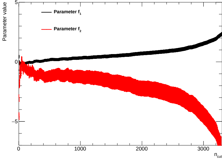
Figure 6.18: The coefficients of the attenuation function f_{att} versus n_{cut} .
