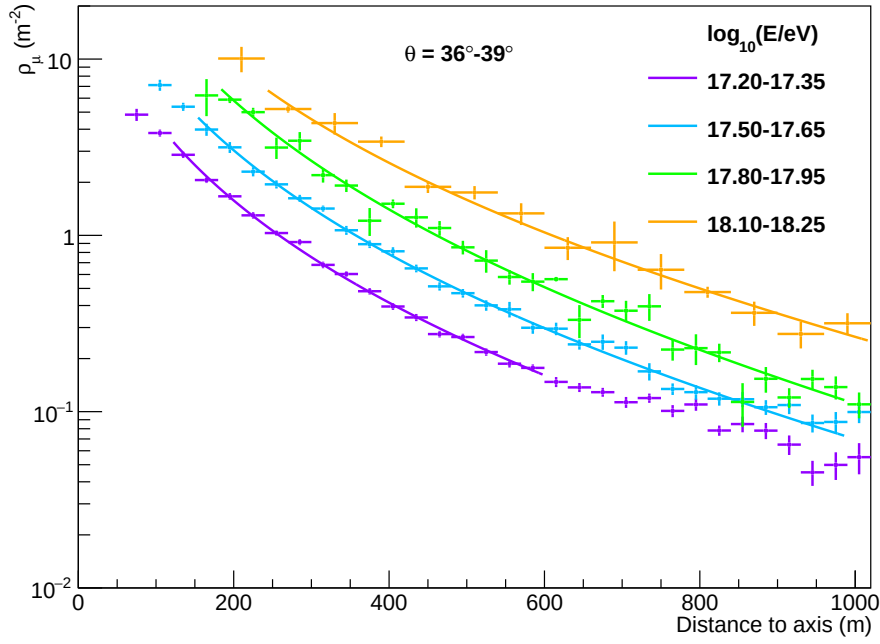
Figure 6.10: Some of the accepted MLDFs of the zenith bin \theta = (36^\circ - 39^\circ) .
