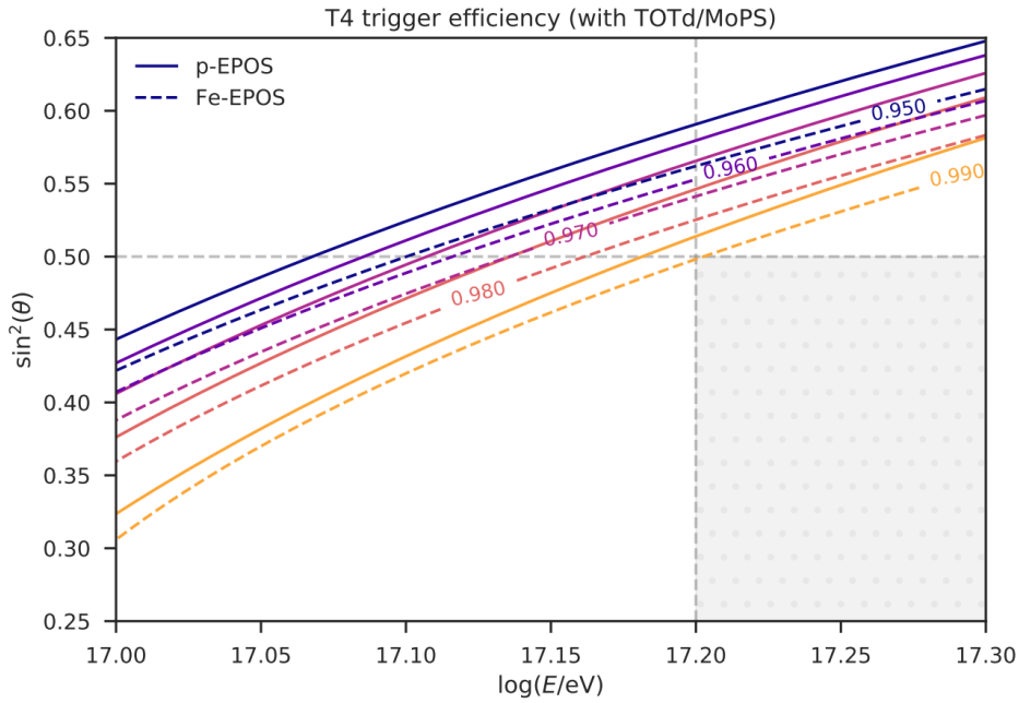
Figure 6.5: T4 trigger efficiency for proton and iron showers for the EPOS model in a zenith angle vs energy plot. Plot by F. Gesualdi from [221].
