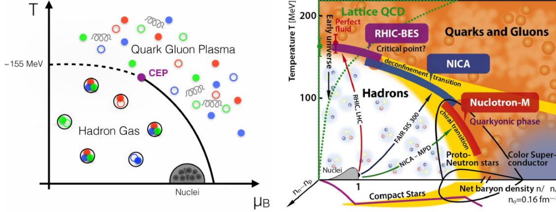
Figure 2.6: On the left, the phase diagram for QCD matter shows the Hadron Gas phase and the Quark-Gluon Plasma phase in the temperature ( T ) - baryon chemical potential ( \mu_B ) plane [107]. On the right, the phase diagram for QCD matter shows the Hadron Gas phase, the Quark-Gluon Plasma phase and the Quarkyonic phase in the temperature ( T ) - baryon density ( n ) plane. Here n is normalized to the cold nuclei baryon density n_0 [108].
