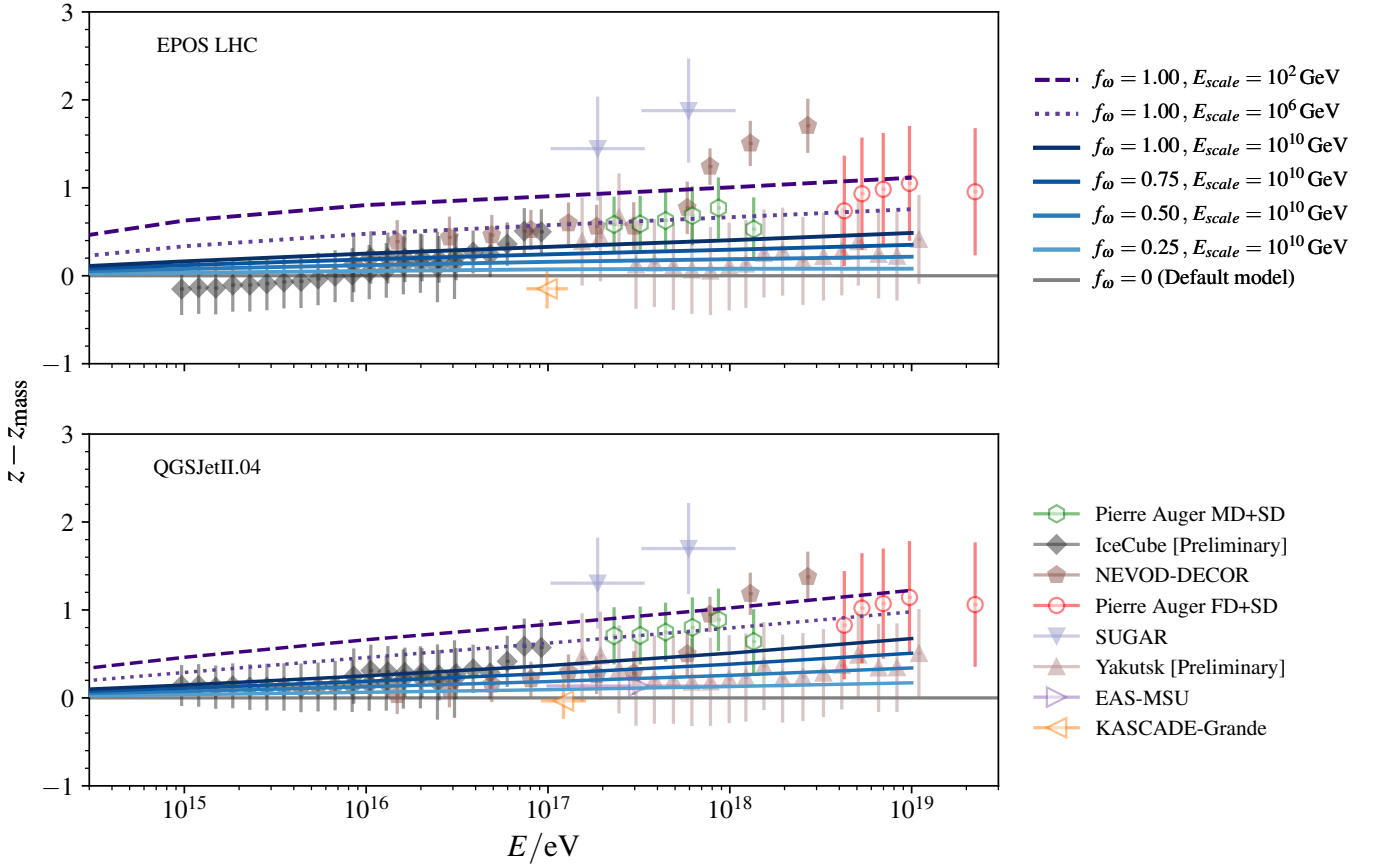
Figure 4.8: Evolution of the mass corrected z -scale, \Delta z = z - z_{\text{mass}} , as a function of the primary energy. z values are taken from [80] and the updated Auger data from [197]. Overlaid are predictions obtained from changing the scale f_\omega (solid lines) and E_{\text{scale}} (dashed and dotted lines) obtained with EPOS LHC (top) and QGSJETII.04 (bottom) air shower simulations.
