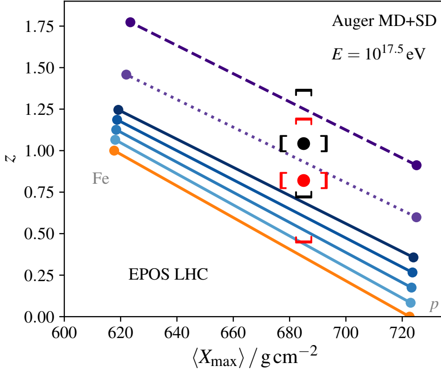
Figure 6.33: Fig. 4.7 including the UMD data (red point ) calculated in this study.
