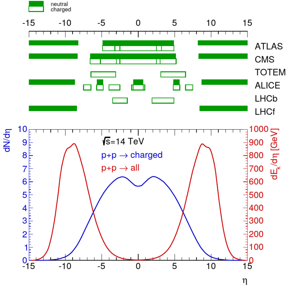
Figure 2.1: Energy and particle flow at \sqrt{s} = 14 TeV as a function of pseudorapidity at the LHC. The green bands represent the coverage of different detector components. Plot by R. Ulrich.
