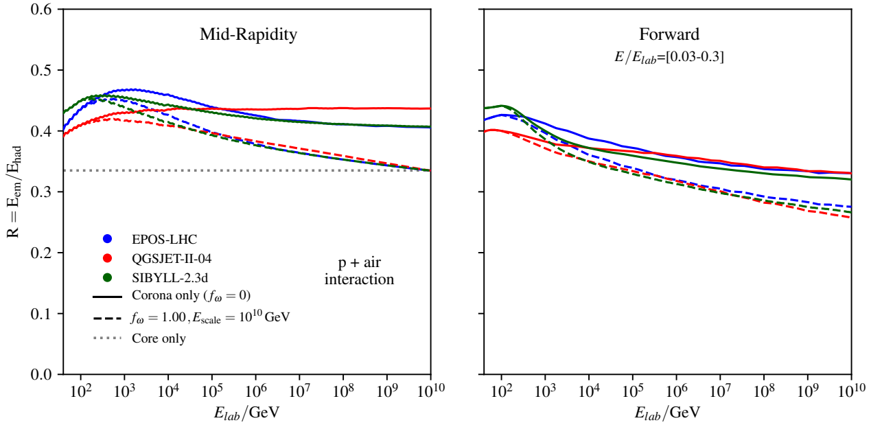
Figure 4.2: R values as a function of the projectile energy E_{\text{lab}} at mid-rapidity (left) and forward 0.03 \leq x_F \leq 0.3 (right) for the default models (solid line) and the modified one with f_{\omega} = 1.00 and E_{\text{scale}} = 10^{10} GeV (dashed lines) where R reaches the value given by the statistical model at the maximum energy.
