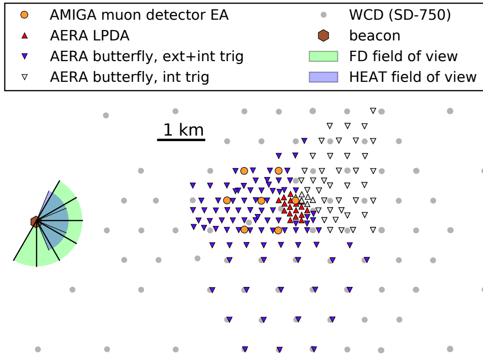
Figure 1.9: Map of the low-energy enhancements area adapted from [46]. It comprises AMIGA, HEAT, and AERA. The different AERA antennas, the SD-750 stations, the AMIGA muon detectors and HEAT field of view are shown.
