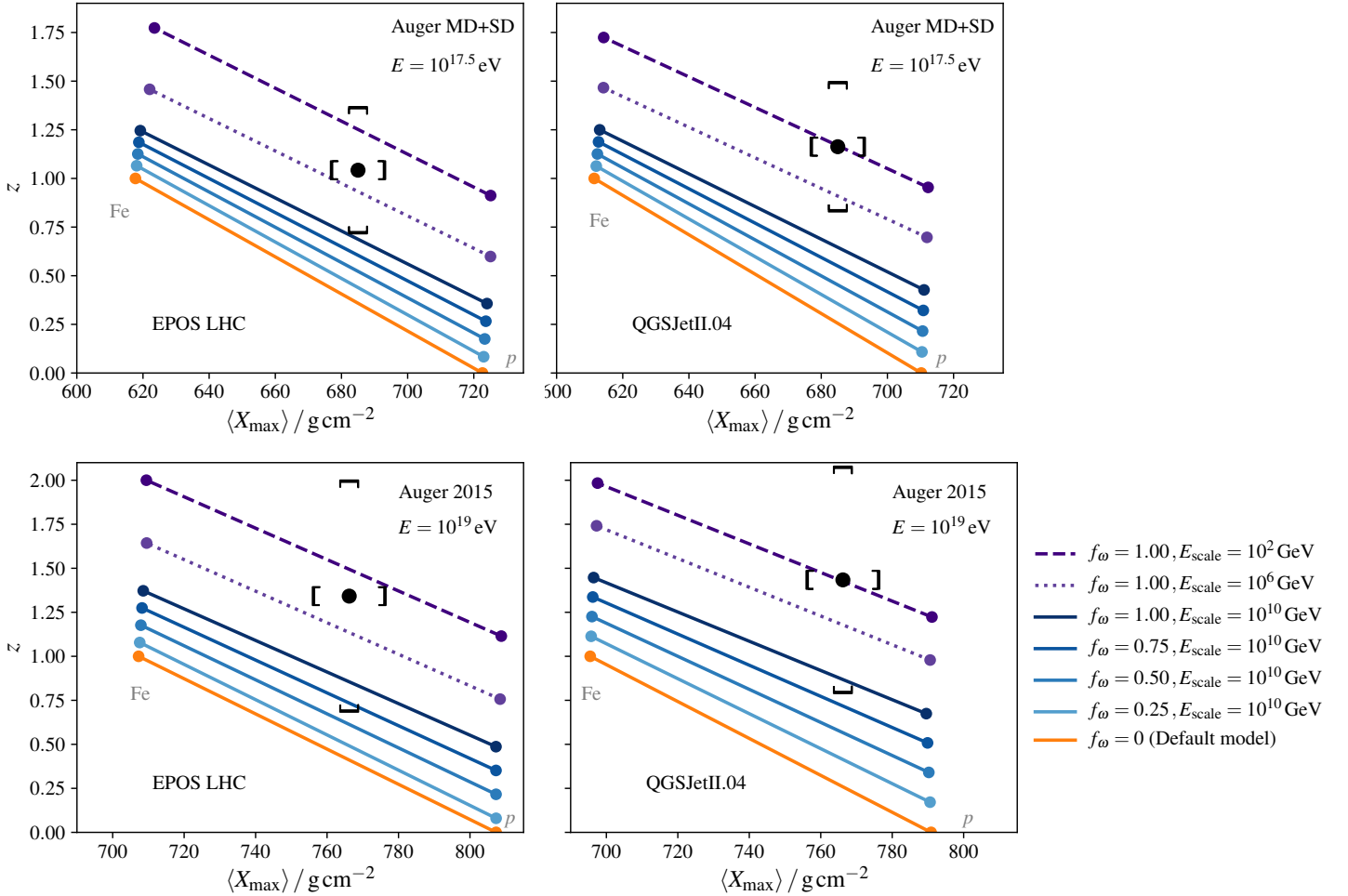
Figure 4.7: Comparison of different core-corona mixing scenarios on air shower simulations at 10^{17.5} eV (top) and 10^{19} eV (bottom) using EPOS LHC (left) and QGSJETII.04 (right) in the X_{\text{max}}-z plane. The solid lines represent changes in the scale f_{\omega} , while the dashed lines also indicate the effect of changing E_{\text{scale}} . The default model corresponds to the corona-only simulations. The z -scale value of data are taken from [197]. Each model line represents all values that can be obtained for any mixture of cosmic nuclei from proton (bottom right) to iron (top left).
