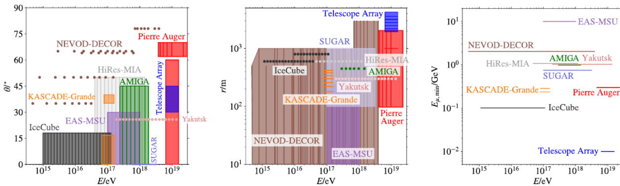
Figure 1.11: Air shower experiments have measured the muon density at ground under various conditions which are shown here as a function of the shower energy. Points and lines indicate a measurement in a narrow bin of the parameter, while boxes indicate integration over a parameter range. Left: Zenith angle of air showers. Middle: Lateral distance of the muon density measurement. Right: Energy threshold for the muons that are counted in the experiment. [80]
