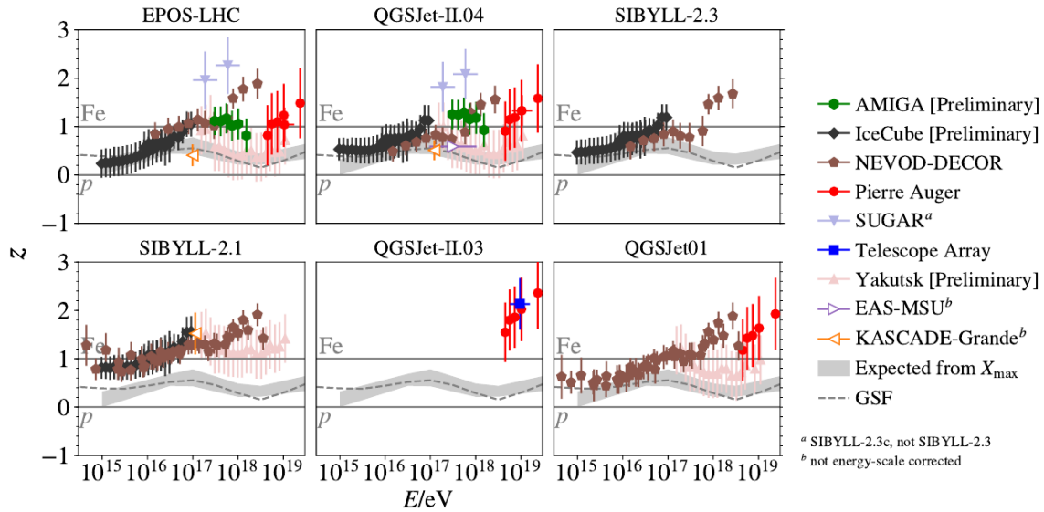
Figure 1.13: Muon density measurements converted to the z -scale. It depends on the hadronic interaction model, so the same data sets are repeatedly shown for different models. When corresponding simulations are missing for an experiment, no points can be shown. [80]
