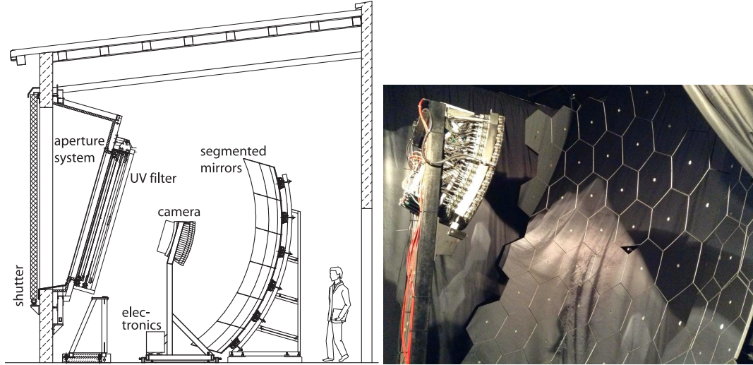
Figure 1.8: (Left) schematics of a fluorescence telescope at the Pierre Auger Observatory [45]. (Right) picture of the telescope mirror and camera.
