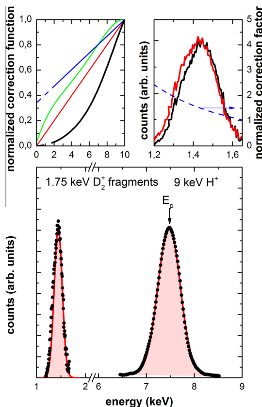
Fig. 1. Left upper panel: Energy dependence of the correction functions due to the analyzer transmission (red), the detector efficiency (blue), and the outgoing ion fraction (green); together with the total correction function (thick black). All of them were normalized to 1 at 10 keV for comparison. Right upper panel: Energy spectra of 1.75 D_2^+ fragments transmitted through a 15 nm Pt film. The Black line corresponds to the uncorrected spectrum, and the red one to the spectrum corrected by multiplying the uncorrected one by the normalized correction factor (dash blue). See text for correction factor definition. Lower panel: Energy spectra of 1.75 D_1^+ fragments and 9 keV protons transmitted through a 15 nm Pt film (black solid circles). Red solid line and light red area correspond to function shape and area of gaussian fit. (For interpretation of the references to color in this figure legend, the reader is referred to the web version of this article.)
