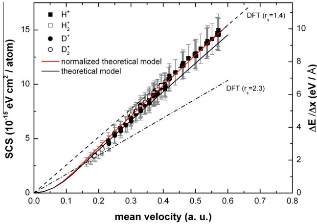
Fig. 8. Stopping cross section for hydrogen ions in Pt, as a function of the mean projectile velocity (lower scale). The scale on the right side shows the energy loss values \langle \frac{dE}{dx} \rangle . The solid and open squares and circles show the current measurements. The solid red line shows the SCS values obtained with the theoretical model of Eq. (5), normalized to the mean value of the highest experimental SCS data value. The solid black line correspond to the absolute values given by Eq. (5). The dash and dash-dot lines show the DFT calculations for a free-electron gas with r_s = 1.4 and r_s = 2.3 , respectively. (For interpretation of the references to color in this figure legend, the reader is referred to the web version of this article.)
