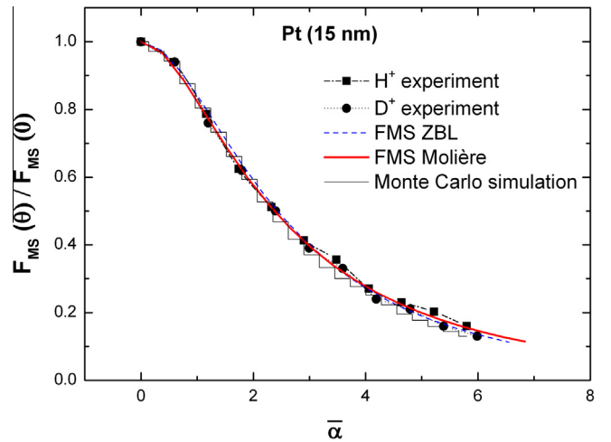
Fig. 4. Normalized angular distribution of 9 keV protons and deuterons transmitted through a thin film (15 nm) of Pt in terms of the reduced angle \alpha = (Ea/2Z_1Z_2e^2)\theta .
