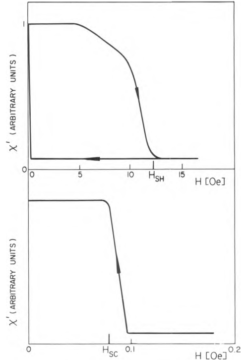
FIG. 2. Typical hysteresis loop (in the case for 50\text{-}\mu Cd spheres at t=0.95 ). The lower curve shows the supercooling transition with an expanded horizontal scale.
