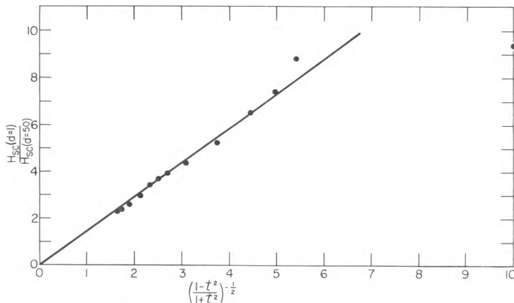
FIG. 10. Ratio of the supercooling field of the sample of 1 \mu to that of the 50- \mu sample as a function of (1+t^2)^{1/2}/(1-t^2)^{1/2} .
