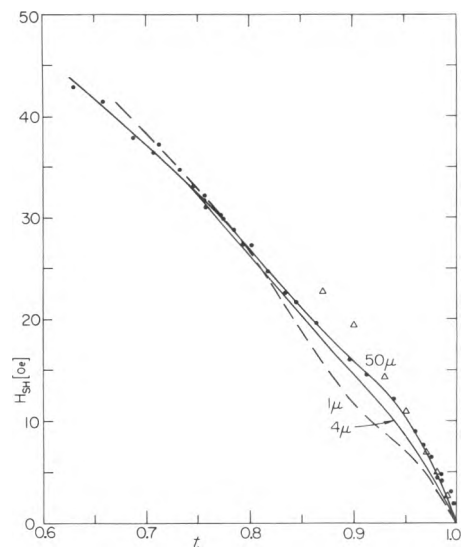
FIG. 4. Superheating field measured as a function of reduced temperature for Cd spheres of several sizes. The triangles are points calculated with Eq. (5) for C=1 .
