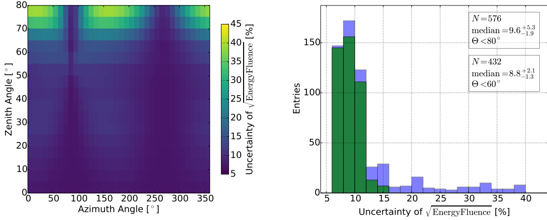
Figure 15. ( Left ) Systematic uncertainty of the square root of the energy fluence for all arrival directions taking into account a signal polarization due to the dominant geomagnetic emission process. The square root of the energy fluence is shown because the energy fluence scales quadratically with the electric-field amplitude and the cosmic-ray energy. Hence, the uncertainties of the square root of the energy fluence is the relevant uncertainty in most analyses. ( Right ) Histogram of the systematic uncertainty of the square root of the energy fluence of signals with zenith angles smaller than 80^\circ (blue) and of signals with zenith angles smaller than 60^\circ (green).
