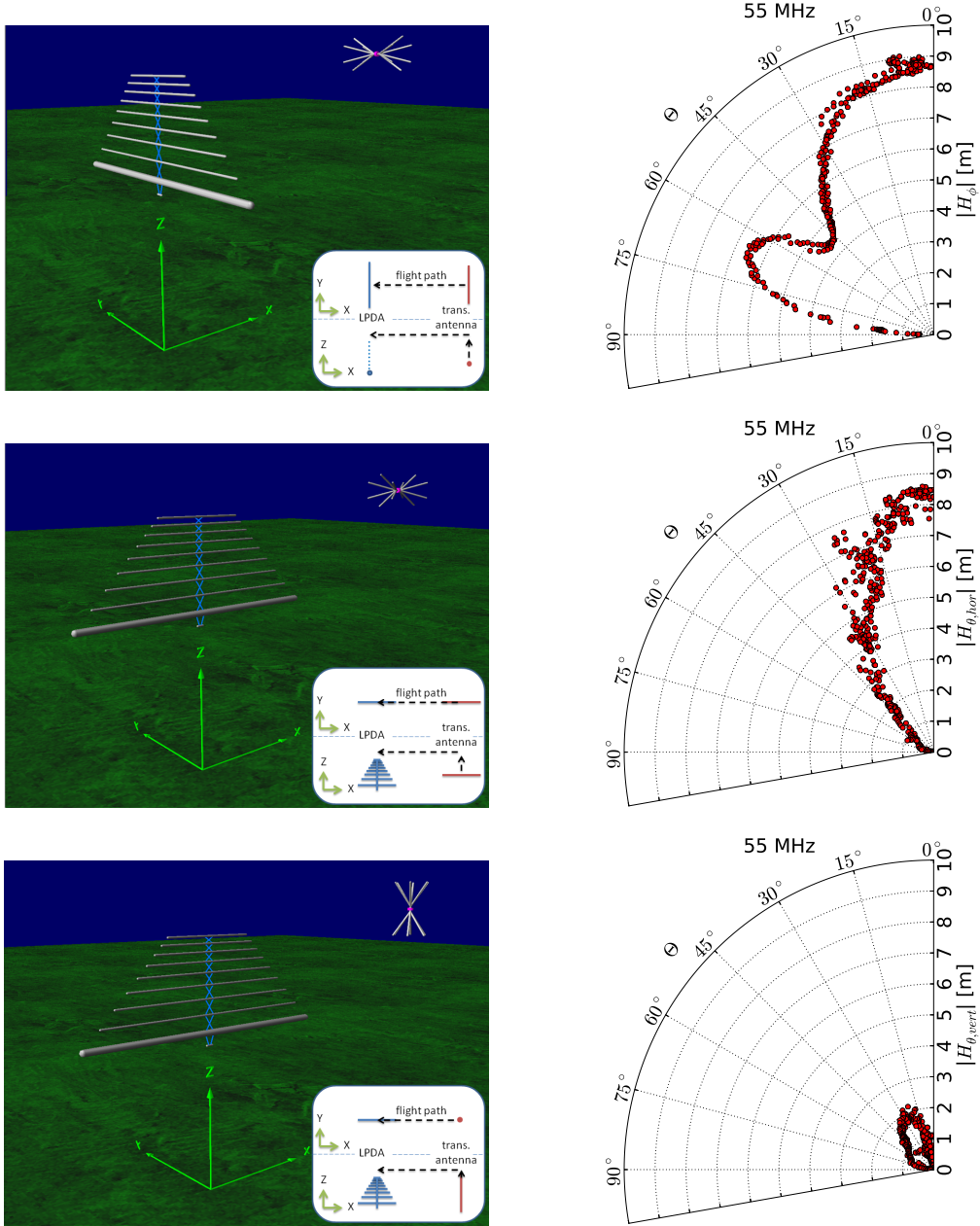
Figure 3. (Left) NEC-2 realization of the setup to simulate the three VEL components (from top to bottom) |H_\phi| , |H_{\theta,hor}| and |H_{\theta,vert}| . The meridional component |H_\theta| is a combination of |H_{\theta,hor}| and |H_{\theta,vert}| . The distance between transmitting and receiving antenna is reduced and the transmitting antenna is scaled by a factor of 3 to make both antennas visible. For clarity, the LPDA and the transmitting antenna (assumed as a simple dipole) orientations are sketched in the lower right corner of each picture in the XY-plane as well as in the XZ-plane. (Right) Measured VEL as function of the zenith angle (red dots) of three example flights for the three VEL components at 55 MHz.
