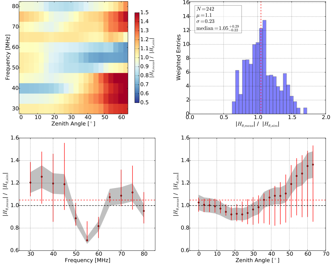
Figure 13. Comparison of the combined meridional VEL |H_\theta| with the simulation. ( Top left ) Ratio of combination of all measurements and simulation for all frequencies as a function of the zenith angle \Theta up to 63^\circ in 3^\circ bins. ( Top right ) Histogram of all ratios of the combination of all measurements and simulation for all frequencies and all zenith angle bins previously mentioned weighted with \sin(\Theta) . The median value is marked as the red dashed line. ( Bottom left ) Median (red dots) and the 68% quantile (red error bars) of the zenith angle weighted correction factor distribution as a function of the frequency. ( Bottom right ) Median (red dots) and the 68% quantile (red error bars) of the ratio distribution as a function of \Theta . The gray band indicates the constant systematic uncertainty of the measurement and the red dashed lines mark the overall zenith angle weighted average in both lower diagrams.
