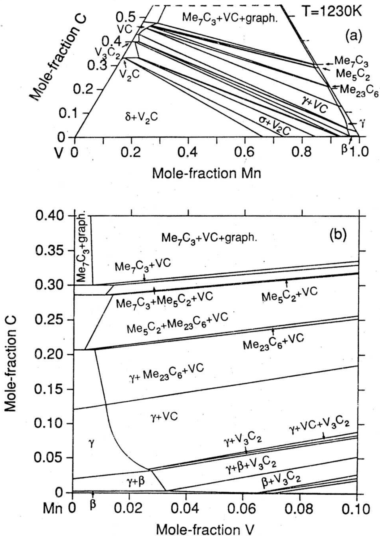
Fig.9 a) The isothermal section and b) an enlargement of the Mn-rich corner of the Mn-V-C phase diagram at 1230 K, calculated using the present thermodynamic description, see Table II.
