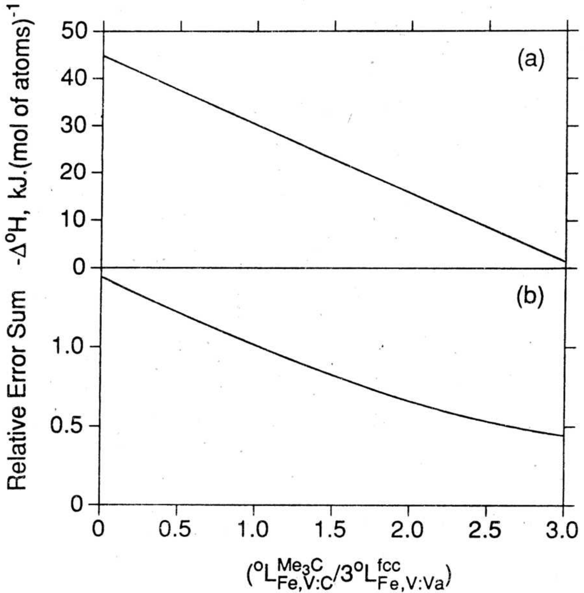
Fig.3 a)The "optimum" value of the negative enthalpy of formation of the metastable V_3C(oP16) carbide, defined in Sec.4.3.1 and b) the "relative" error sum (Sec.4.3.1) describing the goodness of fit to experimental data [37] on the distribution of V between fcc and the (Fe,V)_3C phase, for various choices of the phenomenological interaction parameter L_{Fe,V:C}^{Me_3C} . In these fits the interaction parameter L_{Fe,V:Va}^{fcc} was given the value assessed by Huang [35].
