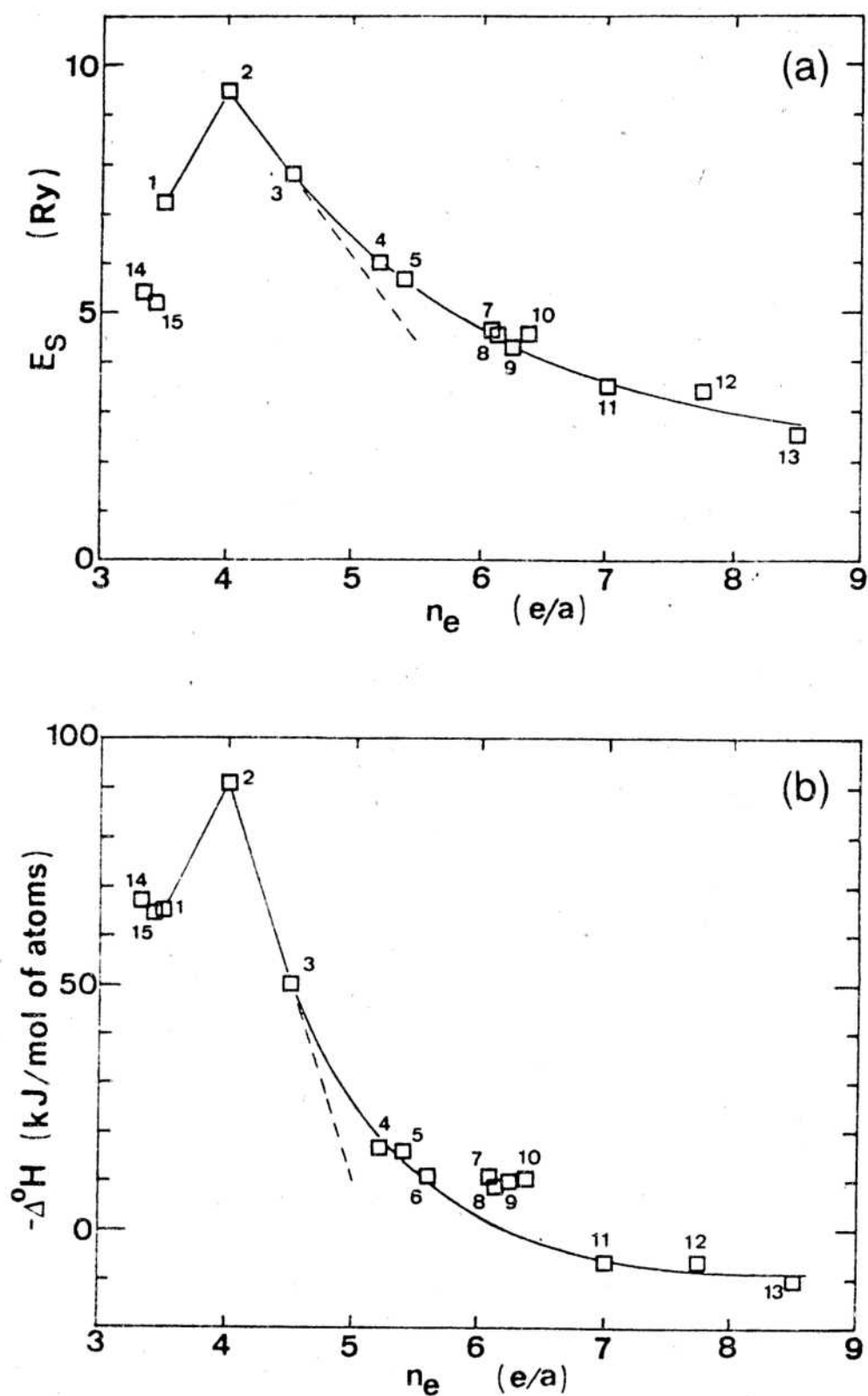
Fig.1 a) The energy-related characteristic energy E_S , defined in eq.(17), and b) The negative enthalpy of formation of carbides at 298.15 K ( -\Delta^\circ H ), as a function of the average number of valence electrons per atom, n_e . The numbers refer to ScC(1), TiC(2), VC(3), \text{Cr}_3\text{C}_2 (4), \text{Cr}_7\text{C}_3 (5), \text{Cr}_{23}\text{C}_6 (6), \text{Mn}_7\text{C}_3 (7), \text{Mn}_5\text{C}_2 (8), \text{Mn}_3\text{C} (9), \text{Mn}_{23}\text{C}_6 (10), \text{Fe}_3\text{C} (11), \text{Co}_3\text{C} (12), \text{Ni}_3\text{C} (13), \text{Sc}_2\text{C} (14), and \text{Sc}_4\text{C}_3 (15). The dashed lined refer to the (cF8) NaCl-structure. From Fernández Guillermet and Grimvall [5].
