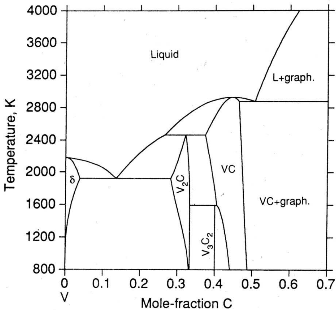
Fig.6 The V-C phase diagram calculated using the thermodynamic description assessed by Huang [10], used as a basis for the present work.
