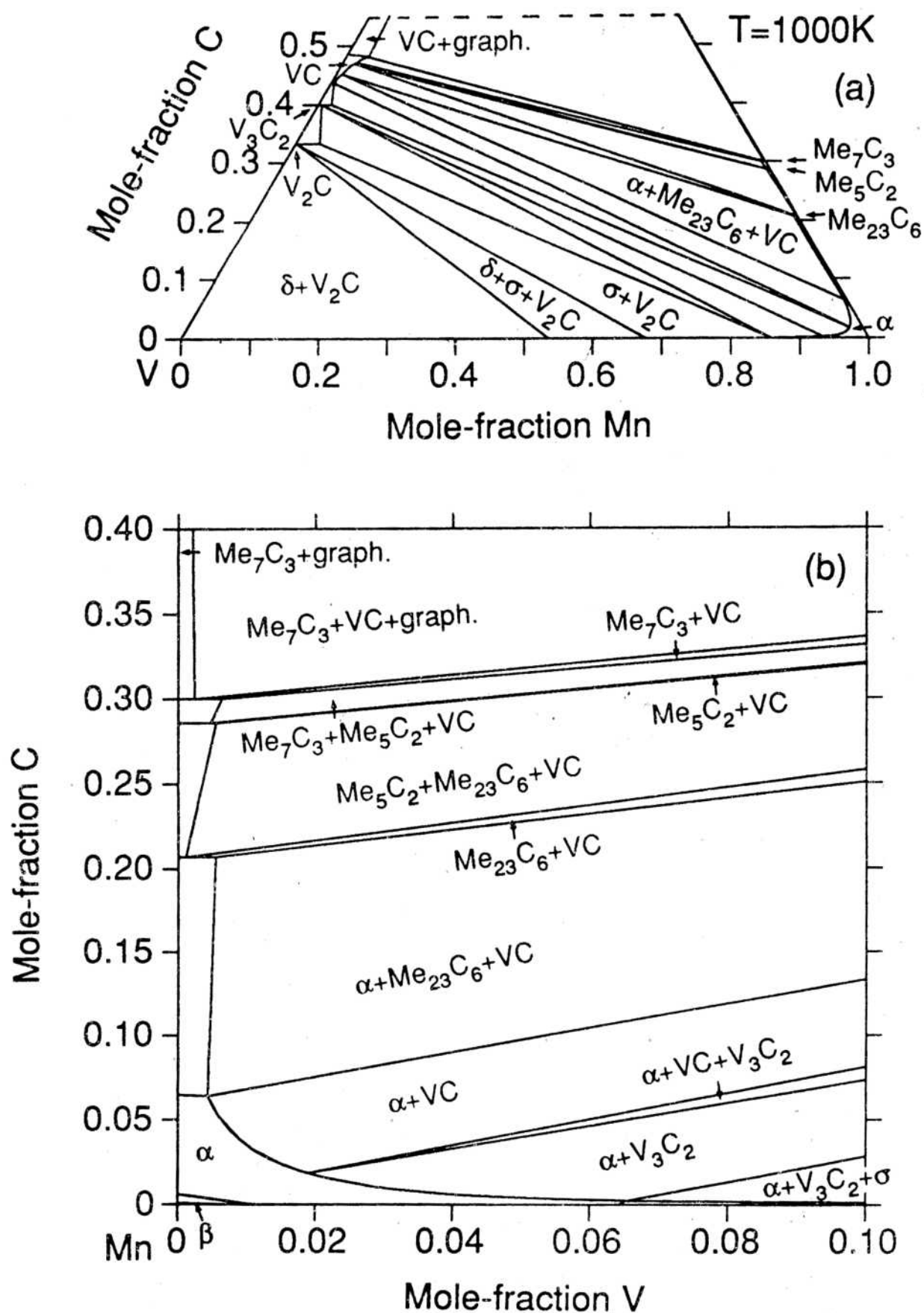
Fig.8 a) The isothermal section and b) an enlargement of the Mn-rich corner of the Mn-V-C phase diagram at 1000 K, calculated using the present thermodynamic description, see Table II.
