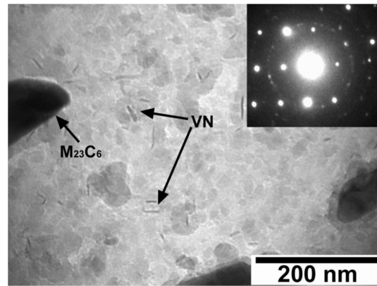
FIG. 4. TEM micrograph of the BM. The inset shows a ring pattern that corresponds to fine VN precipitates and a spot pattern that correspond to the indicated M_{23}C_6 carbide.
