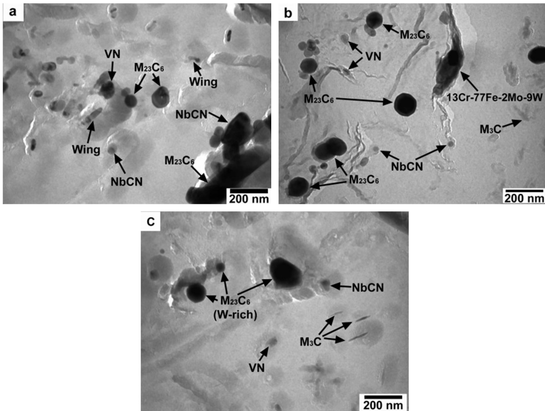
FIG. 7. TEM micrographs of the FGHAZ: a) near ICHAZ, b) intermediate ICHAZ and c) near CGHAZ.
