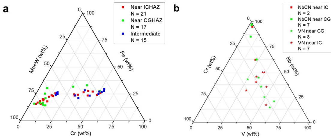
FIG. 8. Ternary composition diagrams of M_{23}C_6 (a) and MX (b) precipitates in the FGHAZ. N = number of particles.
