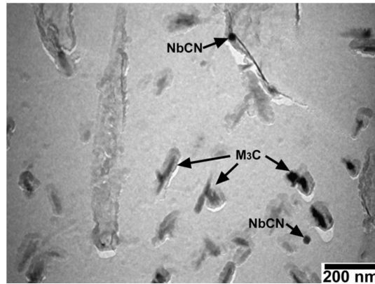
FIG. 9. TEM micrograph of the CGHAZ.
