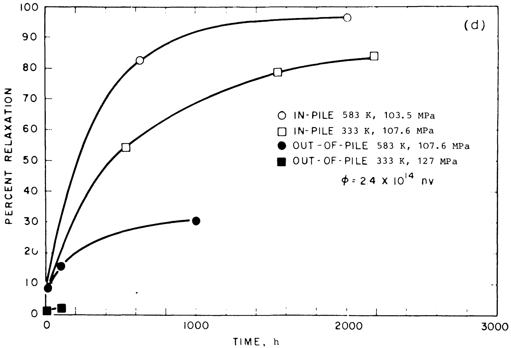
Fig. 16d: Relaxation of 79% cold-worked Zircaloy-4. Data taken from Ref. [20].
