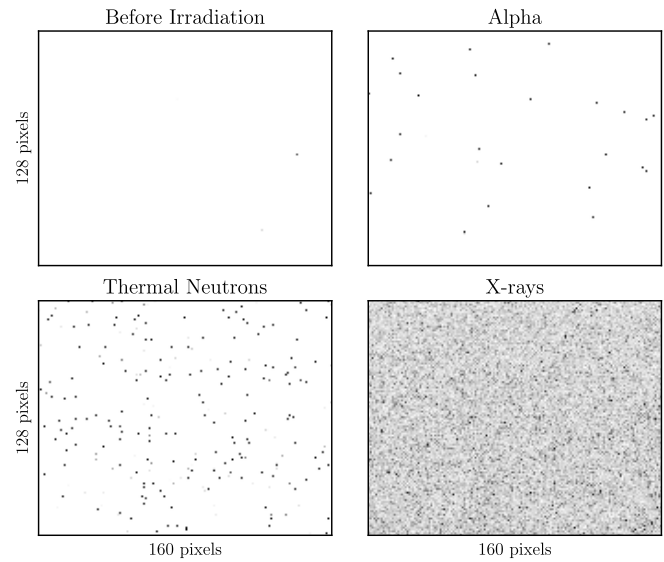
Fig. 2. Comparison of dark output images before and after irradiation. 1/8th of the original images are shown, and also, the color scheme was reversed for clarity, so darker colors correspond to brighter pixels. Alpha particles and thermal neutrons produce defects that are localized, while X-ray photons increase the overall leakage. Alpha particles fluence was 1.6 \times 10^6 \text{ cm}^{-2} , thermal neutron fluence was 2.23 \times 10^9 \text{ cm}^{-2} , and X-ray photon fluence was 1.8 \times 10^{13} \text{ cm}^{-2} [54 Gy(Si)].
