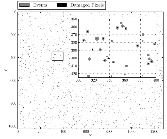
Fig. 6. Events and damaged pixels detected by processing the neutron radiography experiment video with the algorithm. A time span of 30 min of irradiation was analyzed, and the events detected were accumulated to form the presented image. Only a fraction of the image area is shown.
