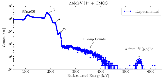
Fig. 7. RBS experimental results. The 5.6-MeV peak indicates that the sample contains boron.
