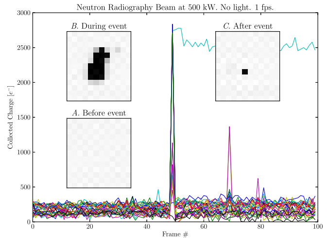
Fig. 4. Typical damage produced during the neutron radiography experiment. The values of a matrix centered on the event are shown versus time (at 1 frames/s, t_{\text{int}} = 1033 ms) and also the image sequence as seen in the video. Inset A: pixels before particle hit. Inset B: frame in which interaction took place. Inset C: resulting damage. In frames 69 and around 80, other particles are detected without creating a permanent defect.
