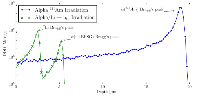
Fig. 8. DDD as a function of depth calculated from SRIM simulations. Zero depth is the Si–SiO 2 interface, and the x-axis points toward the silicon substrate (marked in Fig. 1). The simulation takes into account 1.47-MeV alphas and 0.84-MeV 7 Li, which are the most probable particle energies after boron neutron capture. The remaining 6% of the cases were disregarded.
