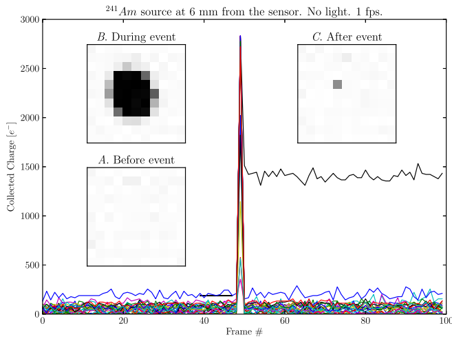
Fig. 3. Typical damage produced by alpha particles. 36 pixel values of a 6 \times 6 matrix centered on the event are shown as a function of time (at 1 frames/s, t_{\text{int}} = 1033 ms). Inset A: image before particle hit. Inset B: frame in which the interaction took place. Inset C: resulting image after damage.
