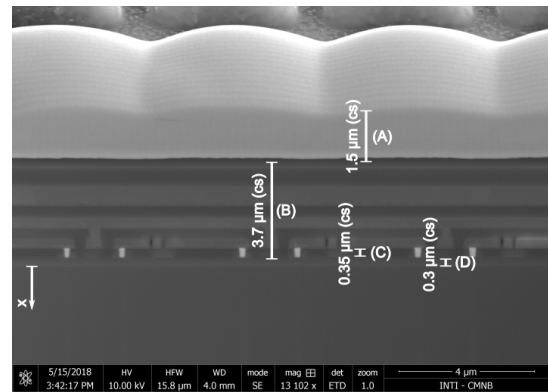
Fig. 1. SEM image of the cross section of the integrated circuit. (A) Microlenses. (B) BEOL. (C) Premetal dielectric. (D) FOX.
