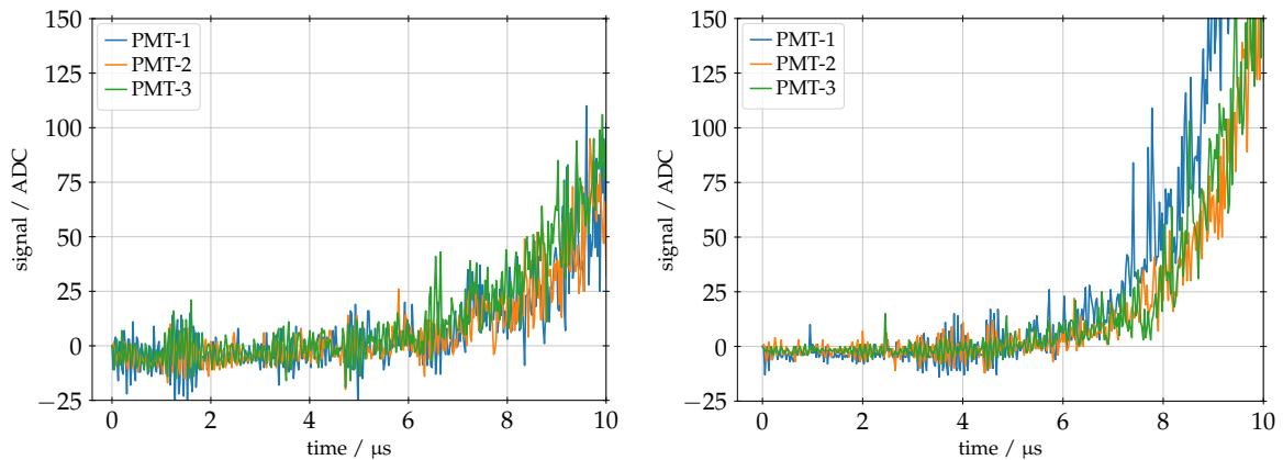
Figure 5.24: Zoom into the start of the two signals from Fig. 5.23. Differences in the rise time and the level of lightning noise are clearly visible. Left: Trace from station 1521 of event 42852075, \Delta Baseline = 5.6 ADC. Right: Trace from station 1110 of event 4067414, \Delta Baseline = 5.8 ADC.
