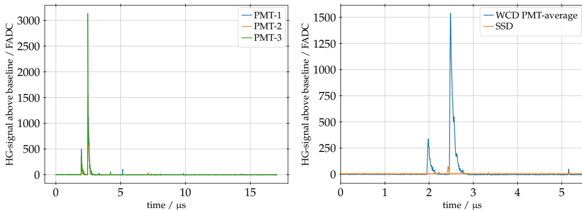
Figure 5.40: Example of a trace from the sample of 1000000 random UUB traces. It is trace number 446595 and it was selected using a simplified ToT-trigger with modified parameters. Left: Complete traces of the WCD PMTs. Right: The average of the large PMTs of the WCD- and the SSD-trace zoomed into the signal part of the trace.
