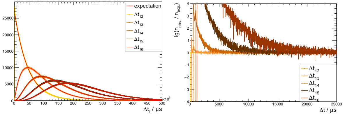
Figure 5.4: Left: Time differences between a trigger and the i^{\text{th}} next trigger per station summed over all stations. It is displayed for i = 2, \dots, 6 . The expectation is computed using Eq. (5.1). Right: Zoom into the first 25 ms of the same data. The logarithm of the ratio of the observed data to the expected is used to display all orders on a similar scale.
