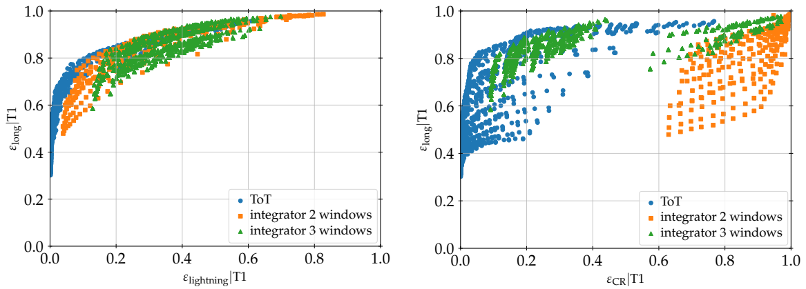
Figure 5.42: Efficiencies of different algorithmic approaches for a potential T1 and different parameter settings. The test-sample consists of UB-signals because of the lack of UUB signals. The choice of UB signals implies that all efficiencies are conditional on having triggered with one of the existing triggers. Left: Detection efficiency of (already triggered) long signals as a function of lightning background rejection, in this case the efficiency of tagging lightning signals. Right: To highlight the properties of the algorithms and settings, the efficiency of the algorithm as a function of the efficiency of finding cosmic-ray signals.
