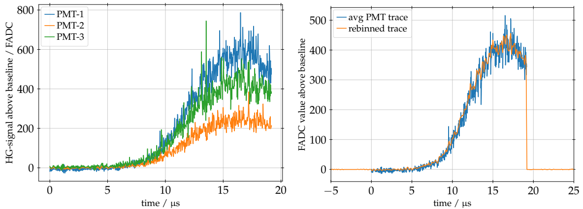
Figure 5.44: Example trace to illustrate the concept of rebinning traces. Data from station 878 of event 1332968 is shown as case of a long-signal trace that extends beyond the time range covered by the trace. Left: Signals of the individual PMTs in raw FADC. Right: Average signal in blue and the rebinned trace averaging 4 bins into one.
