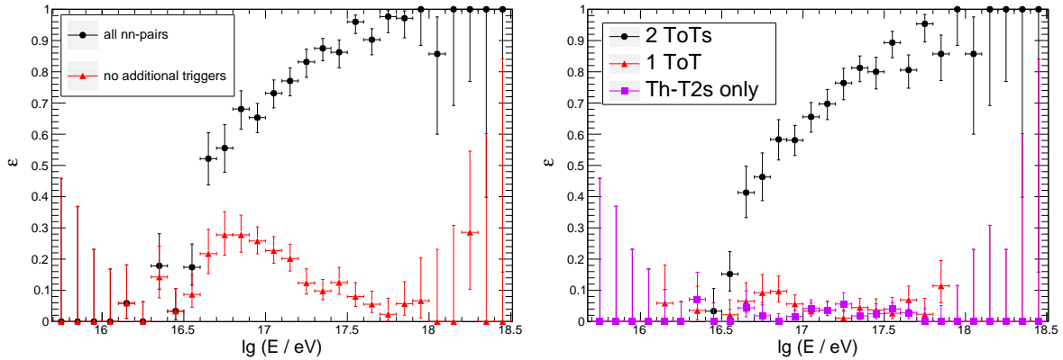
Figure 5.48: Sensitivity of pairs of T2-triggers in nearest neighbour stations in the infilled SD-750 array. Left: Total efficiency (black) as determined with hybrid events [125, 126] with reduced quality cuts to move the energy threshold down. The red dots indicate the efficiency if in addition to the condition of two neighbouring triggers within 4\ \mu\text{s} no additional triggers, i.e. no triplet of triggers, are allowed. Deviations from full efficiency at highest energies are due to reduced quality cuts and missing cuts on non-working stations. Right: Details of the trigger types contributing to the detected events. Out of the two triggers forming the nearest-neighbour pair, none, one, and two are requested to be a ToT for the purple, red, and black points. It is very clear that the vast majority of events is detected with two ToT triggers.
