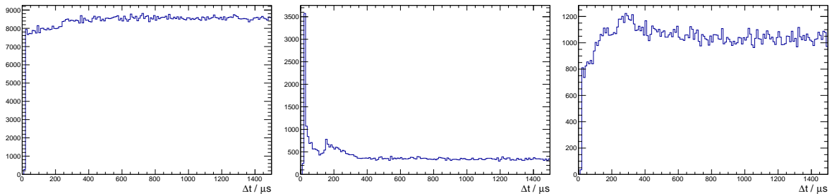
Figure 6.6: Left: Time differences between “old” ToTs only: the spectrum is very regular. Middle: Time differences using only ToTd triggers. The combination of ToTd and MoPS is not included. A clear peak after the veto period of 20 \mu\text{s} is visible. Right: The same distribution for MoPS triggers only. Also here triggers that have both MoPS and ToTd are not used.
