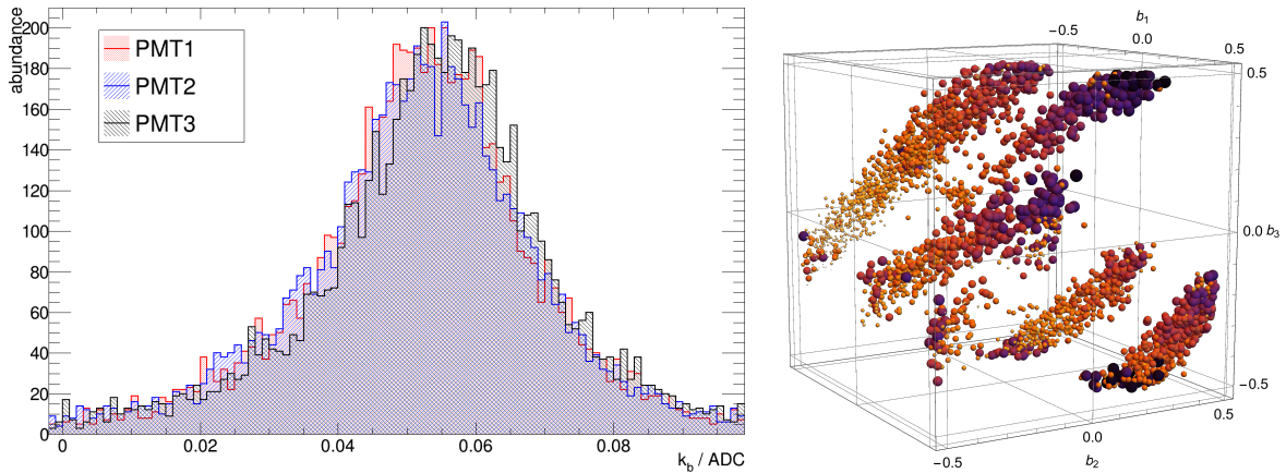
Figure 4.13: Left: Fitted coefficients for baseline mantissas for all stations separated by PMT-number in April 2012. Right: Visualisation of the dependence of the scaler rate on the baseline mantissas. The colour and the size of the markers indicates the scaler rate measured in a 61 s interval while the b_i are defined as b_i = \text{baseline}_i - \text{round}(\text{baseline}_i) . 3D-Visualisation by D. Vebrič.
