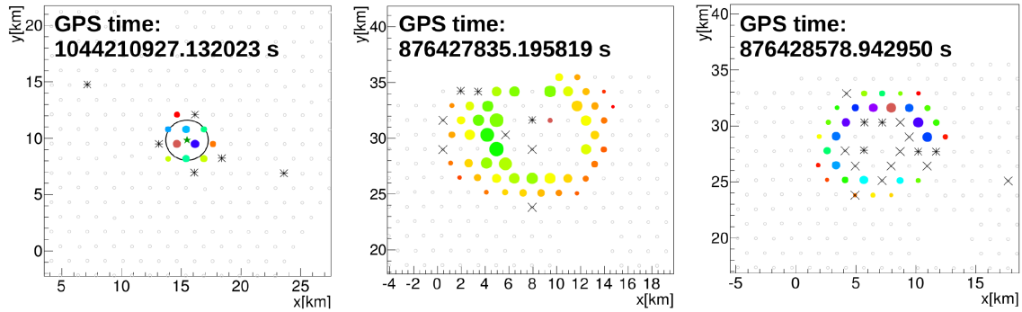
Figure 5.2: Footprints of exemplary peculiar events observed in the SD. Circles mark stations with “long-signals” (c.f. Fig. 5.1 e, f) with the size corresponding to the signal size and the colour representing time (blue early, to late in red). So called lightning stations are marked with stars and muon/cosmic-ray stations with crosses. A ring-like shape for these events is evident, leading to the naming “SD-ring”. For smaller events, the ring is filled creating “SD-disks”. Figure taken from Ref. [10].
