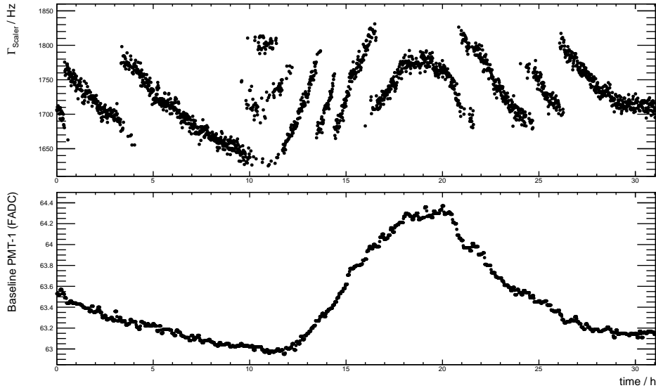
Figure 4.11: Upper panel: Scaler rate of station 751 for a day in April 2012 averaged in 61 s intervals. The intervals corresponds to the station’s calibration intervals. Lower panel: Baseline of PMT-1 in the same period showing the characteristic drift with temperature over the day.
