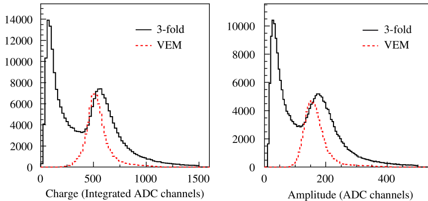
Figure 3.8: Histograms of charge and amplitude (summed over the PMTs) of a station taken with a 3-fold coincidence trigger at 5 FADC-channel threshold. The first peak comes from low-energy particles convolved with the trigger response, while the second one comes from through-going atmospheric muons. With the help of a muon telescope central, vertical through-going muons are selected and shown in red. Taken from Ref. [72].
