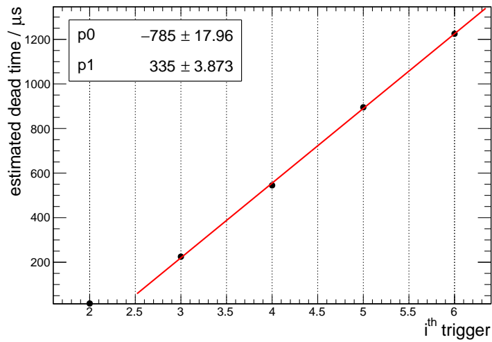
Figure 5.5: Illustration of the amount of dead time as a number of consecutive triggers. The numbers are estimated from the histograms of Fig. 5.4. A linear fit, excluding the lowest order, is performed and the parameters are given in the parameter panel.
