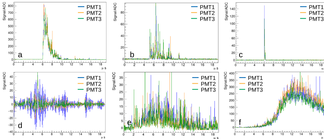
Figure 5.1: Illustration of typical signals in the surface detectors: a-c are signals from cosmic-ray showers at different distances to the core. d is a typical example trace caused by RF-noise picked up in the PMT-cables during lightning activity. e, f show examples of the so called “long-signals” rarely observed during thunderstorms that are due to signals in the detectors rather than pick-up in the cables. The two examples differ in amplitude but are thought to be originating from the same type of events. Taken from Ref. [104].
