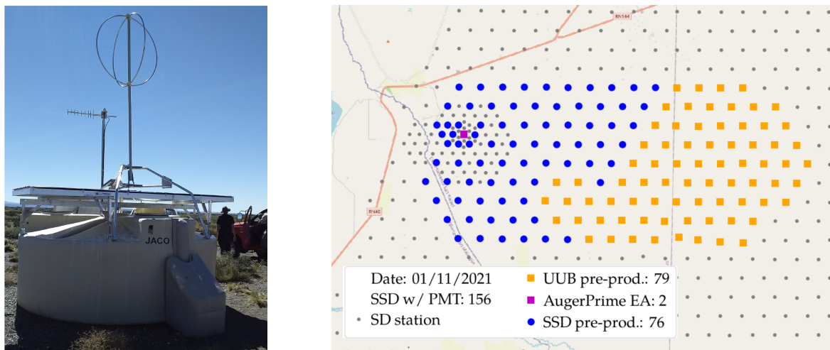
Figure 3.10: Components of the upgrade of the Pierre Auger Observatory (AugerPrime). Left: Photograph of a upgraded stations with Scintillator and radio antenna. Taken from Ref. [78]. Right: Deployment map of the upgraded components in the field. Kindly provided by A. Streich.
