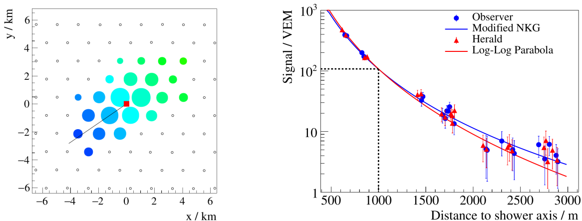
Figure 3.9: Illustrations for the event reconstruction with the Auger SD. Figures taken from Ref. [73]. Left: Footprint of stations of an event coloured by arrival time (blue early, green late). The projection of the reconstructed shower axis ending in the shower core is shown as black line. Right: Lateral distribution of signals in a shower. The fits correspond to two different approaches for the reconstruction and the functional form. For details see Ref. [73].
