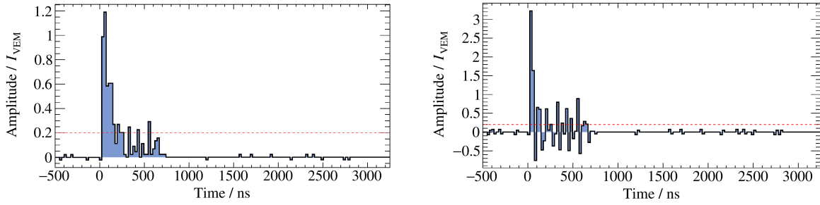
Figure 3.6: Illustration of the deconvolved ToT (ToTd). Taken from Ref. [68]. Left: Trace triggered by a ToTd. Right: Deconvolved trace of the same event used to form the ToTd trigger.
