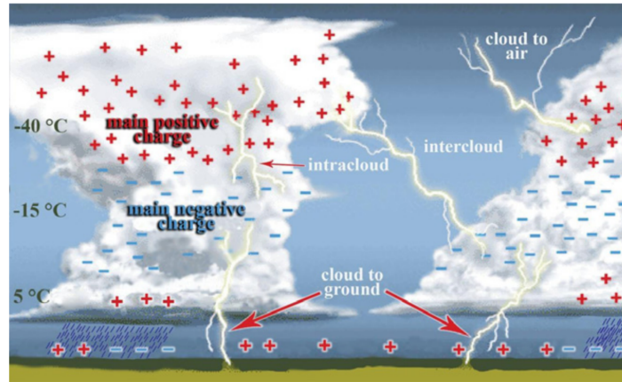
Figure 2.7: Schematic of thunderclouds with typical charge layers formed by friction of hail and graupel. Common names for the different kinds of lightning are given. Taken from Ref. [7].
