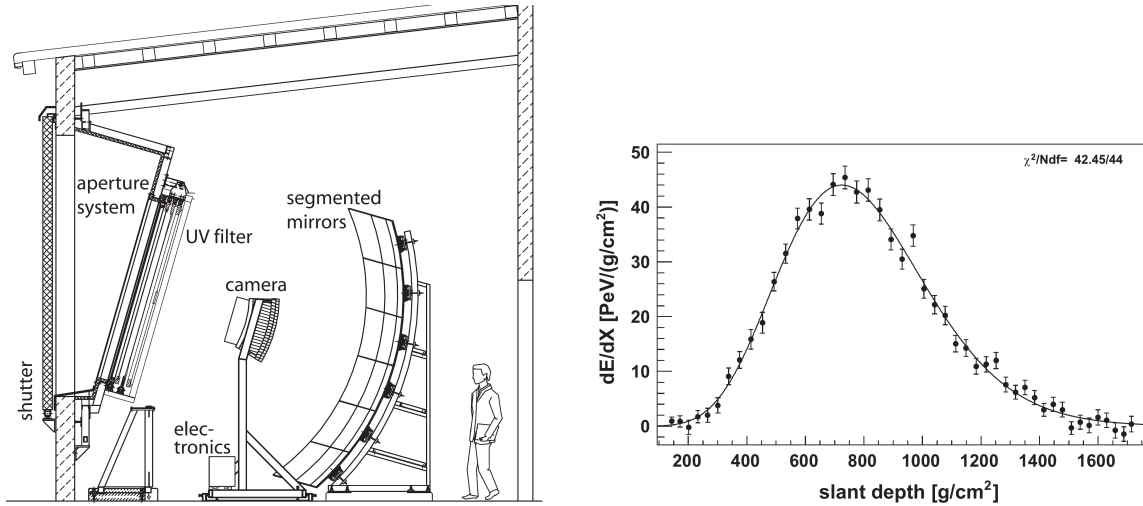
Figure 3.2: Schematics of the fluorescence detector and the associated reconstruction. Figures taken from [1]. Left: Schematics of the telescopes. Right: Example reconstructed shower profile in terms of energy deposit.
