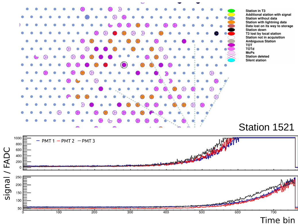
Figure 5.6: Display of the triggered stations of event 42852075. A hole in the middle of the event indicating the “ring” structure is visible. Also in subsequent events within the same GPS second no data from those stations are recorded. Example traces of the three PMTs of station 1521 are given in the lower panel. Both high-gain (upper panel) and low-gain (lower panel) channels show the same behaviour in all three PMTs of a very large and long-lasting signal.
