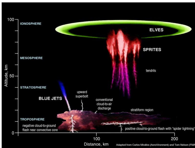
Figure 2.10: Illustration of different Transient Luminous Events (TLE). These are electric events caused by thunderstorms that are visible in different wavelengths. Taken from Ref. [61].
