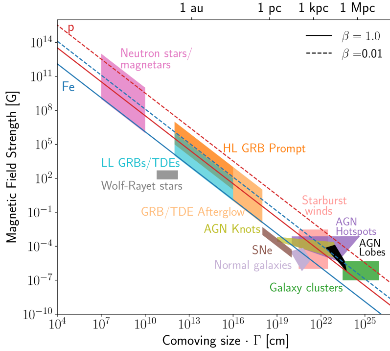
Figure 2.3: Hillas plot showing the sizes and average magnetic field strengths of classes of objects. The Hillas condition [34] (c.f. Eq. (2.7)) is a necessary condition for acceleration of cosmic-rays and is visualised in this diagram. Taken from Ref. [16]
