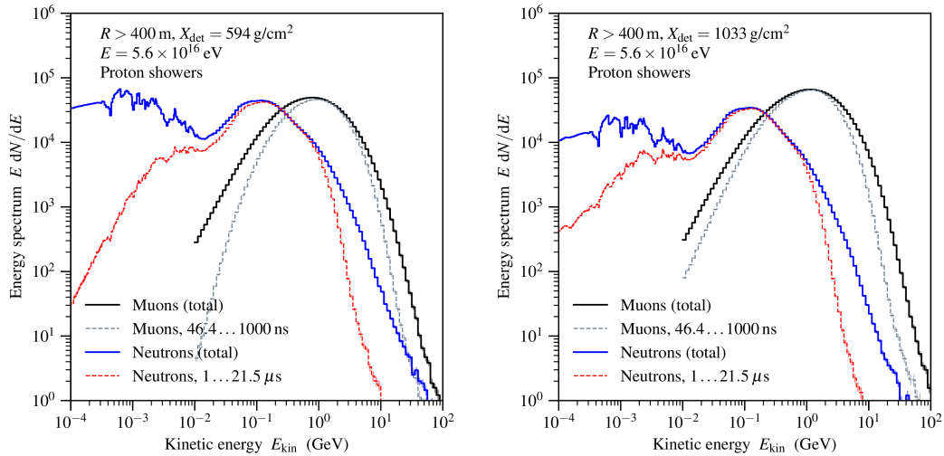
Figure 6.8: Neutron and muon spectra simulated with FLUKA for two observation depths X_{\text{det}} at large distances R from the core. The main time scales contributing to the spectra are highlighted in colour. Taken from Ref. [140].
