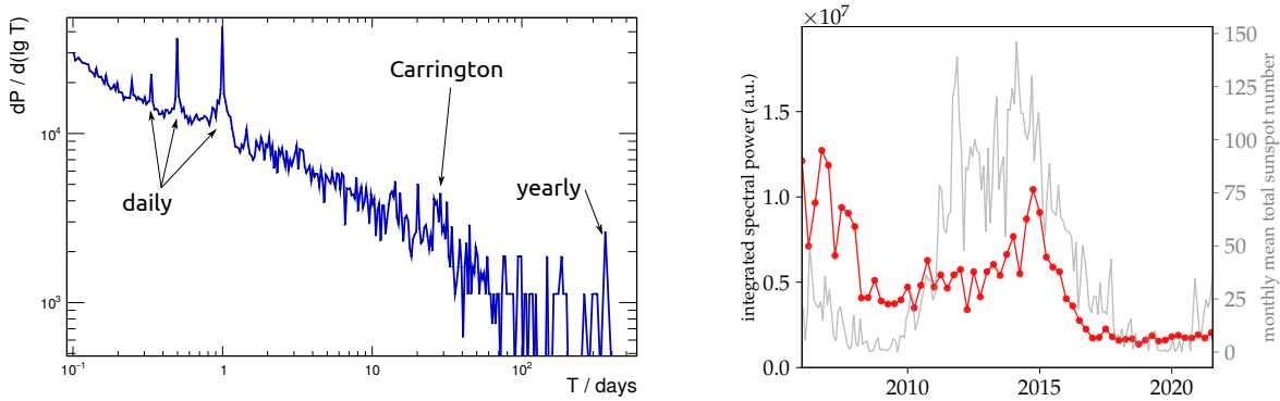
Figure 4.16: Left: Observed frequency spectrum of the data with annotations of frequencies of special interest. Right: Time dependence of the integrated spectral power around the Carrington frequency T \in [20, 70] days including overtones. For reference, the solar sunspot-number data from Ref. [98] is shown in gray.
