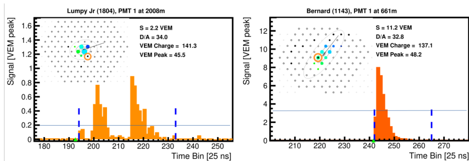
Figure 3.5: Illustration of the two main trigger modes of the SD. Left: ToT-triggered trace of station 1804 (PMT 1) from the event shown in the inset. The threshold of 0.2 I_{VEM, peak} is illustrated as line. Right: Threshold triggered station in an inclined event with larger total signal but smaller time dispersion.
