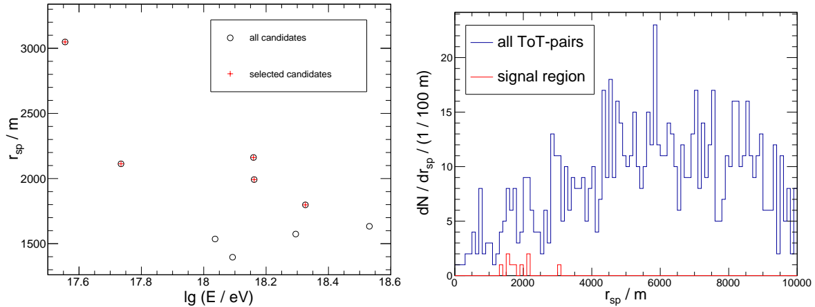
Figure 6.34: Characteristics of the observed event candidates. Left: Correlation of the distance in shower plane r_{\text{sp}} with the energy of the reconstructed event. The candidates left after visual selection are marked with red crosses. Right: Distribution of r_{\text{sp}} in the full extracted set of nearest-neighbour pairs of ToTs for all time differences within 10 ms. The signal region is concentrated on short scales, independent of the used cut r_{\text{sp}} < 5000 m.
