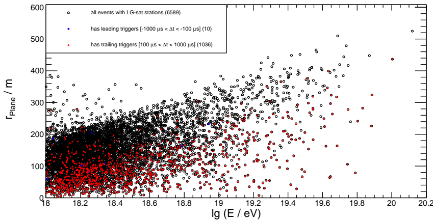
Figure 6.14: Distribution of the distance to the core and shower energy of stations with low-gain saturation. Stations that show delayed triggers are marked in red. They cluster at high energies and closer to the shower core. Blue marked stations with a (random) leading trigger are very rare.
