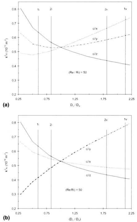
Fig. 2. (a) Fictitious sink strengths of a crack tip ( k_{IT}^2 ), and (b) crack surfaces ( k_{IS}^2 ), as a function of the defect diffusivity ratio D_c/D_a , for three different crystal orientations and R_c/R_i = 50 (from [17]). D_c/D_a predicted by a repulsive pair potential for vacancies (v) and interstitials (i) in \alpha -Zr at 560 K are shown; labels 1 and 2 correspond to strain free crystal lattice and to the homogenous strained crystal lattice ( \epsilon = 0.3 \times 10^{-3} ), respectively.
