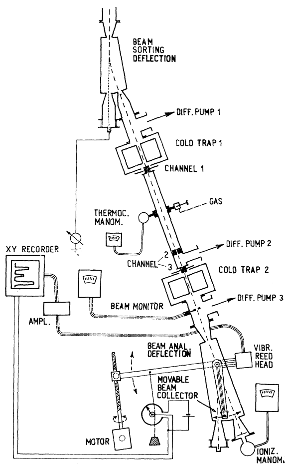
FIG. 1. Schematic diagram of the experimental equipment.
