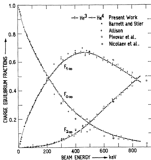
FIG. 4. Charge-equilibrium fractions F_{0\infty} , F_{1\infty} , and F_{2\infty} of He ions in He gas between 60 and 840 keV. Measurements made with the (He^3)^{++} beam are plotted at \frac{1}{3} of their actual energy.
