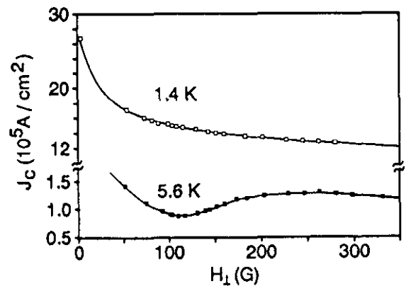
Fig. 3 : Comparison between high and low temperature behavior
