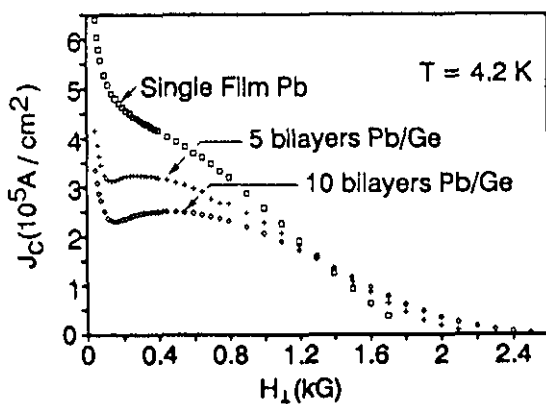
Fig. 1 : J_c(H_{\perp}) for a single Pb film and two [Ge/Pb] multilayers
