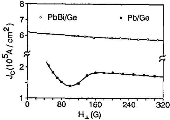
Fig. 4 : Effect of pinning strength on J_c(H_\perp)
