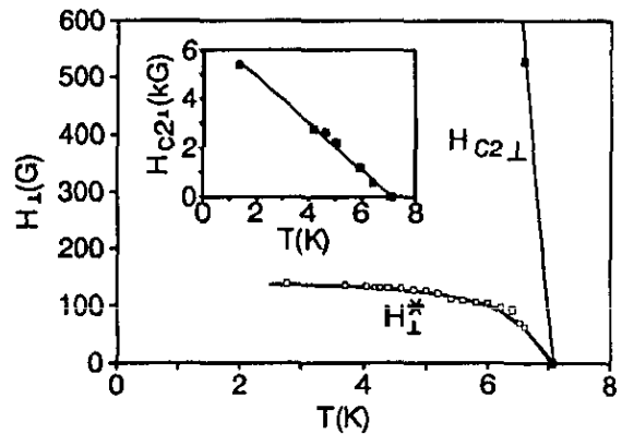
Fig. 5 : The H-T phase diagram. The inset shows H_{c2\perp}(T)
