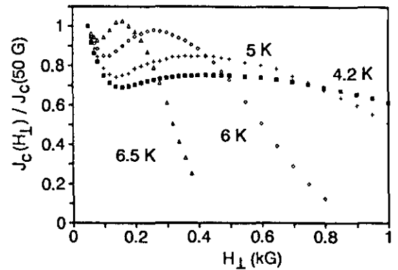
Fig. 2 : J_c(H_{\perp}) for a multilayer at various temperatures
