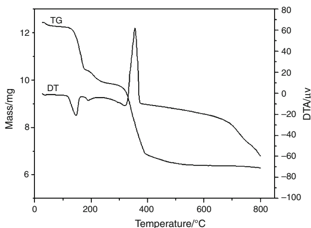
Fig. 1 TG and DTA curves for Y[Fe(CN) 6 ] \cdot 4H 2 O in air
