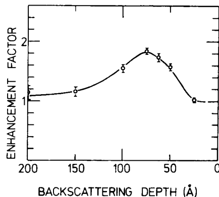
FIG. 2. Enhancement factor F(\theta) averaged over \theta < 0.2^\circ , as a function of backscattering depth, and for 1-MeV He on Pt. Bars represent standard deviations in the simulations.
