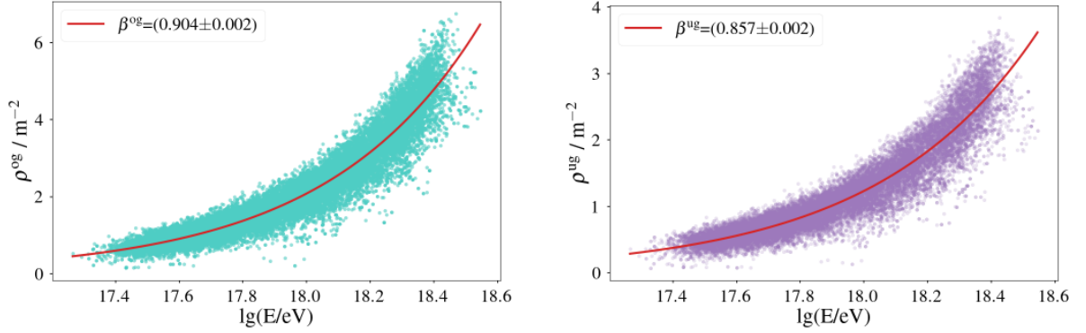
Figure 5.5: Power-law regressions of \rho^{0g} (left) and \rho^{ug} (right) versus primary energy with Monte Carlo values.
