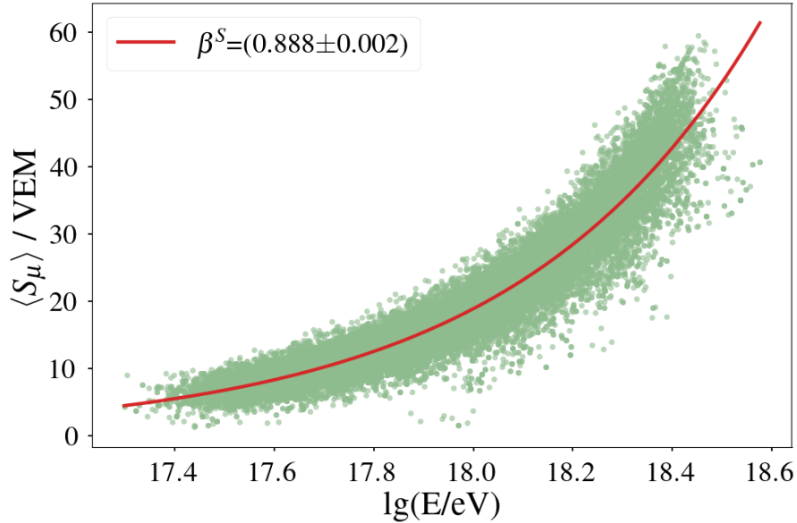
Figure 6.1: S_\mu dependence on primary energy.
