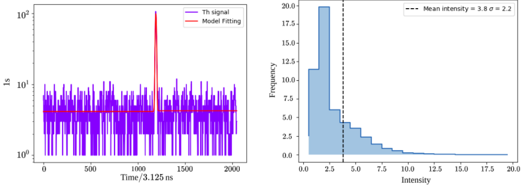
Figure 8.9: Left: histogram of ones per bin showing a Threshold trigger peak near the expected value of 1200. Right: histogram of intensities showing a lower-than-expected mean value of 3.8. Data correspond to December 2020.
