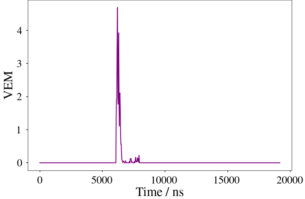
Figure 3.3: Example of a single muon trace in VEM units at 450 m from the shower core.
