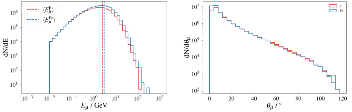
Figure A.5: Energy and zenith distributions for muons on-ground for 30° showers with an energy of 10^{18} eV
