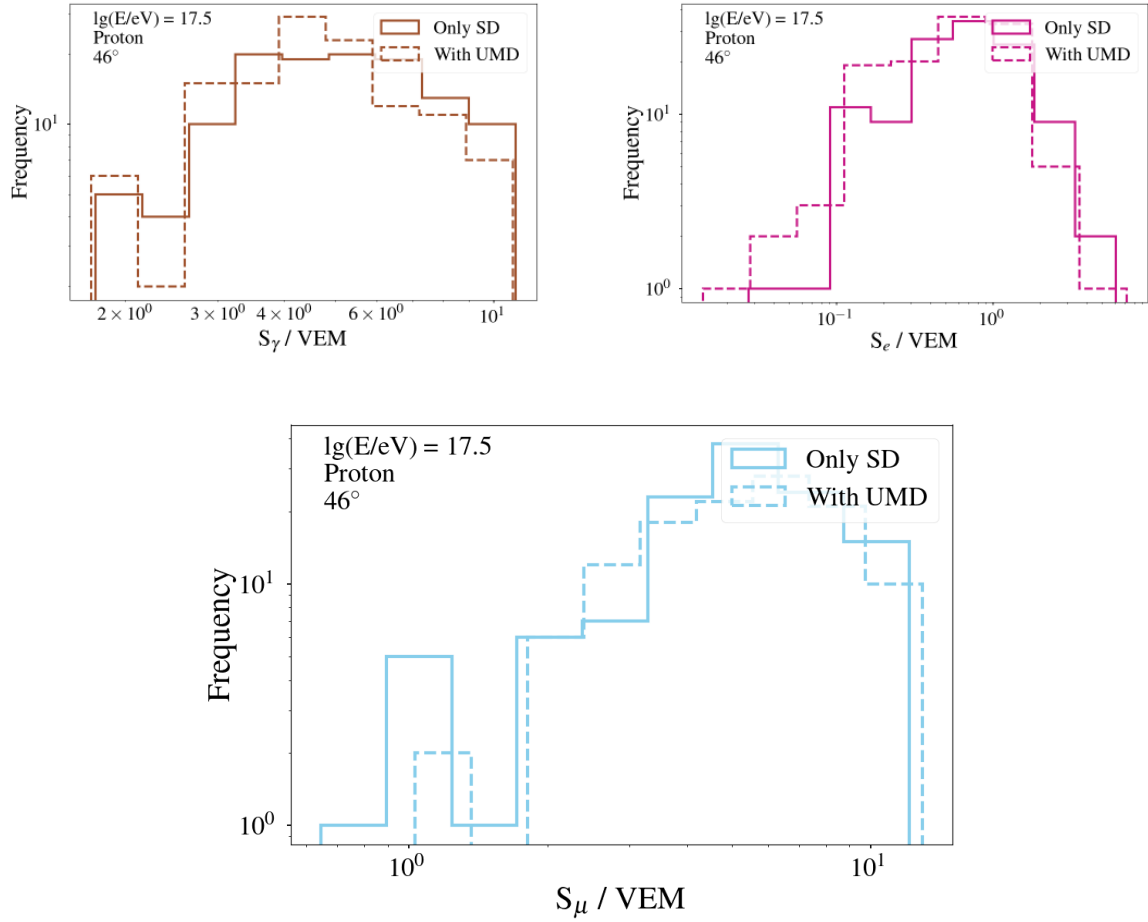
Figure C.2: Integrated WCD signals (photons, electrons, muons).
