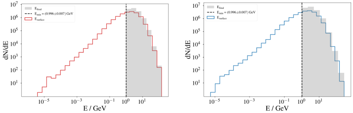
Figure A.6: Energy distributions of muons underground for 30° showers with an energy of 10^{18} eV compared to their original energy before trespassing the soil.
