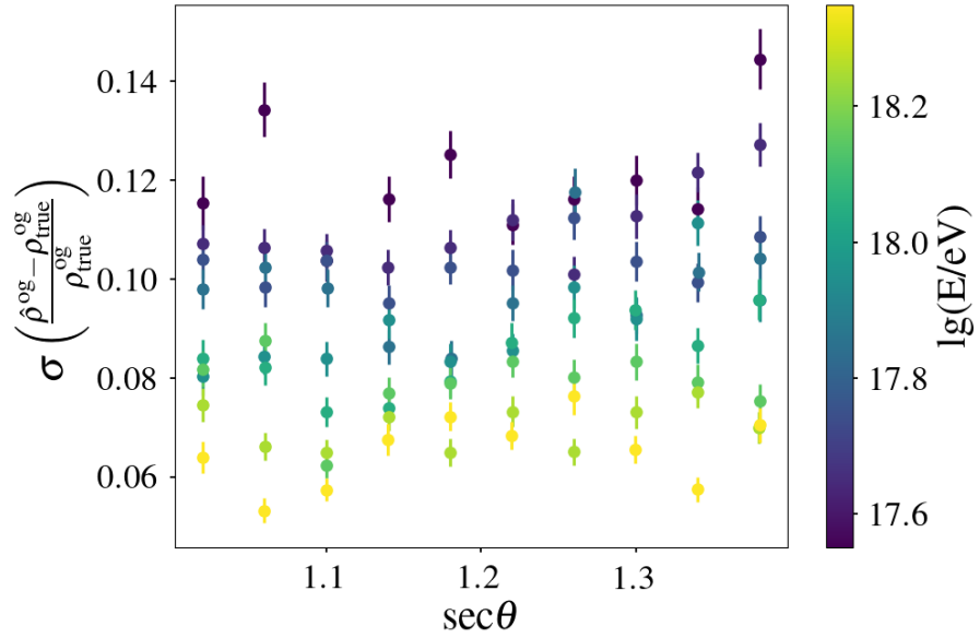
Figure 5.12: Resolution of the estimated muon density across the full energy and \sec(\theta) range.
