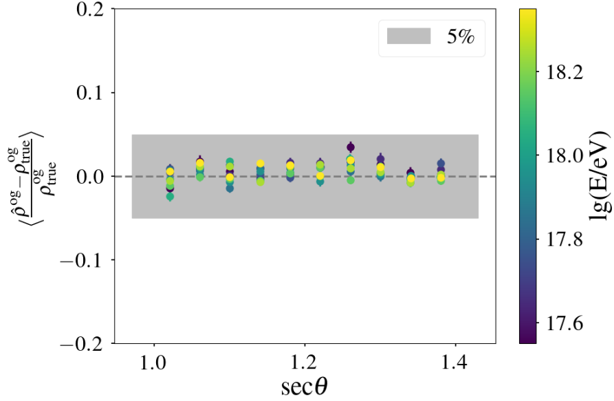
Figure 5.10: Bias across the full energy and \sec(\theta) range, computed as the mean residual in each bin.
