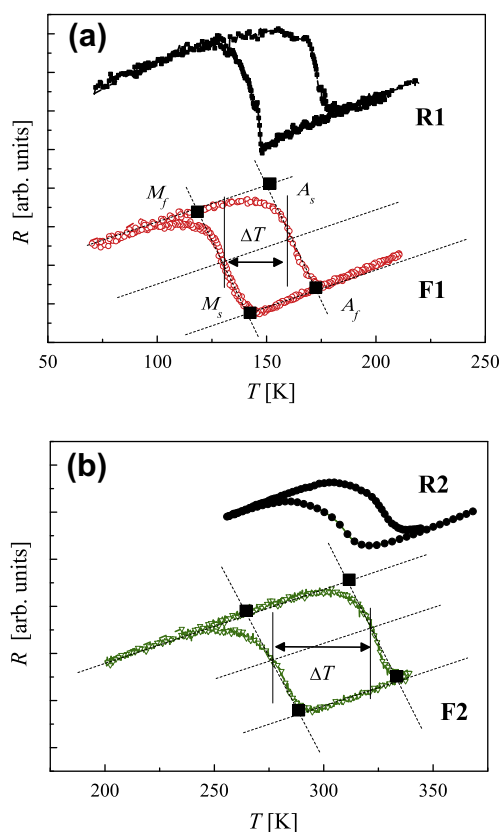
Fig. 1. Resistance vs. temperature in the reference R1 and in the films F1 and F2. The method for defining the parameters of the martensitic transformation was included. The hysteresis is measured as \Delta T . On cooling, the transformation temperature is set to start at M_s and to go to completion at M_f . On heating, the retransformation is set to start at the A_s temperature and finish at A_f . The resistance was rescaled for a clearer presentation.
