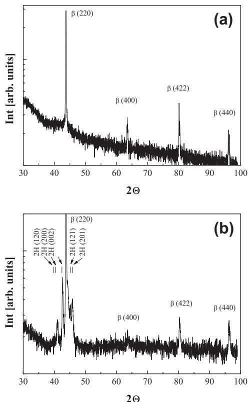
Fig. 2. (a) X-ray diffraction pattern at room temperature in a Cu–Zn–Al (F1) film obtained by reactive thermal annealing. The peaks were indexed according to the L_{21} structure. (b) X-ray diffraction pattern at room temperature in a Cu–Zn–Al (F2) film obtained by reactive thermal annealing. The peaks were indexed according to the L_{21} structure and to the 2H martensitic structure.
