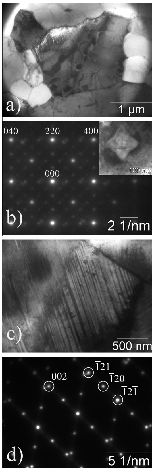
Fig. 4. Film F2. (a) After heating, the film is mainly in the \beta phase with the L2_1 structure. Antiphase boundaries can be observed in some grains. (b) [100] Electron diffraction pattern of the \beta phase with additional reflections corresponding to a \gamma -phase precipitate (inset). (c) After cooling, the film is in 2H martensite. Twinned variants can be observed. (d) Electron diffraction pattern of the twinned 2H martensite from a [210]_{2H} orientation.
