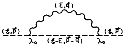
FIG. 1. Second-order contribution to the Reggeon self-energy.
