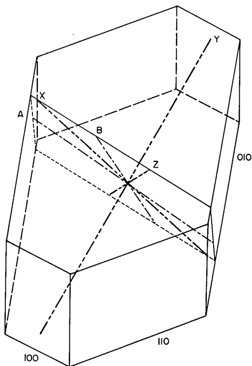
FIG. 2. Preliminary optical orientation of huerulite.
