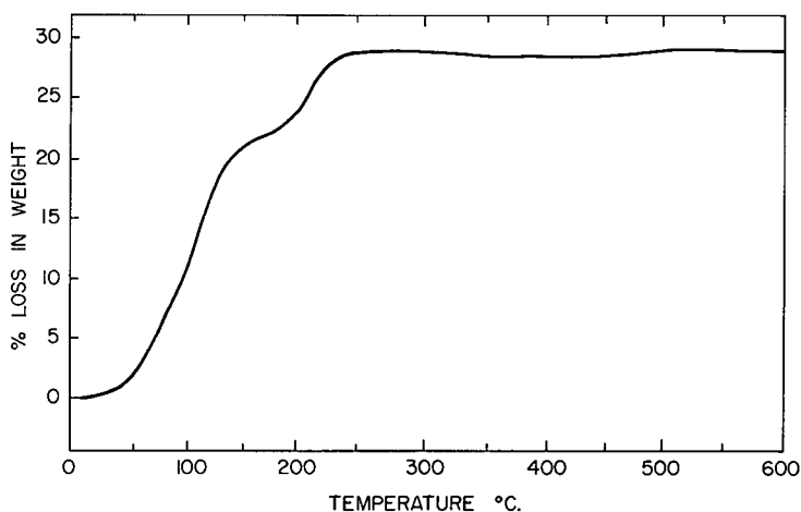
Fig. 4. Chevenard thermobalance curve of huemulite.
