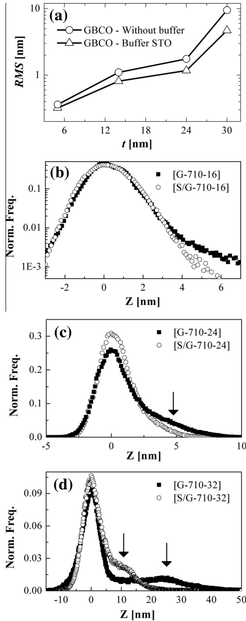
Fig. 3. (a) Thickness dependence of the RMS roughness of pure and STO buffered GBCO thin films. (b)–(d) Histograms of peak height profile for the different films based on the AFM images shown in Fig. 2. The frequency was normalized by the area under the curves. Arrows indicate a bimodal distribution by 2D and 3D growth.
