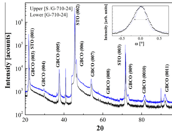
Fig. 1. X-ray diffractogram (logarithmic intensity scale) of the [\text{G}-710-24] and the [\text{S/G}-710-24] films at room temperature. The inset shows the rocking curves for the (005) reflection.
