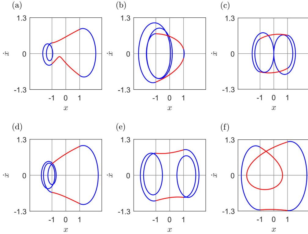
Fig. 5. Six different non-physical orbits obtained with the proposed method for excitation frequency of \omega = 0.26 and the same parameters as in Fig. 4. Red colour is used to mark the trajectory described by the solution inside the gap ( |x| < e ) and blue colour for the trajectory described by the solution outside the gap ( |x| > e ).
