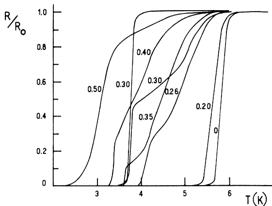
FIG. 2. Resistivity ratio as a function of temperature for \text{Cu}_x\text{La}_{1-x} sput-cooled samples. The resistance is normalized by the residual one, R_0 , for each sample.
