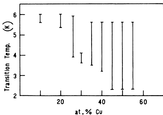
FIG. 3. Superconductive transition temperature as a function of alloy composition. Vertical bars indicate the total transition width (100% of the superconductive transition).
