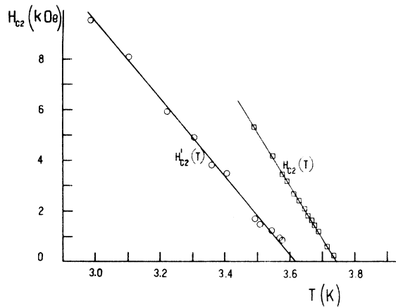
FIG. 6. Upper critical field as a function of temperature for a splat-cooled \text{Cu}_{30}\text{La}_{70} sample. H_{c2}(T) represents the results obtained by dc electrical resistivity measurements and H'_{c2}(T) those obtained by ac susceptibility measurements. The solid line is a mean square fit of the experimental data.
