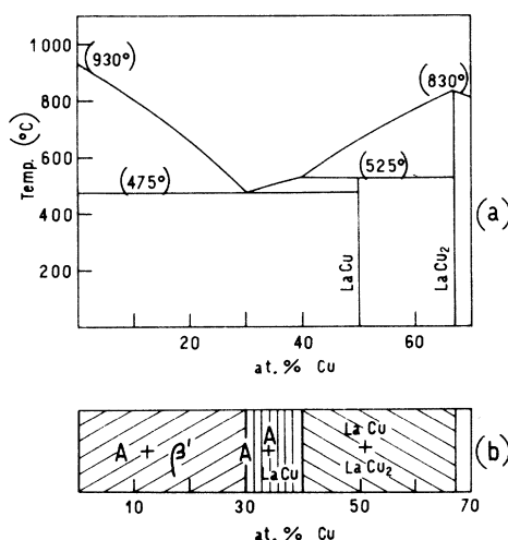
FIG. 1. (a) Constitutional phase diagram of the Cu-La system (Ref. 7). (b) Nonequilibrium diagram obtained by x-ray analysis of the splat-cooled samples of Cu-La.
