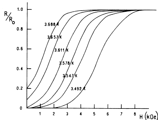
FIG. 4. Resistivity ratio as a function of magnetic field and temperature for a disordered \text{Cu}_{30}\text{La}_{70} sample.
