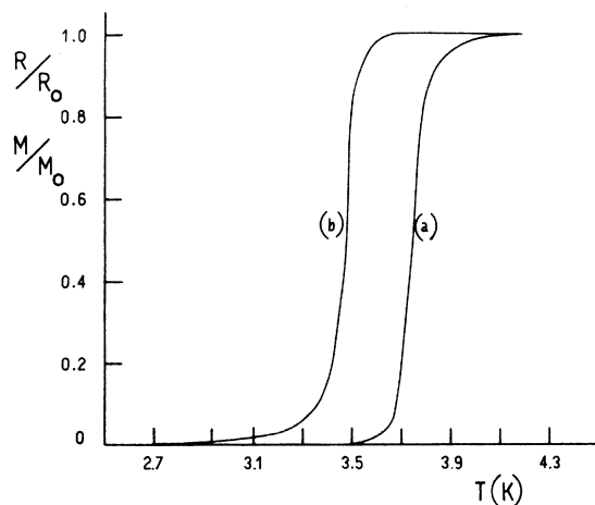
FIG. 5. (a) Resistivity ratio as a function of temperature for a \text{Cu}_{30}\text{La}_{70} sput-cooled sample. (b) Normalized amplitude of the ac susceptibility as a function of temperature for the same \text{Cu}_{30}\text{La}_{70} sample.
