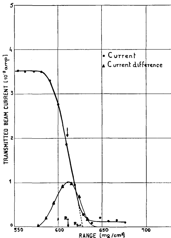
FIG. 3. Example of beam energy measurement data.
