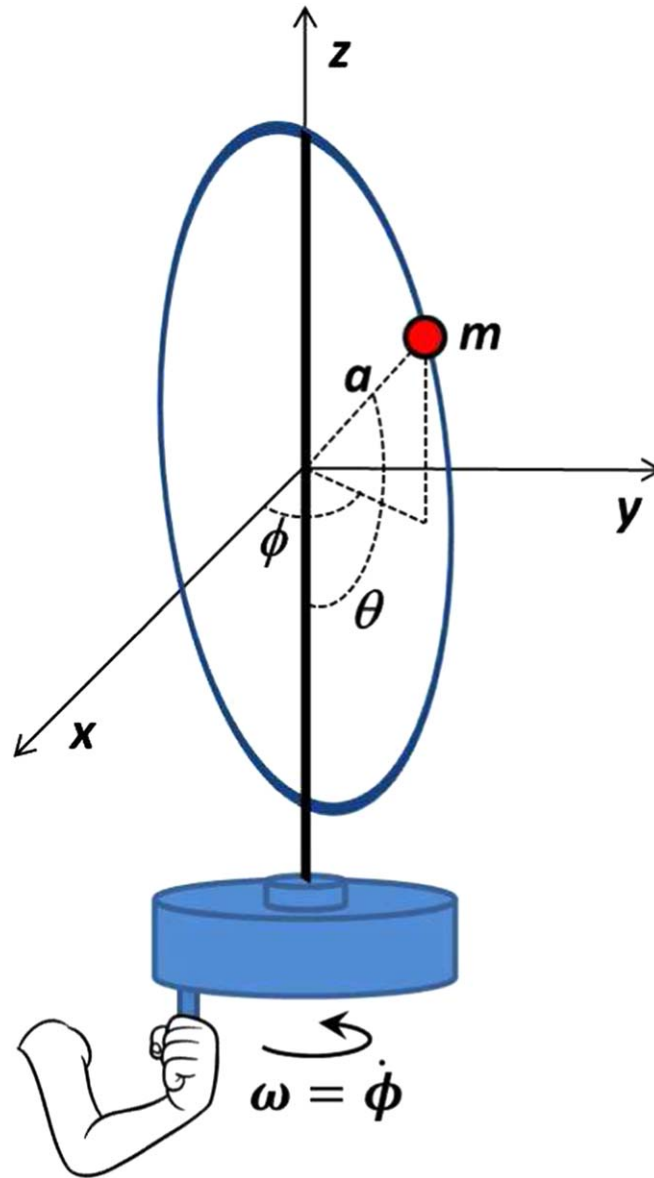
Figure 1. A bead of mass m on a rotating hoop of radius a and constant angular velocity \omega , under gravity.
