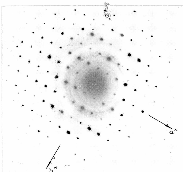
FIG. 2. Selected area electron diffraction pattern of ranquillite. Plane of the grid is approximately normal to the electron beam. 100 KV.
