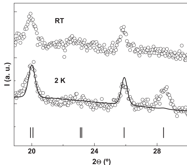
Fig. 8. Detail of the neutron powder diffraction pattern at RT and 2 K, showing the appearance of an extra peak (ca. 28^\circ ) due to weak long range magnetic coupling at low temperature. Vertical bars are Bragg positions for the crystallographic cell.
