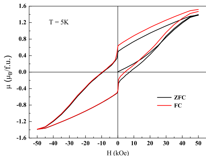
Fig. 5. Hysteresis loop at 5 K taken after ZFC (black “on line”) and FC (red “on line”) conditions. (For interpretation of the references to color in this figure legend, the reader is referred to the web version of this article.)
