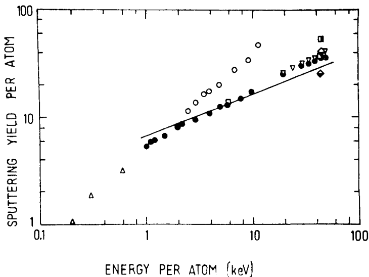
Figure 1 Sputtering yields per atom for Au bombardment with Xe and Xe 2 . ▼ Almen and Bruce 7 ; Δ Rosemberg and Wehner 8 ; □ Andersen and Bay 3 ; ▽ Nenadovic et al 9 ; ◆ EerNisse 10 ; ○ Szymonski and de Vries 11 ; ● Xe and ○ Xe 2 , this work; — Sigmund's theoretical prediction.
