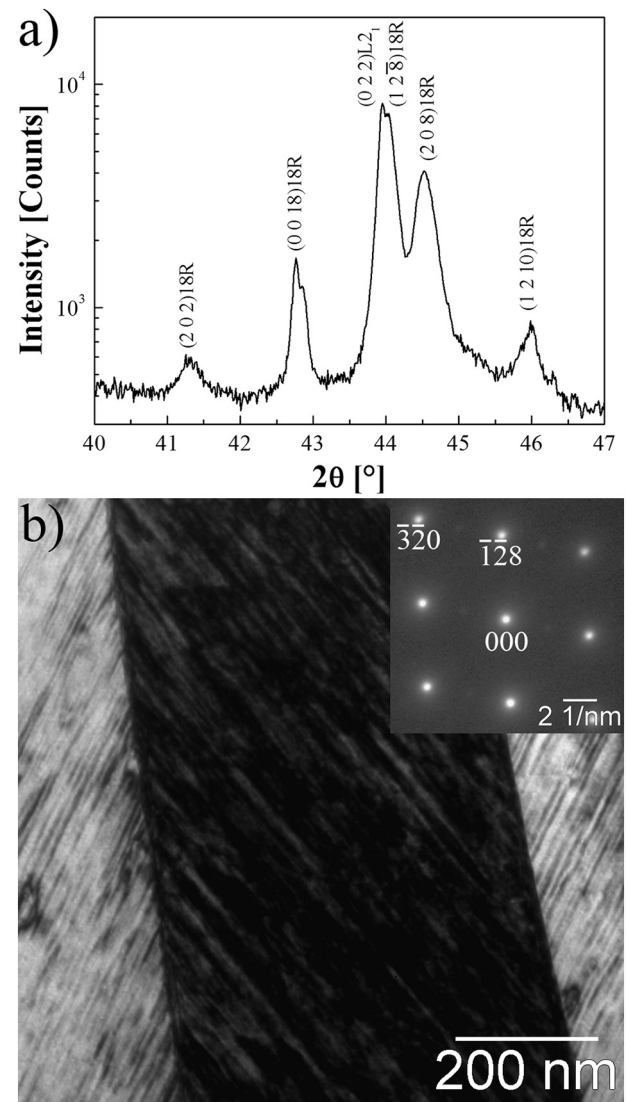
Fig. 6. a) X-ray diffraction patterns at room temperature of [1123 K-20 m] (after warming up the film from liquid N_2 temperature). b) Plan-view bright field TEM image in [1123 K-20 m] showing 18R twinned martensite. Inset shows the electron diffraction pattern along the [46\bar{1}] direction corresponding to the dark central 18R plate.
