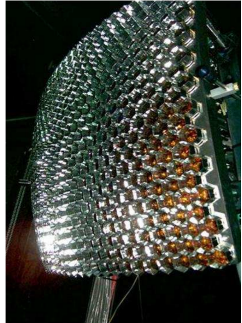
Figure 3.6: Left: Schematic view of an FD telescope and its main components. Right: Picture of an FD camera and its 440 PMTs. Taken from Ref. [43]
