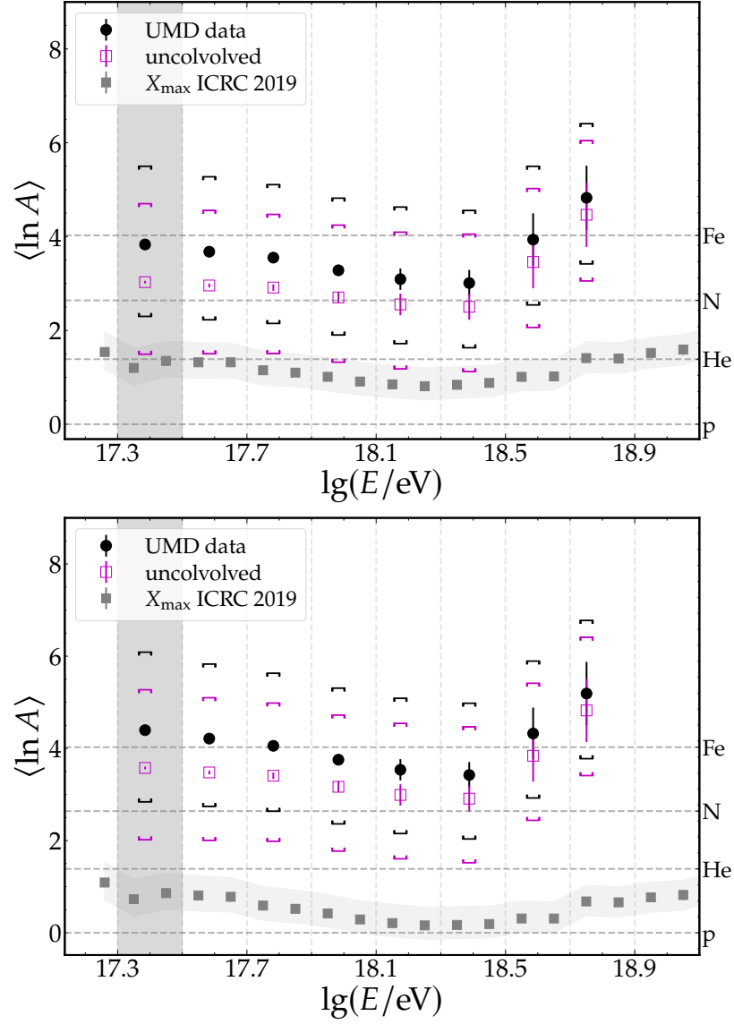
Figure F.3: Mean logarithmic mass as a function of energy for EPOS-LHC (upper panel) and QGSjetII-04 (lower panel). Error bars indicate statistical uncertainty, whereas brackets correspond to systematic uncertainties. Grey markers indicate the logarithmic mass inferred from X_{\text{max}} measurements [84]. The shaded grey area indicates the energy bin below full efficiency (see Section 7.1.1), preserved for visualization only. The magenta markers indicate the masses inferred with the uncolvolved densities shown in Fig. 7.31.
