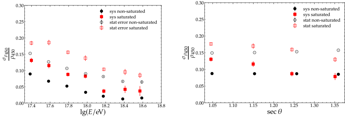
Figure 7.20: Statistical and systematic uncertainties of \rho_{450} as function of energy (left) and \sec \theta (right). Saturated and non-saturated events are treated separately.
