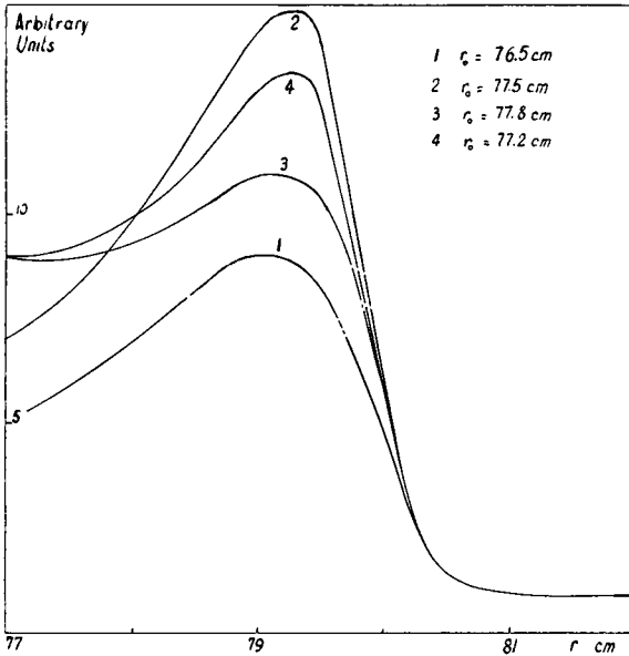
Fig. 6. Detector current versus radius for different radial position of the regenerator.
