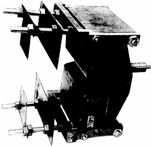
Fig. 2. Regenerator assembly.
