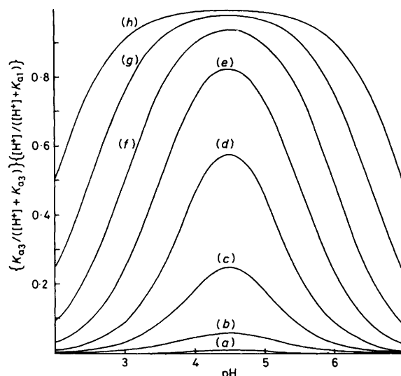
FIGURE 8 Dependence of the dissolution rate constant k of magnetite on pH, according to the term \{K_{a3}/([H^+] + K_{a3})\}\{[H^+]/([H^+] + K_{a1})\} of equation (11), for different values of the ratio K_{a1}:K_{a3} : curve (a) 10^2 , (b) 10, (c) 1, (d) 10^{-1} , (e) 10^{-2} , (f) 10^{-3} , (g) 10^{-4} , and (h) 10^{-5} .
