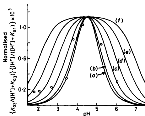
FIGURE 9 Dependence of the dissolution rate constant k of magnetite on pH, according to the term \{K_{a3}/([H^+] + K_{a3})\}\{[H^+]/([H^+] + K_{a1})\} of equation (11), for different values of the ratio K_{a1}:K_{a3} (curves have been normalized by equating the values at the maxima to the maximum experimental k value): (a) 1, (b) 10 and 10^{-1} , (c) 10^2 and 10^{-2} , (d) 10^3 and 10^{-3} , (e) 10^4 and 10^{-4} , and (f) 10^5 and 10^{-5} ; (○) experimental values
