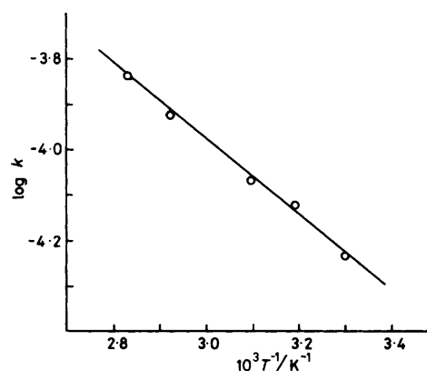
FIGURE 10 Temperature dependence of the dissolution rate constant k of magnetite at pH 4.0; [\text{HSCH}_2\text{CO}_2\text{H}] = 0.524 \text{ mol dm}^{-3}
