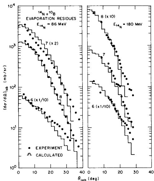
FIG. 3. Angular distributions of evaporation residues of oxygen, nitrogen, and carbon at E_{14N} = 86 MeV (left side) and 180 MeV (right side) for the ^{14}\text{N} + ^{10}\text{B} fusion reaction. The data are the experimental cross sections and the histograms are the Monte Carlo calculations discussed in the text.
