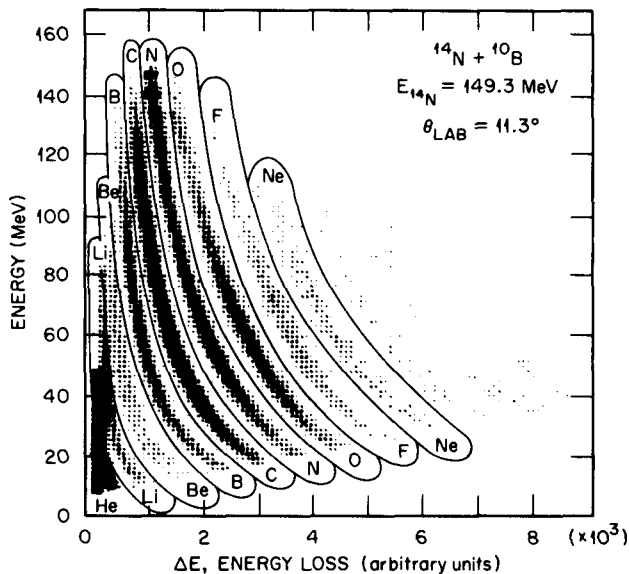
FIG. 1. \Delta E vs E array for the reaction products of ^{14}\text{N} + ^{10}\text{B} at E_{14\text{N}} = 149 MeV and \theta_{\text{lab}} = 11.3^\circ . The total energy E was obtained by analog summation of the signals from the ionization chamber and solid-state detector. The curves around the contours of constant Z were used to obtain the projections along the E axis.
