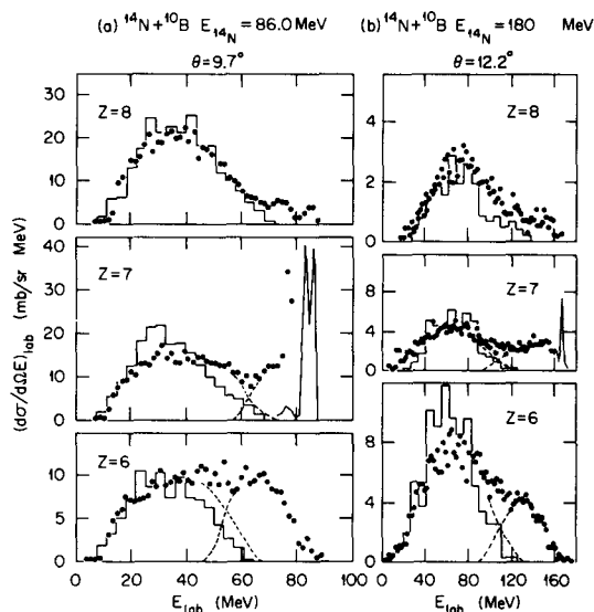
FIG. 2. (a) Energy spectra of oxygen, nitrogen, and carbon ions produced in the ^{14}\text{N} + ^{10}\text{B} reaction at E_{14\text{N}} = 86 MeV and \theta_{\text{lab}} = 9.7^\circ . The histograms are the results of Monte Carlo calculations discussed in the text. The dashed lines for the nitrogen and carbon spectra indicate separation assumed between low-energy (evaporation residues) and high-energy (direct reaction products) components. (b) Energy spectra of oxygen, nitrogen, and carbon ions from the ^{14}\text{N} + ^{10}\text{B} reaction at E_{14\text{N}} = 180 MeV and \theta_{\text{lab}} = 12.2^\circ . The curves through the data points have the same meaning as in (a).
