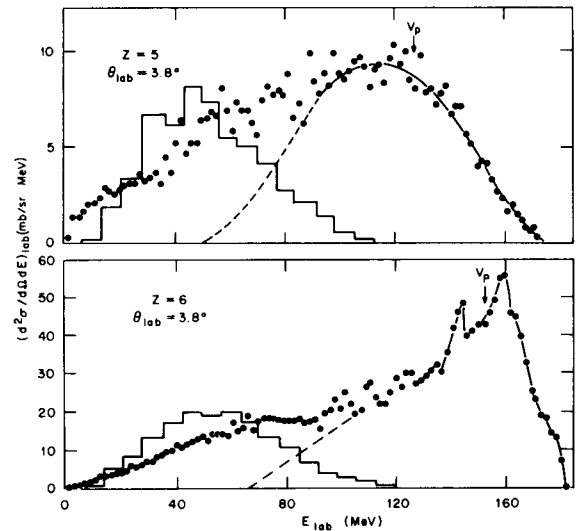
FIG. 8. Energy spectra for carbon and boron isotopes from the ^{14}\text{N} + ^{10}\text{B} reaction at E_{14\text{N}} = 180 MeV and \theta_{\text{lab}} = 3.8^\circ . The dashed lines indicate the separation between the high (direct) and low (evaporation residue) energy components. The histograms are predictions of the Monte Carlo Hauser-Feshbach calculations.
