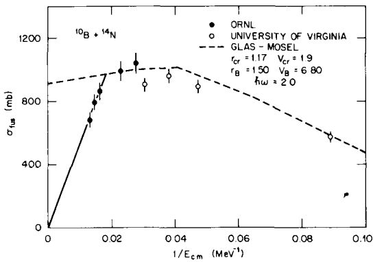
FIG. 10. The fusion cross section (in mb) plotted against 1/E_{c.m.} . The solid points are the present results; the open circles are from Ref. 11. The dashed line is the Glas-Mosel fit with the indicated parameters. The solid line intersecting the origin indicates that \sigma_{fus} \propto 1/E_{c.m.} at high energies, which can be interpreted as evidence for a saturation of the angular momentum at 21 \pm 1\hbar .
