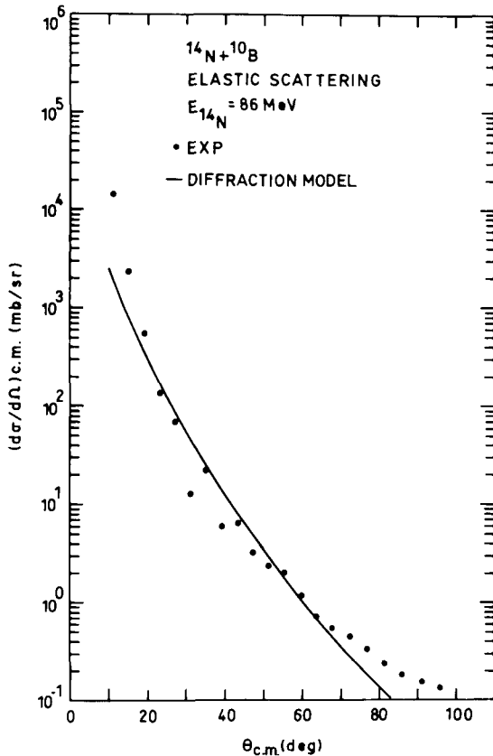
FIG. 9. The elastic scattering of ^{14}\text{N} + ^{10}\text{B} at E_{14N} = 86 MeV. The solid line is the angular distribution predicted by the diffraction model.
