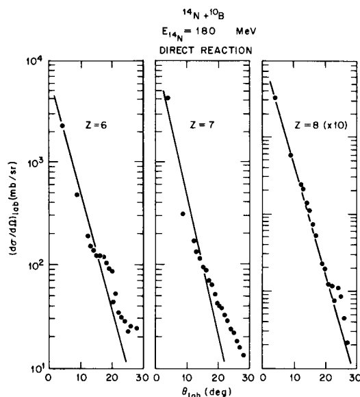
FIG. 4. Angular distributions of the direct reaction products for the ^{14}\text{N} + ^{10}\text{B} system at E_{14N} = 180 MeV. The solid line is the result of the diffraction model analysis discussed in the text.
