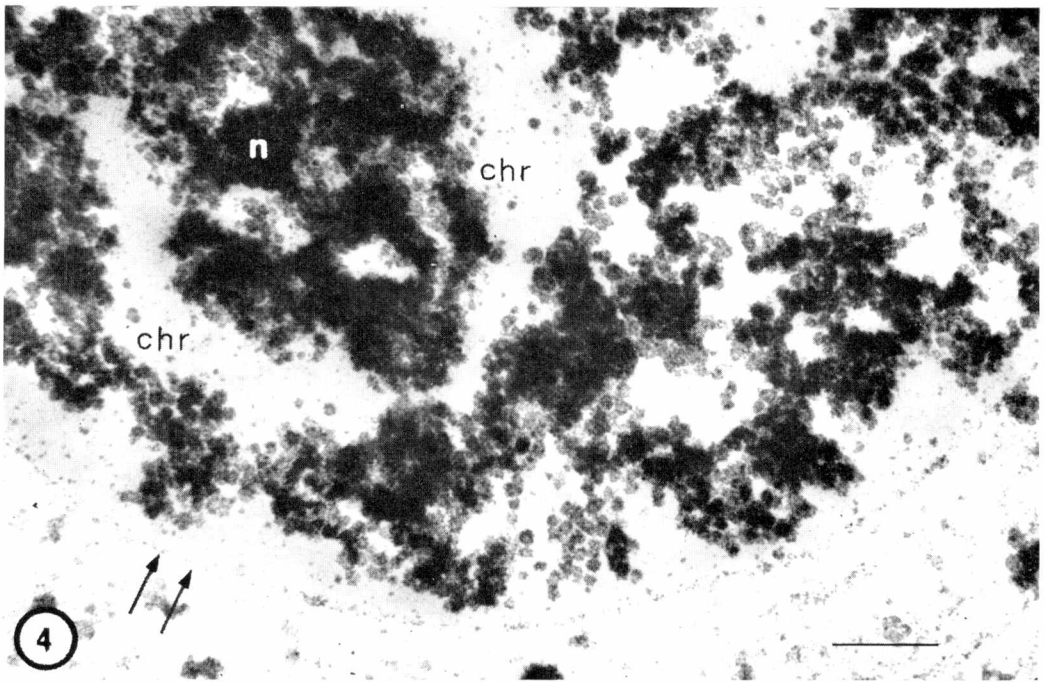
FIGURE 4 Electron micrograph of part of a rat liver cell nucleus; fixation as for Fig. 3. The condensed chromatin ( chr ) associated with the nucleolus ( n ) and the nuclear membrane (double arrow) are relatively free of precipitate which is massively deposited in the nucleolus and in the rest of the nucleus. Mark, 0.5 \mu . \times 28,500 .
