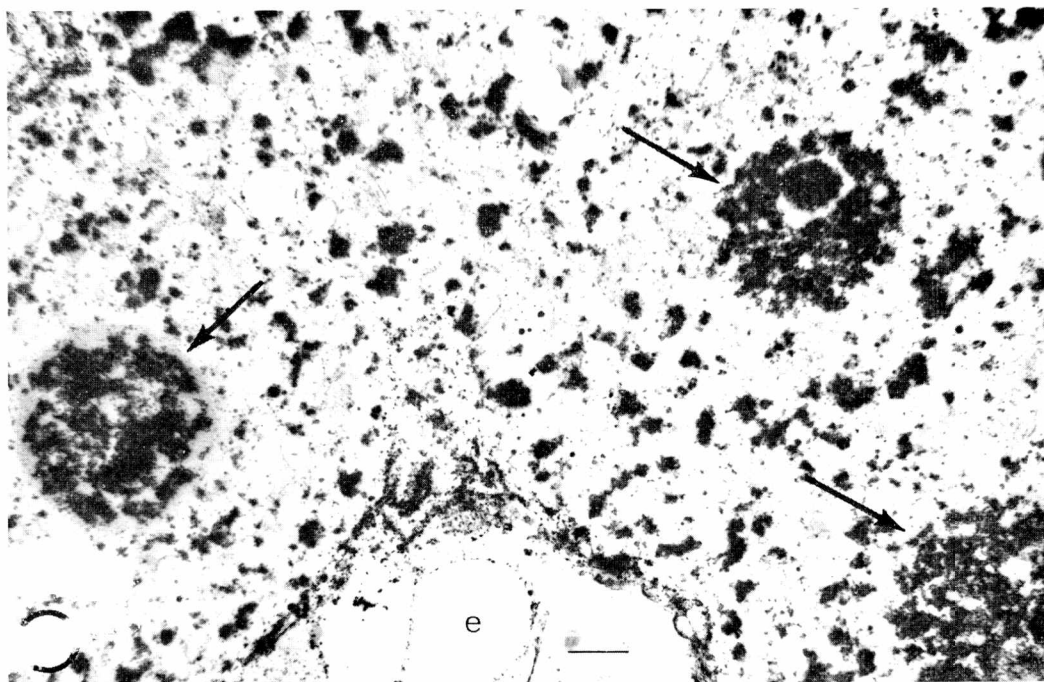
FIGURE 3 Survey electron micrograph of a thin section of rat liver fixed in half-saturated potassium pyroantimonate, illustrating the generality of the reaction. The precipitates are localized in the nuclei (arrows), in several discrete masses in the cytoplasm, and in the wall of the blood vessel; e, erythrocyte. Mark, 2\ \mu . \times 4,000 .
