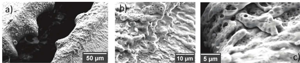
4 5 Figure 9. SEM micrographies (a) contiguous cavities machined on the copper coating of a PCB with 25 pulses each. (b, 6 c) Micrographies at larger magnifications to show the porosity.
