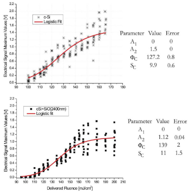
3 4 Figure 2. Amplitude of the electric signal versus laser fluence fitted by the logistic function of Eq. (1). (a) For c-Si and 5 (b) for c-Si + SiO 2 (2400) along with the values of the fitting functions' parameters. 6 The results were fitted with the heuristic curves described by Eq. (1), the parameters of which 7 are related to the physical properties of irradiated substrates [34]:
