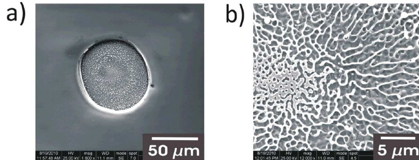
Figure 5. c-Si + \text{Si}_3\text{N}_4(370) nanostructuring obtained with a ns laser pulse (Nd:YAG, 8 ns, 532 nm). (a) Complete cavity. (b) Magnification of the cavity base.
