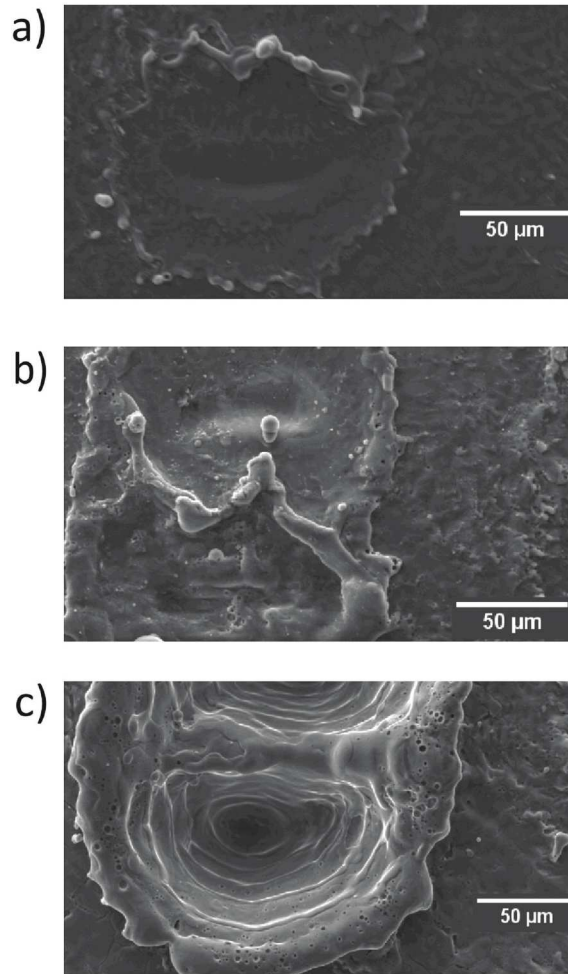
4 5 Figure 8. SEM micrographies of cavities drilled on a Ta(99.9%) sample with (a) 1, (b) 500, and (c) 1000 laser pulses of 6 200 mJ/cm 2 .
