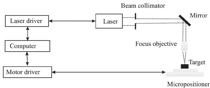
8 Figure 1. Micromachining system diagram.
