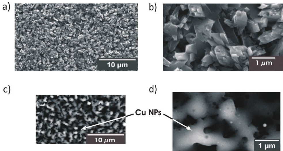
13 14 Figure 10. SEM micrographies of a copper oxide surface: (a, b) before irradiation; (c, d) after irradiation with one 15 square laser shot. Cu nanoparticles of lighter color than the rest of the surface due to their larger conductivity can be 16 appreciated.
