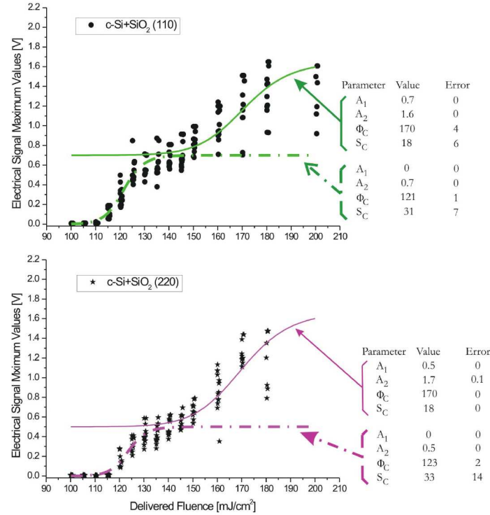
2 Figure 4. Amplitude of the electric signal versus laser fluence fitted by the logistic function, of Eq. (1) for two silicon 3 dioxide thin films thicknesses deposited with the EPCVD technique on monocrystalline silicon: 110 and 220 nm. The 4 parameters of logistic function are shown too.
