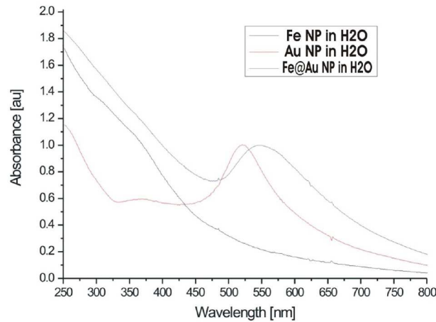
Figure 15. Absorbance spectrum of dispersions of Fe NPs, Au NPs Au, and Fe@Au NPs in ultrapure H 2 O.
