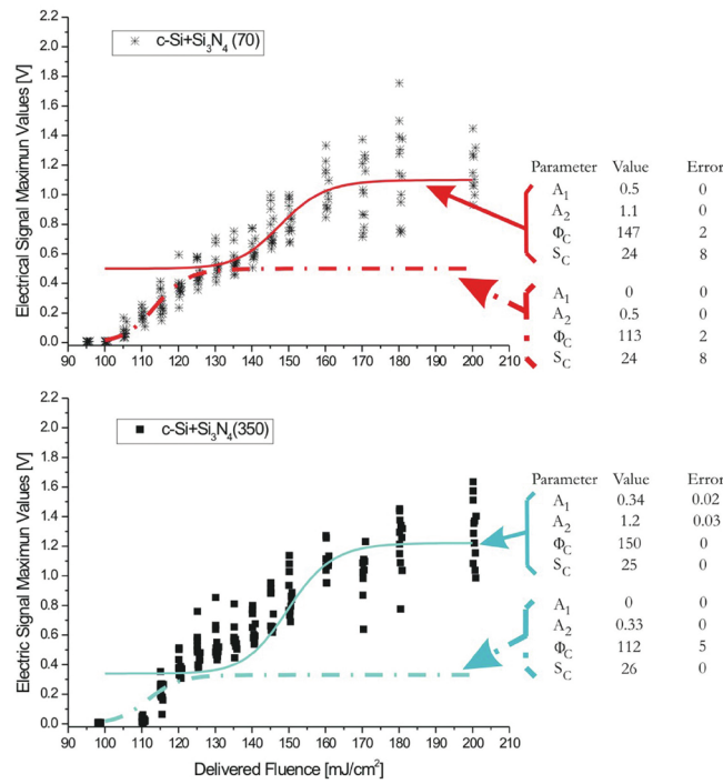
11 12 Figure 3. Amplitude of the electric signal versus laser fluence fitted by the logistic function, Eq. (1) for \text{Si}_3\text{N}_4 thin films 13 thicknesses deposited with the EPCVD technique on monocrystalline silicon: 70 and 350 nm. The parameters of the 14 logistic function are shown too.
