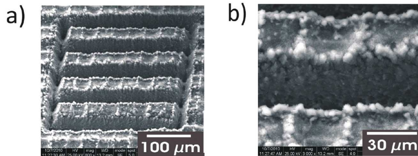
Figure 6. SEM microographies of (a) the c-Si sample surface after machining. (b) Magnification of part of the machined channels to show the deeper channels. In order to observe the roughness of the channel's wall, the sample's surface was placed forming an angle of 20^\circ with electron beam.
