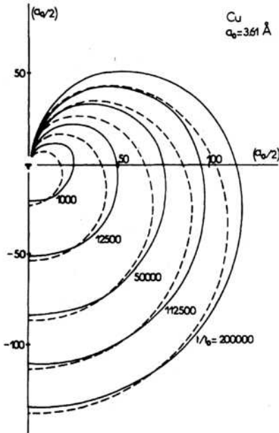
FIG. 1. Vacancy-depleted zone around an edge dislocation in Cu at 300 K. The time is taken in units of t_0 = \nu_0^{-1} \exp(Q_0/kT) , and M dipole tensors (Ref. 13) are used. Solid line: "discrete approximation," Eq. (1). Dashed line: R^{CB}(\theta, t) and "discrete approximation" with zero dipole tensor at the saddle point.
