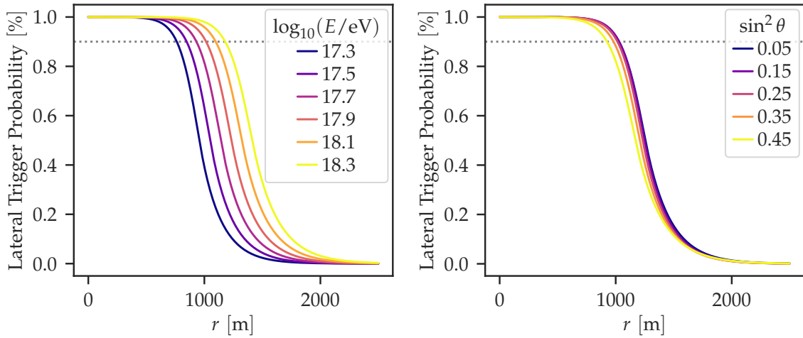
Figure 6.13: Lateral trigger probability (LTP) as a function of the distance to the shower axis, as parameterized in Ref. [114]. The left panels shows said curves for different energies at fixed \sin^2 \theta = 0.25 , while the right panel shows them for different zenith angles at \log_{10}(E/\text{eV}) = 17.9 . Gray dashed lines mark 90 % lateral trigger probability.
