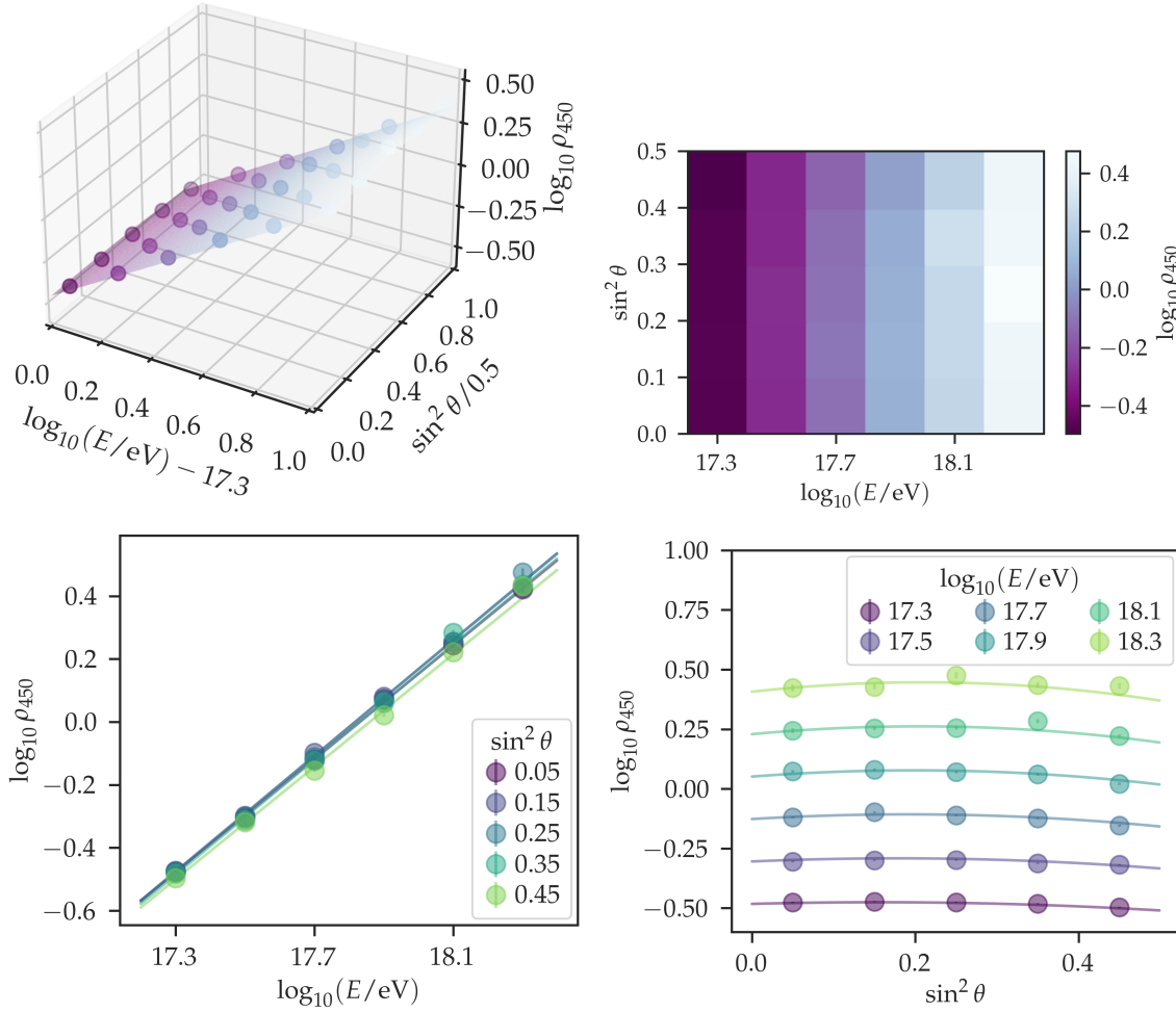
Figure 6.19: Parameter \log_{10} \rho_{450} of the modified-NKG fits to data (see text for details), as a function of the \log_{10}(E/\text{eV}) and \sin^2 \theta bins. The surface and lines are the result of the biquadratic fit (c.f. Eqs. (6.24) and (6.26)). Top left: 3-dimensional plot. Top right: 2-dimensional projection. Bottom left: \log_{10} \rho_{450} as a function of \log_{10}(E/\text{eV}) , with the different \sin^2 \theta -bins in different colors. Bottom right: \log_{10} \rho_{450} as a function of \sin^2 \theta , with the different \log_{10}(E/\text{eV}) -bins in different colors.
