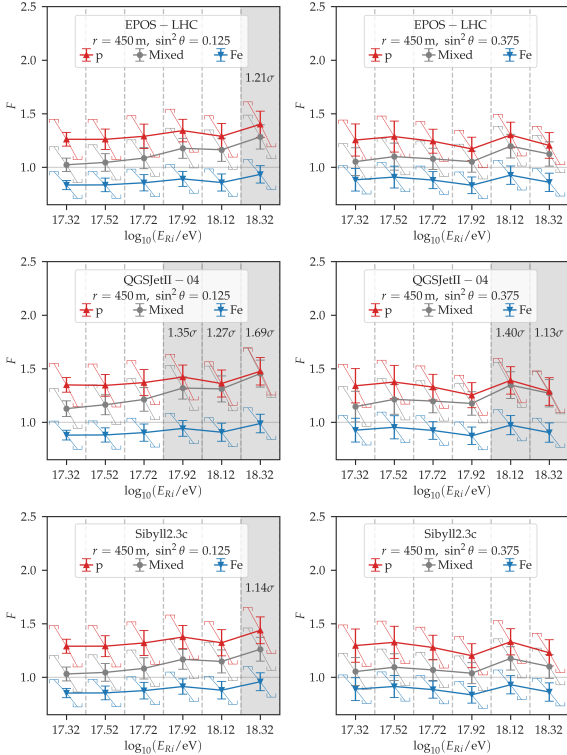
Figure 7.7: Same as Fig. 7.6, but for 2.60 \leq \log_{10}(r/\text{m}) < 2.70 ( r \sim 450 \text{ m} ).
