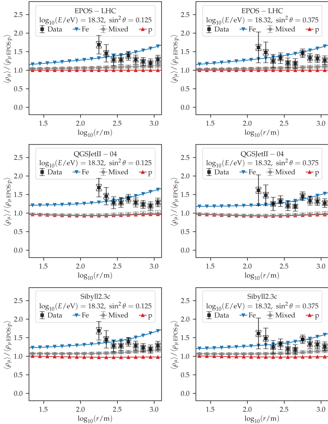
Figure B.5: Same as Fig. 7.2 but for the reconstructed energy bin centered at \log_{10}(E_{Ri}/\text{eV}) = 18.32 .
