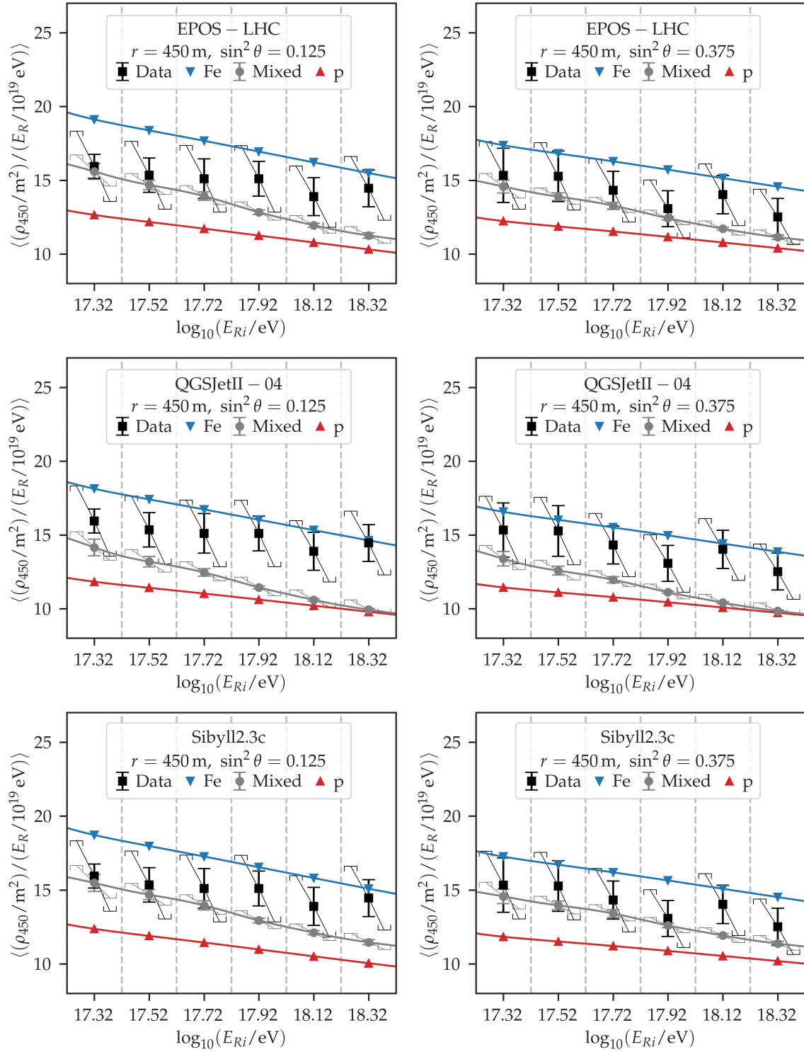
Figure 7.4: Same as Fig. 7.3, but for 2.60 \leq \log_{10}(r/m) < 2.70 ( r \sim 450 \text{ m} ).
