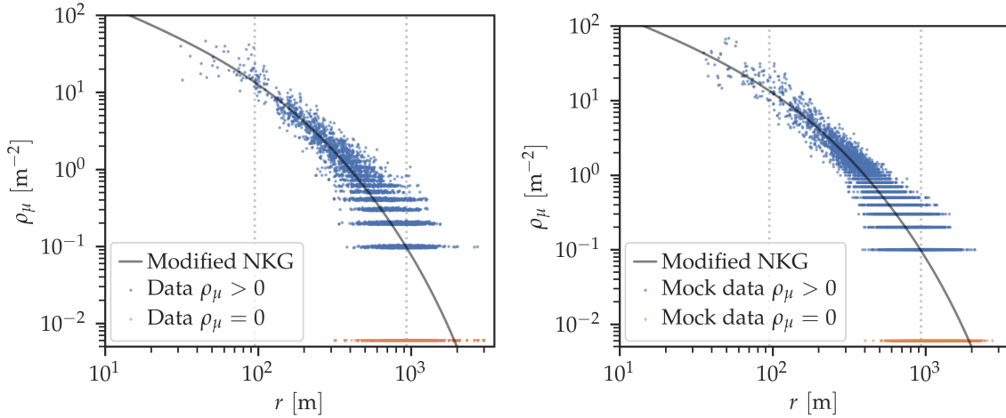
Figure 6.23: Muon density as a function of the distance to the shower axis for real (left panel) and mock (right panel) data. The muon LDF that is fitted to real data is the one used to generate the mock data, which is a modified NKG with parameters \log_{10} \rho_{450} = -0.12 and \beta = 2.70 (and the fixed parameters described in Sec. 6.5.2). The real data are events with reconstructed energies in 17.6 \leq \log_{10}(E/\text{eV}) \leq 17.8 and zenith angles in 0.2 \leq \sin^2 \theta \leq 0.3 . The dashed vertical lines are the minimum and maximum distance cuts that are used in data (see Secs. 6.3.5 and 6.3.6).
