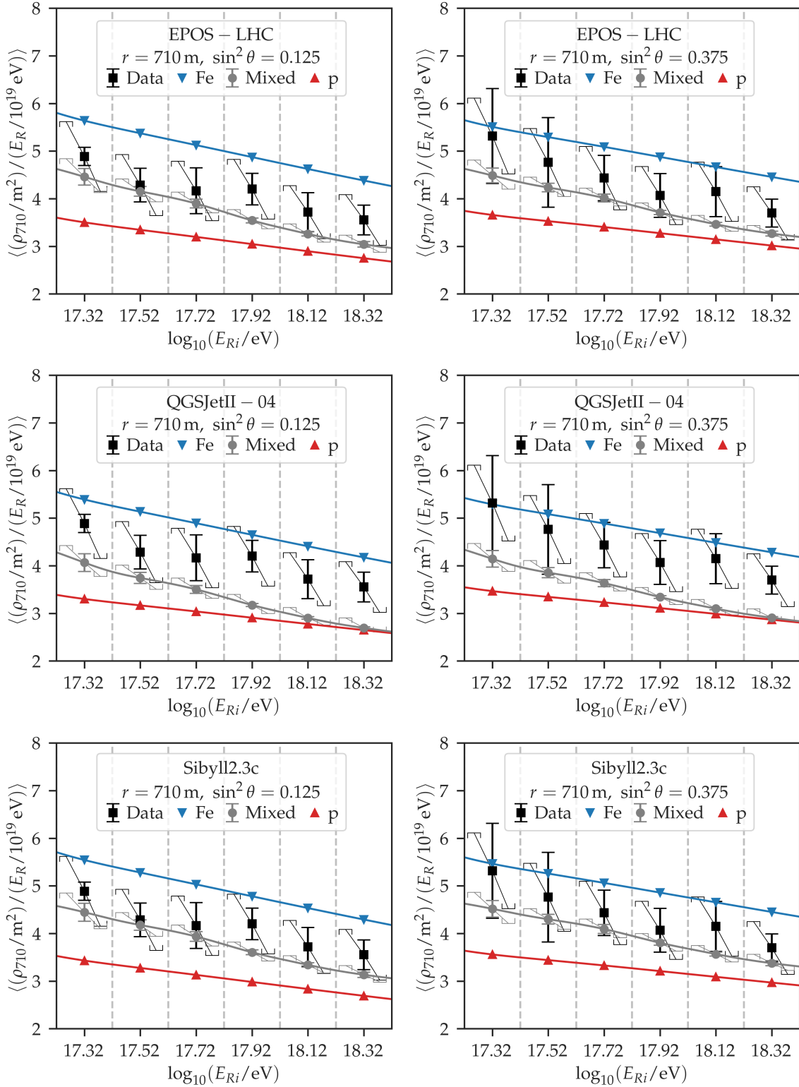
Figure 7.5: Same as Fig. 7.3, but for 2.80 \leq \log_{10}(r/\text{m}) < 2.90 ( r \sim 710 \text{ m} ).
