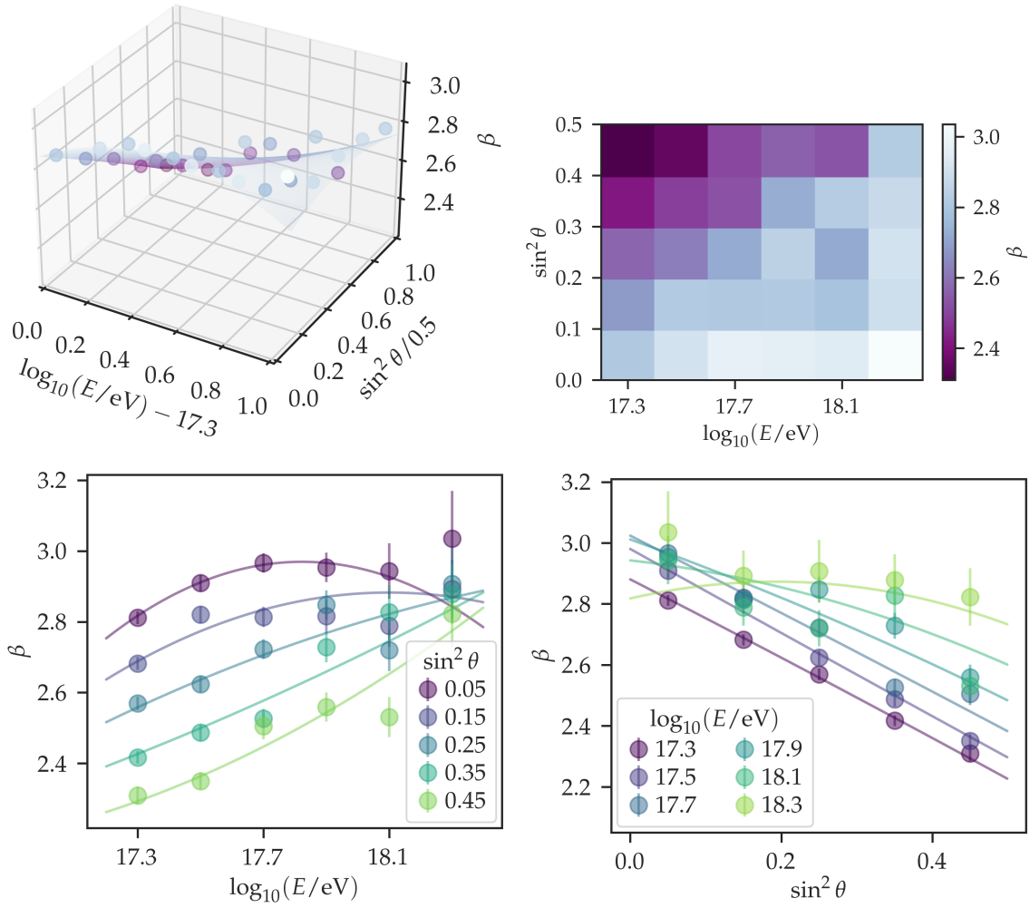
Figure 6.20: Same as Fig. 6.19 but for the parameter \beta . The parameterization is that of Eqs. (6.25) and (6.27).
