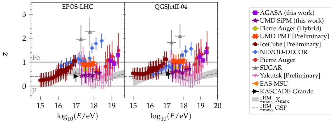
Figure 8.9: Values of z computed from the UMD data (c.f. Chapter 7), from AGASA data (this chapter), and from nine different data sets of seven experiments [5, 15, 59, 147], as a function of the logarithm of the center of the reconstructed energy bin for the three considered models. The left panel shows the values computed for EPOS-LHC, and the right panel for QGSJetII-04. Gray horizontal lines mark the expected values of z for pure proton and pure iron compositions (0 and 1 respectively). Dashed lines show the z -value expected from mixed composition scenarios considering the mass fractions of the GSF model, while the gray shaded area represents the ones expected from the fits to the X_{\max} distributions. The error bars represent total uncertainties (excluding the uncertainty of the reference energy scale).
