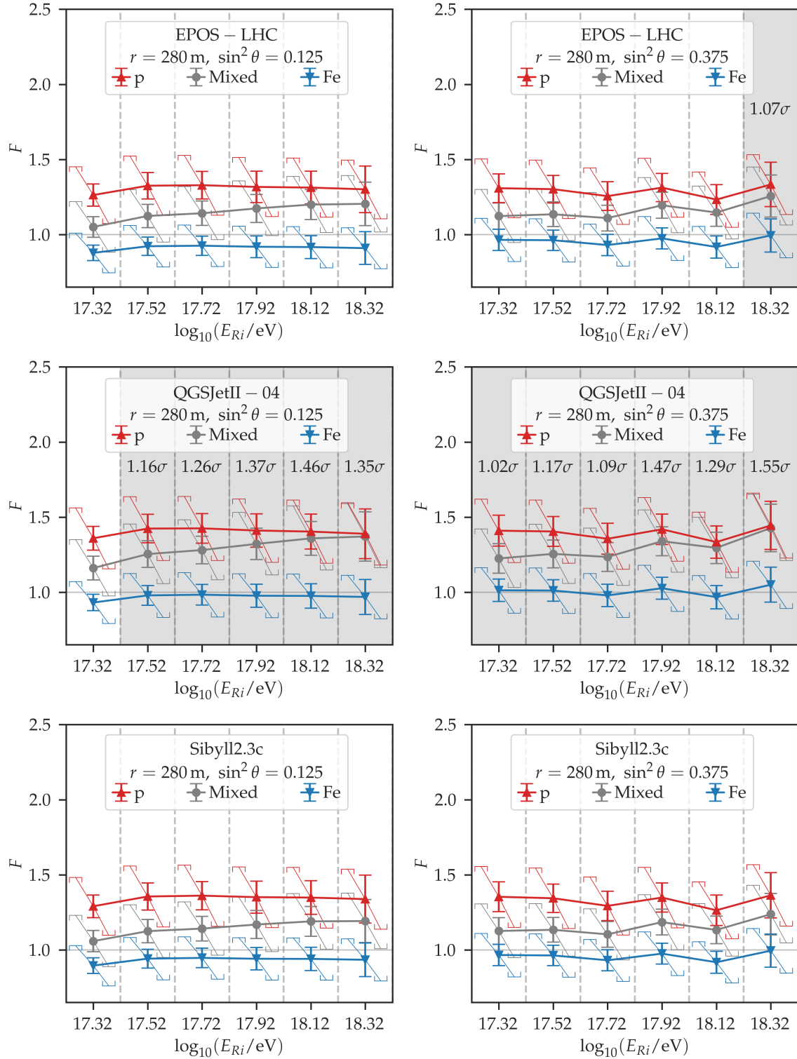
Figure 7.6: Correction factor F (see Eq. (7.20)), as a function of the center of the reconstructed energy bin, for 2.40 \leq \log_{10}(r/\text{m}) < 2.50 ( r \sim 280 \text{ m} ), considering a bin width of \Delta \log_{10}(E_R/\text{eV}) = 0.2 . Down triangles represent iron, circles represent the mixed composition scenarios, and up triangles represent proton. Statistical uncertainties are shown with error bars and systematic uncertainties with brackets. In the two upper panels the model is EPOS-LHC, in the central panels it is QGSJetII-04, and in the bottom panels it is Sibyll2.3c. The three left panels show the comparison for the smaller zenith angles ( \theta < 30^\circ ), and the three right panels for the larger zenith angles ( 30^\circ \leq \theta < 45^\circ ). Highlighted in gray are the reconstructed energy bins where the correction factor F , that makes the mixed composition scenario match data, is larger than 1 with a significance of more than 1\sigma ; in these cases the significance is detailed in the same bin. A gray horizontal line marks F = 1 .
