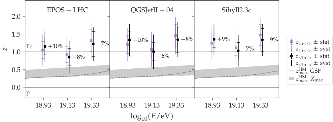
Figure 8.8: z_{\ln(\cdot)} (squares) and z_{\langle \ln \cdot \rangle} (circles), for EPOS-LHC (left), QGSJetII-04 (center), and Sibyll2.3c (right) as a function of the logarithmic reconstructed energy (in the reference energy scale). For clarity, we introduce a horizontal displacement between the two sets of values. The relative difference of z_{\langle \ln \cdot \rangle} to z_{\ln(\cdot)} is written next to each pair of points. We also show the values of z_{\text{mass}}^{\text{HM}} from the GSF model (gray dashed lines) and from the Pierre Auger X_{\text{max}} (gray shaded area) composition models.
