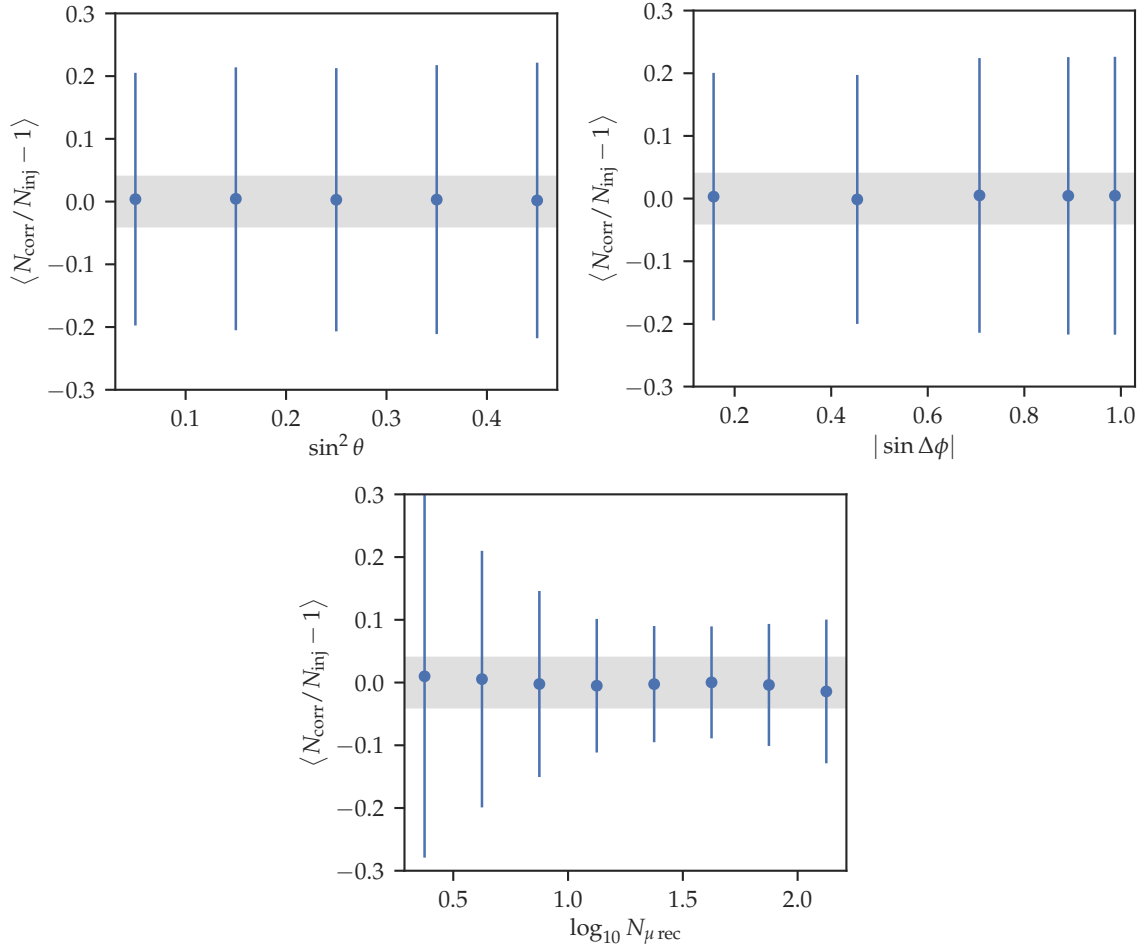
Figure 5.4: Bias in the corrected number of muons against the injected one (see Eq. (5.8)) as a function of \sin^2 \theta (top left), of |\sin \Delta \phi| (top right), and of \log_{10} N_{\mu \text{ rec}} (bottom). The points represent the mean of \varepsilon^* and the error bars the standard deviation of \varepsilon^* . The gray band marks \pm 4\% .
