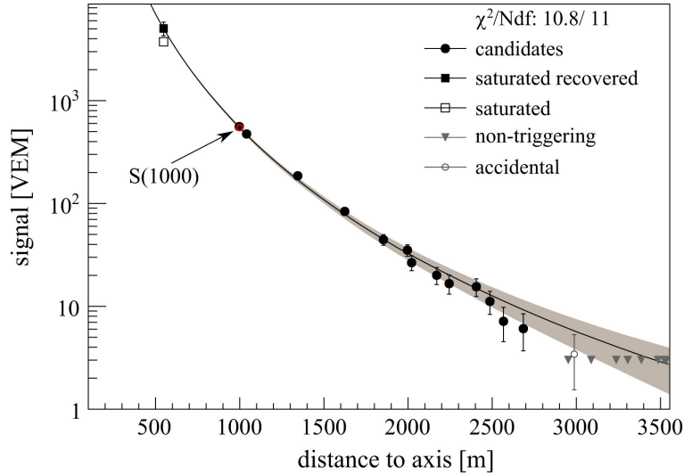
Figure 3.3: Measured signals (in VEM) as a function of the distance to the shower axis on the shower plane, for different types of stations (different markers), and the Offline fit (solid line) that uses a modified-NKG model (see text for details). Taken from Ref. [38].
