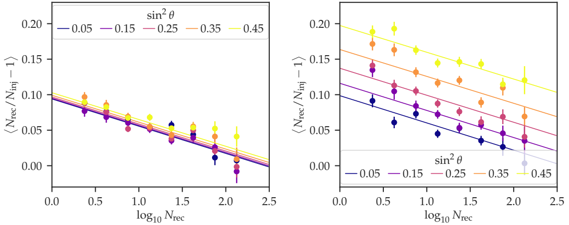
Figure 5.2: Bias in the reconstructed number of muons against the injected ones (see Eq. (5.1)) as a function of the logarithm of the reconstructed number of muons, for different \sin^2 \theta bins in different colors, and for two \Delta\phi bins: 7^\circ \lesssim \Delta\phi \lesssim 14^\circ in the left panel, and 76^\circ \lesssim \Delta\phi \lesssim 83^\circ in the right panel. The global fit is superimposed.
