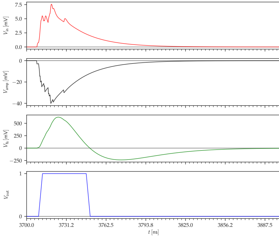
Figure 3.12: Simulation of the response of the electronics to one muon impinging on a scintillation bar. The muon generates photon-equivalents (top panel). The signal is then amplified and inverted by the pre-amplifier (second to top panel). Afterwards, the fast shaper further amplifies and inverts again the signal (second to bottom panel). Finally, the FPGA digitizes the signal (bottom panel).
