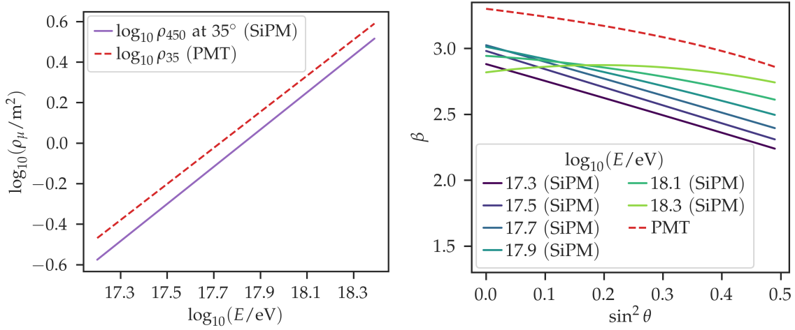
Figure 6.29: Left panel: Comparison between the parameterization of \log_{10} \rho_{450} of this work (c.f. Eq. (6.24)) evaluated at \theta = 35^\circ as a function of the logarithmic energy (solid line), and the parameterization of \log_{10} \rho_{35} from the UMD PMT data analysis (c.f. Eq. (6.32), dashed line). Right panel: Comparison between the parameterization of \beta from this work (c.f. Eq. (6.25)) evaluated at different energies (different colors, solid lines) as a function of the sine square of the zenith angle, and the one of the UMD PMT data analysis (c.f. Eq. (6.31), dashed lines).
