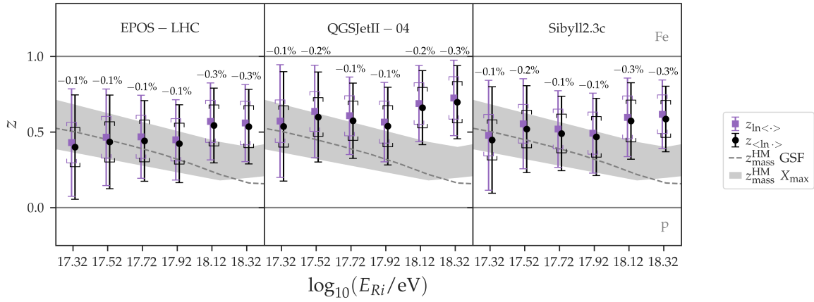
Figure B.6: z_{\ln\langle\cdot\rangle} (squares) and z_{\ln\langle\cdot\rangle} (circles), for EPOS-LHC (left), QGSJetII-04 (center), and Sibyll2.3c (right) as a function of the logarithmic reconstructed energy (in the reference scale). For clarity, we introduce a horizontal displacement between the two sets of values. The relative difference of z_{\ln\langle\cdot\rangle} to z_{\ln\langle\cdot\rangle} is written on top of each pair of points. We also show the values of z_{\ln\langle\cdot\rangle}^{\text{HM GSF}} from the GSF model (gray dashed lines) and from the Pierre Auger X_{\text{max}} (gray shaded area). Gray horizontal lines mark the expected values of z for pure proton and pure iron compositions (0 and 1 respectively). The statistic uncertainties are represented with error bars and the systematic uncertainties with brackets.
