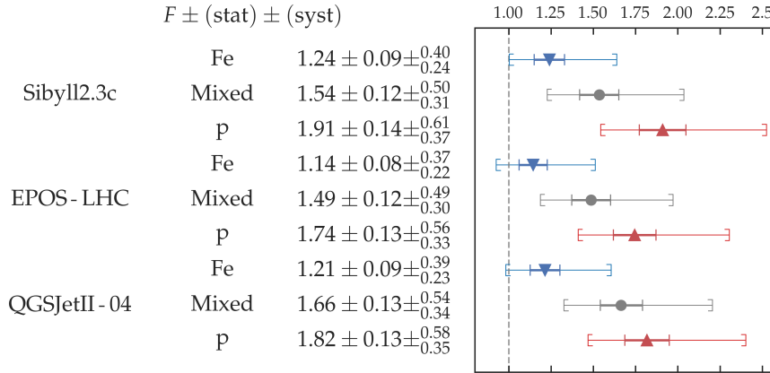
Figure 8.7: Correction factor F (see text for details) corresponding to the single nuclei and mixed composition scenarios, for the three considered models. The analyzed energy range is 18.83 \leq \log_{10}(E_R/\text{eV}) \leq 19.46 . The obtained values are reported in the table (left) and are also plotted (right) on the same row. The systematic uncertainties are depicted with square brackets.
