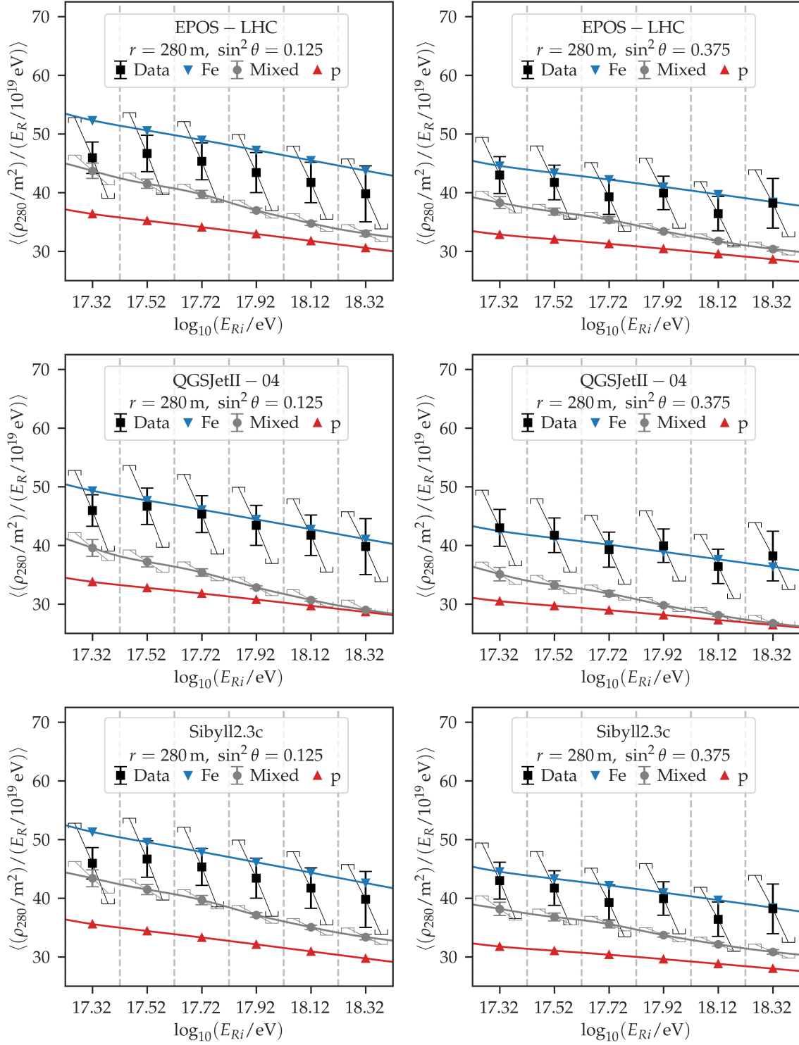
Figure 7.3: Average muon density divided by the reconstructed energy, as a function of the center of the reconstructed energy bin, for 2.40 \leq \log_{10}(r/m) < 2.50 ( r \sim 280 m). The considered bin width is \Delta \log_{10}(E_R/\text{eV}) = 0.2 . Square markers represent data, down triangles iron, circles represent the mixed composition scenarios, and up triangles proton. Error bars represent statistical uncertainties and brackets represent systematic uncertainties. These are contained within the markers in the case of proton and iron simulated densities. In the two upper panels the simulated muon densities and those of the mixed composition scenarios correspond to the model EPOS-LHC, in the central panels to QGSJetII-04, and in the bottom panels to Sibyll2.3c. The three left panels show the comparison for the smaller zenith angles ( \theta < 30^\circ ), and the three right panels for the larger zenith angles ( 30^\circ \leq \theta < 45^\circ ).
