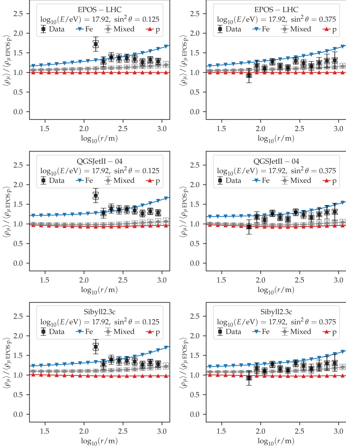
Figure B.3: Same as Fig. 7.2 but for the reconstructed energy bin centered at \log_{10}(E_{Ri}/\text{eV}) = 17.92 .
