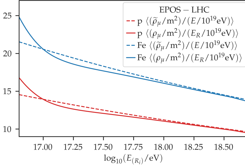
Figure 7.1: Average muon density at 450 m from the shower axis, divided by the energy, as a function of the logarithm of the Monte Carlo energy E (dashed lines) and average muon density at 450 m from the shower axis, divided by the reconstructed energy, as a function of the logarithm of the reconstructed energy bin E_{Ri} (solid lines). We used a bin width of \Delta \log_{10}(E/\text{eV}) = 0.2 . The high-energy hadronic interaction model used to generate the air showers is EPOS-LHC, and the primaries are proton (red) and iron (blue).
