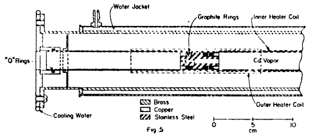
FIG. 5. The Cd-vapor absorption tube. The rate of escape of Cd through the apertures was negligible. The graphite rings were a satisfactory solution to difficulties with inserts sticking after heating. The inserts had sufficient friction to hold them in place; they could be positioned by detachable rods.
