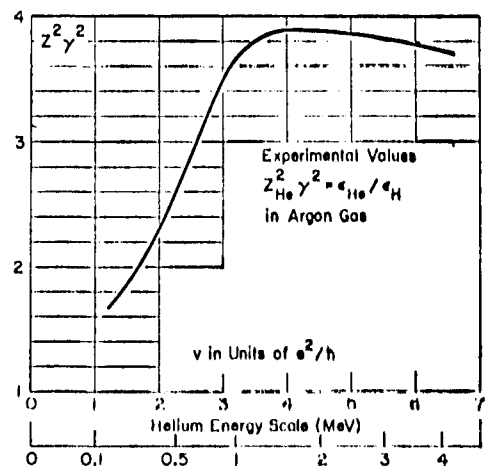
FIG. 1. The ratio of the atomic stopping powers of argon gas for He and H beams of the same velocity. The rising curve from 0.1- to 1.5 MeV He kinetic energy is due to the stripping of electrons from the H and He projectiles.
