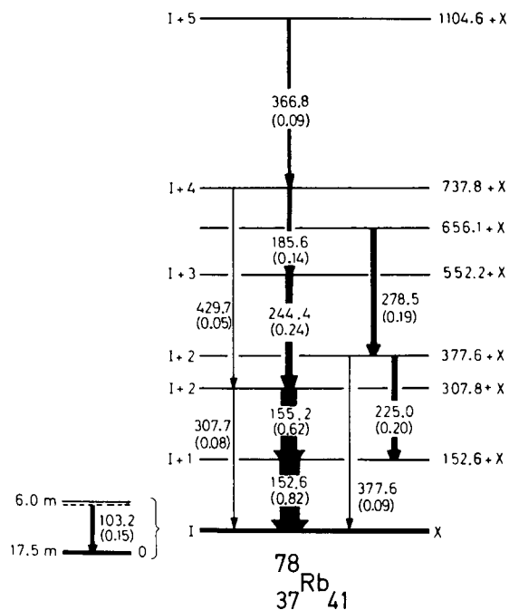
FIG. 4. Proposed level scheme for ^{78}\text{Rb} . It is not known which of the two previously known isomers in ^{78}\text{Rb} (indicated on the left) correspond to the lowest state I , but most probably it is the 6 min isomer.
