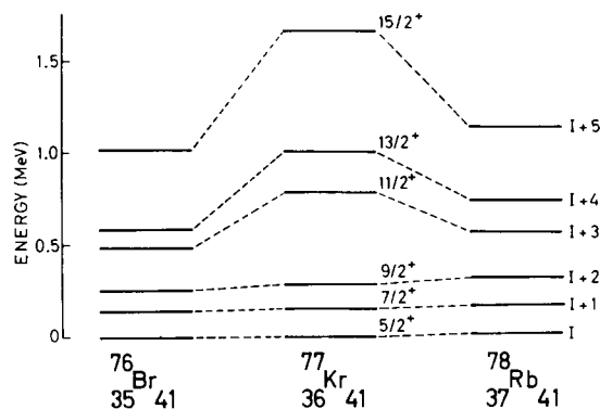
FIG. 5. The main band found in ^{78}\text{Rb} is compared to that in ^{76}\text{Br} (Ref. 1) and the 5/2^+ ground state band of ^{77}\text{Kr} (Ref. 2). The similarities in the excitation energies of the first two excited states as well as in the level staggering exhibited by the three nuclei are apparent.
