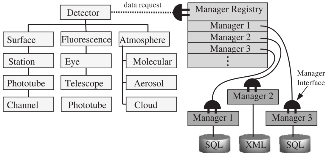
Figure 3.2: Schematic depiction of detector description machinery in Offline (taken from [28]) including both logically motivated classes (left) capable of sending requests for data to the manager registry (right). This machinery has been updated for greater flexibility in the grouping of hardware components and the time evolution of hardware on the level of individual surface detector stations.
