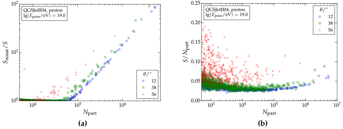
Figure 3.19: (a) Ratio of signal without and with simulation of electronics saturation as a function of station particle number. The particle number threshold at which saturation occurs depends on zenith angle. (b) Signal per particle as a function of station particle number. See Fig. B.2 in Appendix B for the corresponding muon fractions.
