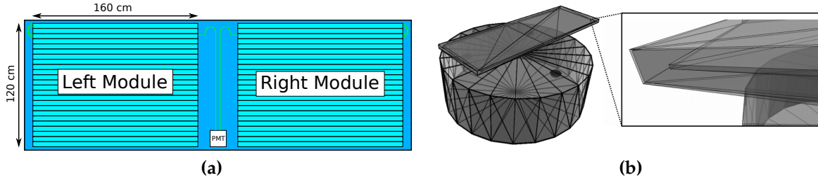
Figure 3.5: (a) Schematic of a surface scintillator detector, which is comprised of two symmetric modules consisting of 24 polystyrene scintillator bars each for a combined area of 3.84 \text{ m}^2 . (b) Visualization of SSD and WCD volumes as implemented in GEANT4 within the Offline framework.
