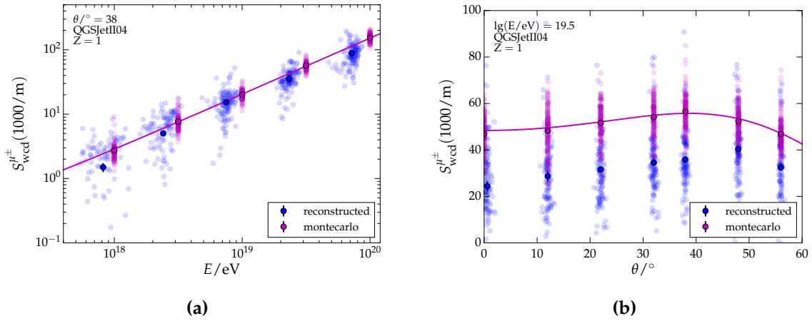
Figure 4.14: Monte-carlo and reconstructed muonic signals in the WCD, S_{wcd}^{\mu\pm} , as a function of (a) energy and (b) zenith. Also plotted by magenta lines is the parameterization to Monte-carlo data to obtain the zenith and energy independent estimator muon content estimator R_{38}^\mu .
