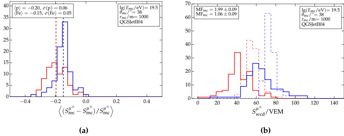
Figure 4.12: (a) Biases in reconstructed muonic signal in the WCD for ensembles of proton and iron primaries with energies of 10^{19.5} eV and zenith angle of 38^\circ . The standard deviation of these distributions is taken to be the bias resolution, which must be added in quadrature with the resolution of the reconstructed signal to obtain the total uncertainty. (b) Distributions of reconstructed (solid lines) and Monte-carlo (dashed lines) muonic signals in the WCD for ensemble of proton and iron primaries of the same Monte-carlo energy and zenith angle.
