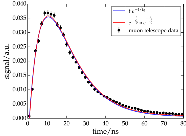
Figure 3.10: Fit of a model of two subsequent exponential decays to signals of the SSD from particles crossing at its end furthest from the PMT where the distance traveled by the two legs of the signal is equal. This two parameter model may be simplified to a function with one parameter since the decay constants are very similar in magnitude.
