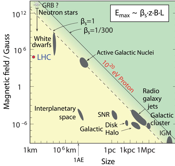
Figure 1.3: Hillas plot depicting potential astrophysical sites for the acceleration of particles and nuclei [6]. Strong candidates for 10^{20} \text{ eV} protons have yet to be identified.
