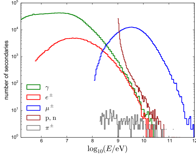
Figure 3.6: Spectrum of background flux of cosmic rays arriving at ground from low energy showers. A set of 10^5 10 GeV muons was used for first-order tuning as this energy is close to the peak of the energy spectrum of atmospheric muons, which primarily compose the data sample of the muon telescope. The vertical muons were simulated uniformly over the surface of the SSD with injection positions a few centimeters above the aluminum frame. Figure from [32].
