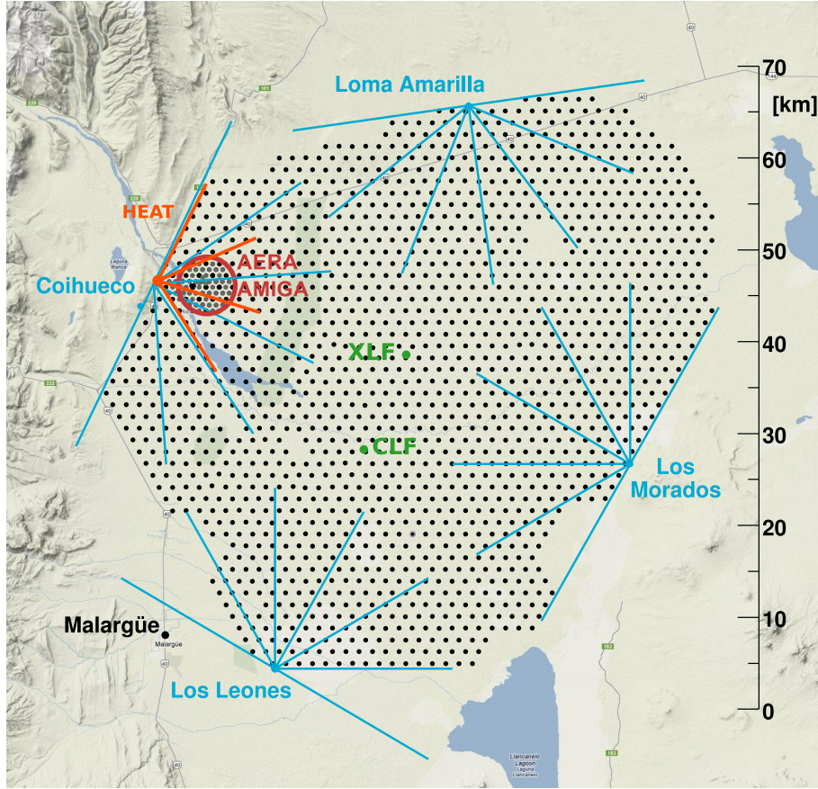
Figure 1.5: Schematic depiction of the Pierre Auger Observatory. Each black dot represents one surface detector station. The blue lines represent the fields of view of the four sites housing fluorescence telescopes. The orange lines represent additional high-elevation telescopes for observation of showers induced by lower energy primaries. The locations of the observatory's two laser facilities used for calibration of the fluorescence telescopes (the CLF and XLF) are also depicted. The denser array with a spacing of 750 m between surface detectors is also depicted. Each of these stations in the denser array will be accompanied by a 30 \text{ m}^2 buried muon counter for the direct detection of the muon component of EAS.
