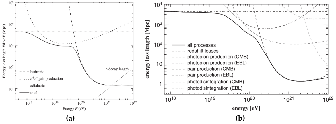
Figure 1.2: (a) Energy loss length for protons for various processes. (b) Energy loss length for iron nuclei for various processes.
