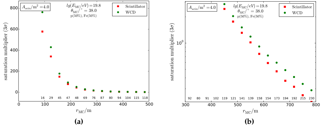
Figure 2.10: The saturation multiplier plotted as a function of distance from the shower axis in (a) linear and (b) logarithmic scale. From the linear scale, it is clear that the demands on the upper limit of the dynamic range begin to rapidly increase at around 200 m from the shower axis. The logarithmic scale shows that the rate at which the demand increases is not exactly equal between the WCD and scintillator, which is important to consider when determining the hardware and gain settings for the two sub-detectors if they should be able to measure up to the same distances from shower axes. This difference can likely be attributed to differing slopes in the two sub-detectors' lateral signal distributions and the compositional makeup of their respective signals. The numbers at the bottom of the plots give the number of simulated stations used in the given bin for calculations.
