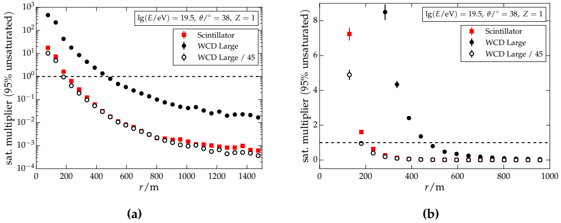
Figure 3.14: Saturation multiplier to guarantee less than 5% saturated stations as a function of distance in (a) logarithmic and (b) scales. The linear scale makes evident the range in distance where the slope of the LDF becomes very steep and demands on the upper limit of the dynamic range rapidly become unreasonable. Both the SSD and the planned small PMT in the WCD saturate at approximately the same distance, which is approximately 200 m for the energy and zenith angle depicted here.
