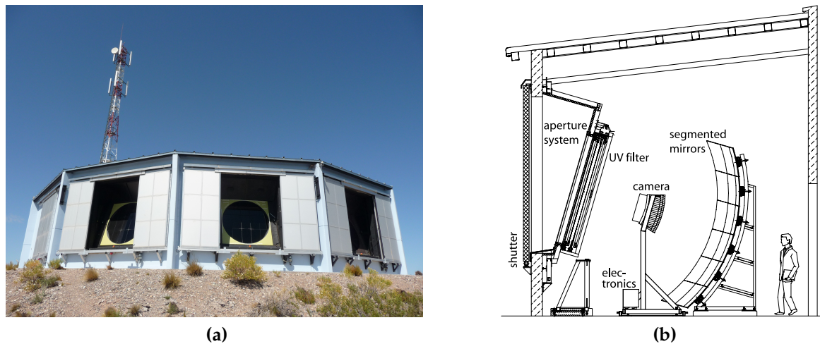
Figure 1.7: (a) Fluorescence detector site in which individual telescope bays may be observed [8]. (b) Schematic of a telescope bay [8].
