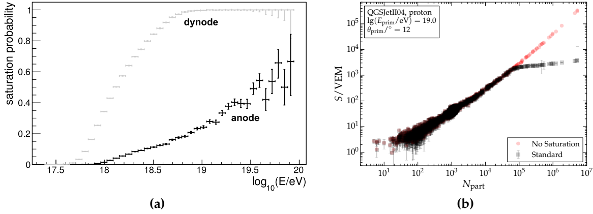
Figure 3.16: (a) Saturation probability as a function of the primary energy (in Auger data [35]). Signal estimation switches from using the dynode to the low-gain anode trace as soon as the former is saturated. Anode saturation is only partially recoverable with some empirical methods. (b) Dependence of station signal S on the number of injected particles N_{\text{part}} . Around a particular particle number, the dependency changes due to anode saturation.
