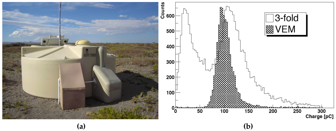
Figure 1.6: (a) Picture of a surface detector station [7]. (b) Sample calibration histogram of a surface detector station [7]. Signals are calibrated to the response of one vertical, through-going, muon (hatched “VEM” histogram) via the relationship with the histogram of signals from all the atmospheric particles triggering the detector in a one minute time span (“3-fold” histogram).
