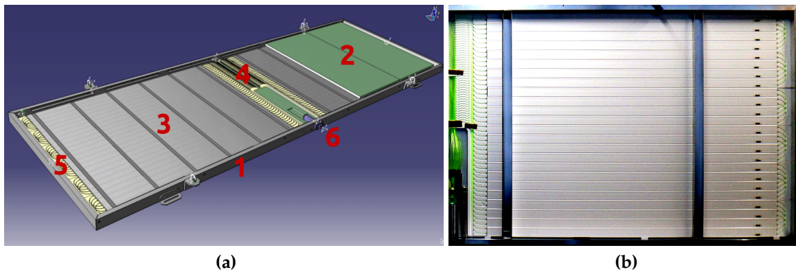
Figure 2.13: (a) Schematic depiction of an open SSD. (b) Top-down picture of one side of an open SSD. The contrast on this image has been significantly increased to increase the visibility of the optical fibers.
