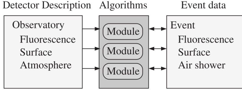
Figure 3.1: Structure of detector description and event interfacing with simulation and reconstruction algorithms (taken from [28]). While the detector description contains static or slowly changing information, the event contains data specific to the air shower in question. Modules may read from both the detector description and the event and write newly calculated information to the event.
