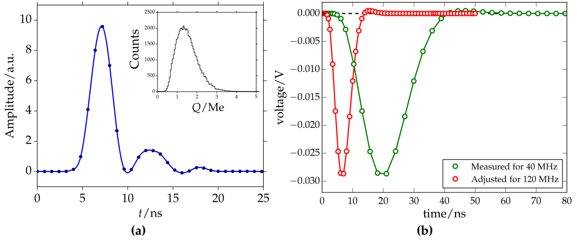
Figure 3.13: (a) Pulse shape and charge distribution (inset) for properly amplified photoelectrons as measured using the the muon telescope setup. The small second peak may be due to unresolved issues in the determining the start times of these pulses or elsewhere in pulse-finding algorithms applied to the telescope data. (b) Transfer function measured for Auger's 40 MHz electronics along with scaled version used for the 120 MHz simulations up to the present.
