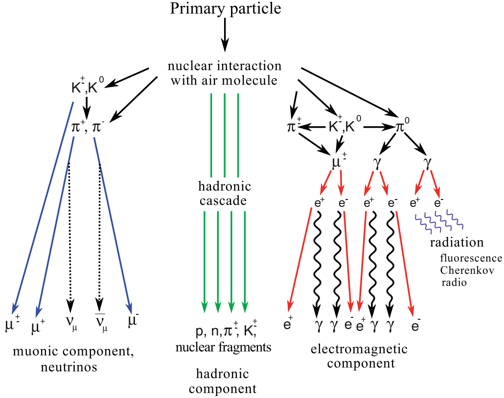
Figure 1.4: Schematic depiction of the hadronic, electromagnetic, and muonic components of EASs.
