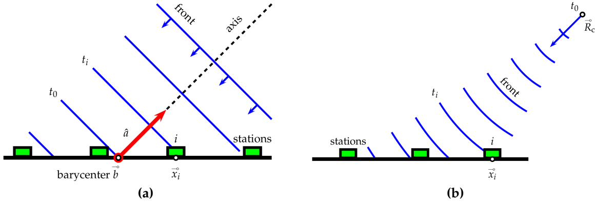
Figure 1.10: (a) Schematic depiction of the definition of the planar front assumption. (b) Schematic depiction of the spherical shower front assumption.
