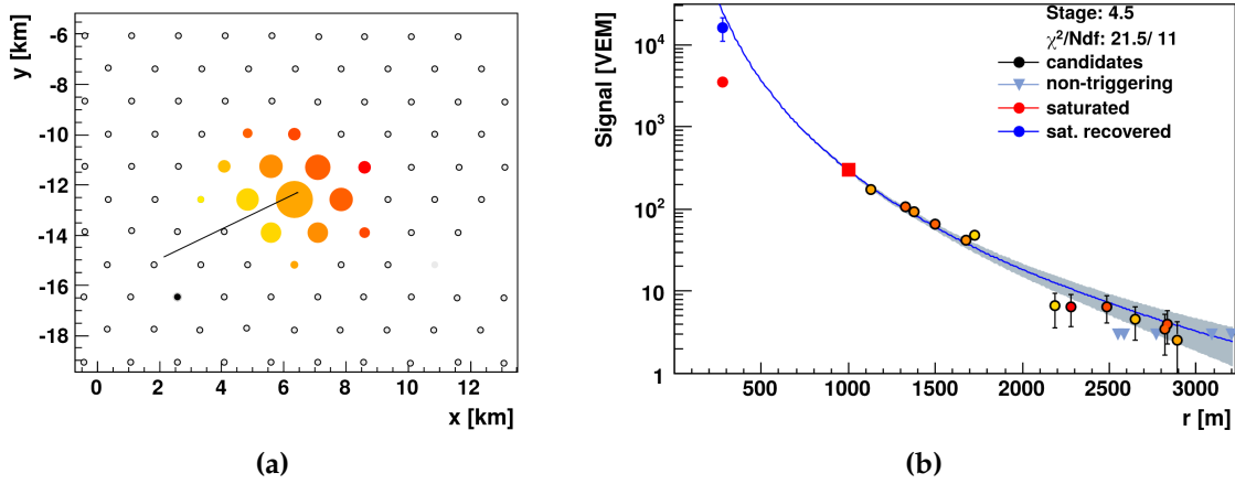
Figure 1.11: (a) Top-down schematic view of the footprint of an EAS on the surface detector array. The size of the circles corresponds to the magnitude of the signals whereas the coloring corresponds to signal start times. The black line represents the shower axis. (b) Fit of the lateral distribution function for the same event. The station closest to the shower axis was saturated, but the signal was recovered. Non-triggering stations, which may be observed at the larger distances, are depicted with downward facing equilateral triangles.
