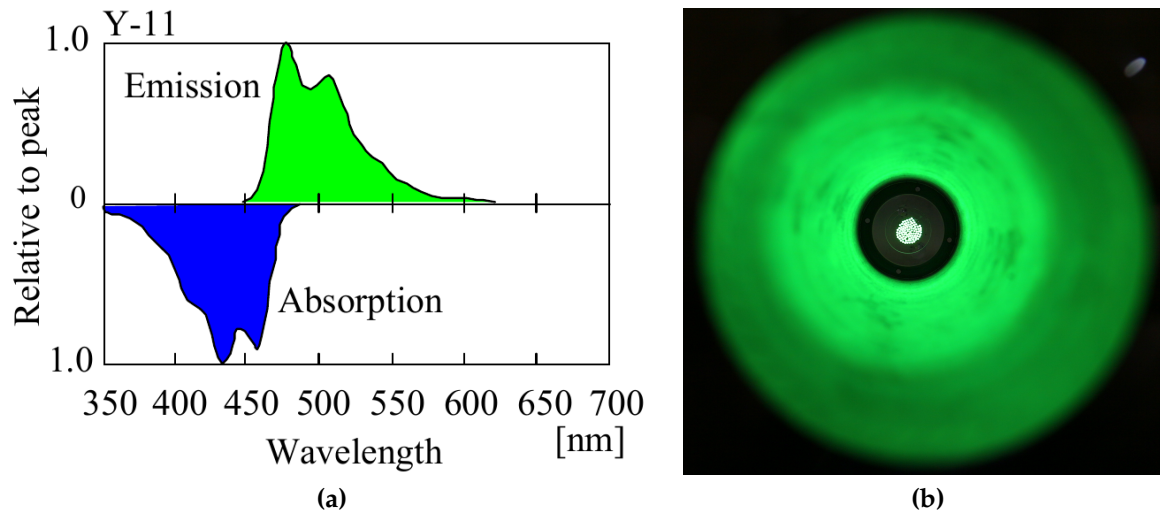
Figure 2.12: (a) Absorption and emission spectra of the K-27 wavelength shifting dye [25] in the Y-11 (300) MSY fibers produced by Kuraray [24] and chosen for the SSD. (b) Optical fiber bundle inside a PMMA cookie as seen by looking down the readout device tube of the SSD.
