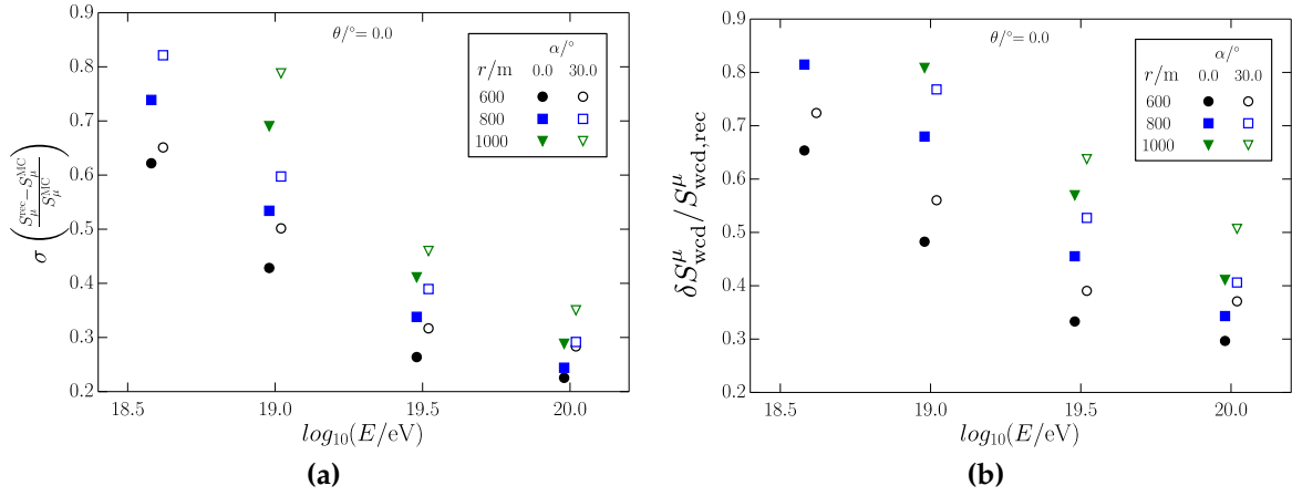
Figure 2.7: (a) Resolutions of the reconstructed muonic signal of the WCD for instances where the sub-detector signals are correlated (filled markers, \alpha = 0^\circ ) and uncorrelated (open markers, \alpha = 30^\circ ). These instances approximately correspond to scenarios where the scintillator is positioned, respectively, on top of and beside the WCD. (b) Analytically propagated resolutions of the matrix formalism for \alpha = 0^\circ and 30^\circ (approximately corresponding to instances where signals are respectively correlated and uncorrelated). These resolutions are systematically greater than those calculated through direct comparison of reconstructed and Monte Carlo quantities. A number of possible explanations exist for this offset. One such explanation is the use of an average resolution derived from all signals within an energy, zenith, distance bin instead of a yet to be determined single station resolution. Further investigation is required. Nonetheless, the general trends in the differences between resolutions with and without correlated signals are similar.
