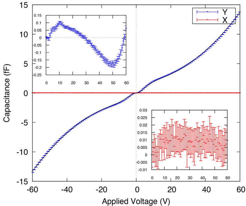
Fig. 5. Capacitance as function of the applied voltage V_{act} . For Y axis, V_{act} > 0 \text{ V} , while for X axis, V_{act} = 0 \text{ V} . Each data point is the mean value of 50 samples per V_{act} step of 1 V. The lines are fits using Eq. (9). The inset to the left is the deviation of Y_p from the fit. The inset to the right is a zoom in to X_p data.
