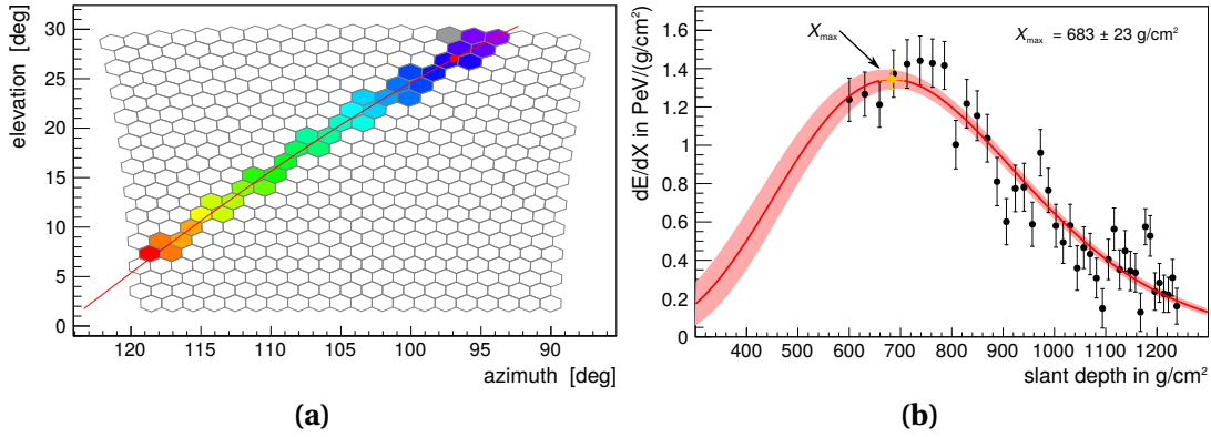
Figure 4.10: Event reconstruction of the Fluorescence Detector of the same example event as in Fig. 4.6b. (a) Light trace measured in the pixel camera of one of the telescopes. The color denotes the arrival time of the light in the pixels, from early times in violet to late times in red. (b) Reconstructed longitudinal shower profile of the energy deposited in the atmosphere. The maximum of the profile corresponds to X_{\max} , which is reconstructed to (683 \pm 23) \text{ g/cm}^2 . Figures are extracted from the Offline EventBrowser.
