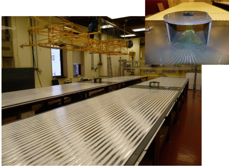
Figure 3.7: AMIGA module in the laboratory A module during production in the laboratory. The inset photo shows the fiber routing to the optical connector. Figure is taken from [70].
