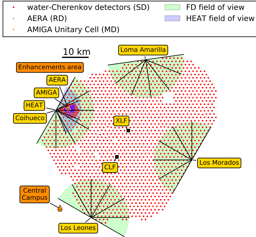
Figure 3.1: Map of the Pierre Auger Observatory The Surface Detector (SD) array comprises water-Cherenkov detectors on a grid of 1500 m spacing. It spans an area of 3000 km 2 . The array is overlooked by the Fluorescence Detector (FD), which is located at four telescope sites at the perimeter of the array. Close to the Coihueco site, the enhancements area is located, including the high elevation telescopes HEAT, the infilled area of water-Cherenkov detectors and buried muon scintillators (MD) of AMIGA and the radio antenna array AERA (RD). For a zoom in the enhancements area see Fig. 3.4.
