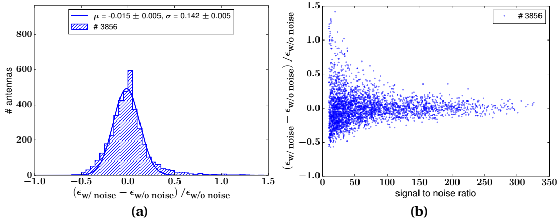
Figure C.3: Biases on the energy fluence by added background (a) The example event is combined with 500 different background events. The resulting energy fluences in the antennas is compared to the reconstruction of the event without background. A small bias of -1.5\% is observed, but a spread of 14.2\% is caused by the added background. (b) The relative difference of the energy fluences including and excluding background are shown over the signal-to-noise ratio. The spread decreases with increasing signal-to-noise ratio.
