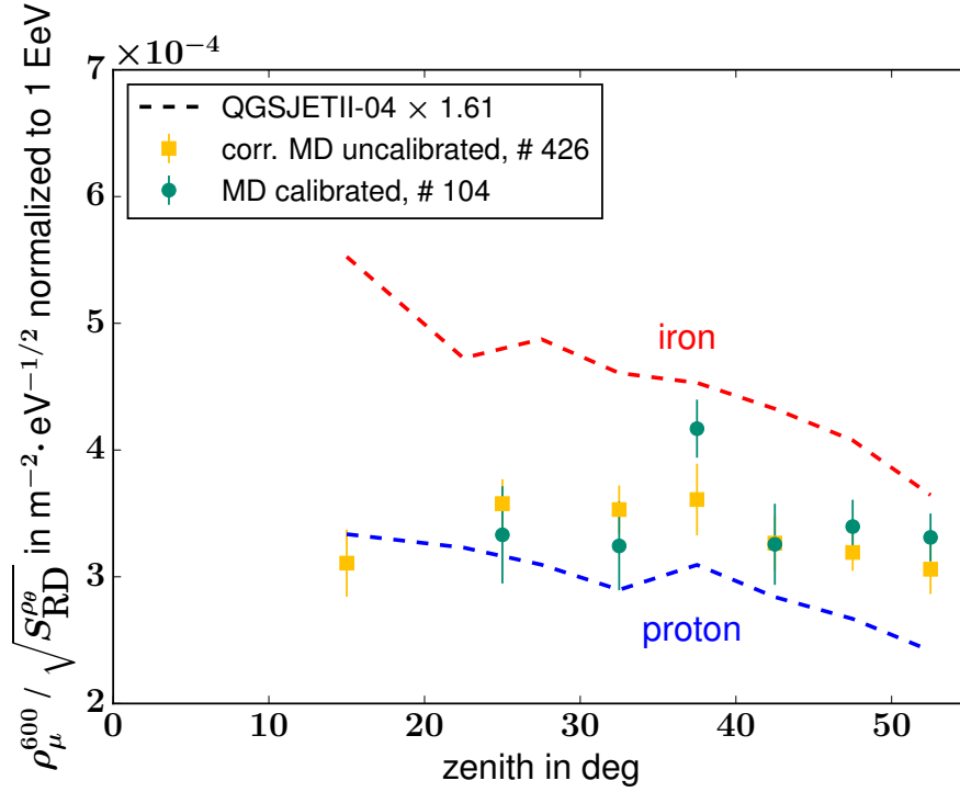
Figure 7.10: Zenith angle dependence The ratio \rho_\mu^{600} / \sqrt{S_{RD}^{\rho_\theta}} shows no dependence on the zenith angle in the zenith angle range of the measurements. However, from simulations a decrease towards higher zenith angles is expected. This discrepancy indicates zenith angle dependent effects not considered in the air-shower simulations or in the simulated detector response. (Error bars depict the uncertainty on the mean \sigma / \sqrt{N} ).
