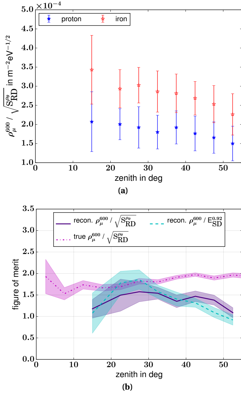
Figure 6.10: Zenith angle dependence of the ratio between the muon density and the square root of the radiation energy (a) The ratio including the detector simulation shows a similar behavior as for true values (see Fig. 5.9). However, the absolute values are larger by about 35 percent due to the reconstruction biases on the radiation energy as well as on the muon density. (b) The figure of merit is decreased for the reconstructed ratio of the muon density and the radiation energy by about 0.5 compared to the true values due to additional uncertainties arising from the detection technique, the reconstruction method and the added radio background. Using the SD energy instead of the radiation energy, the mass separation power is enhanced slightly at small zenith angles, but decreased towards larger zenith angles.
