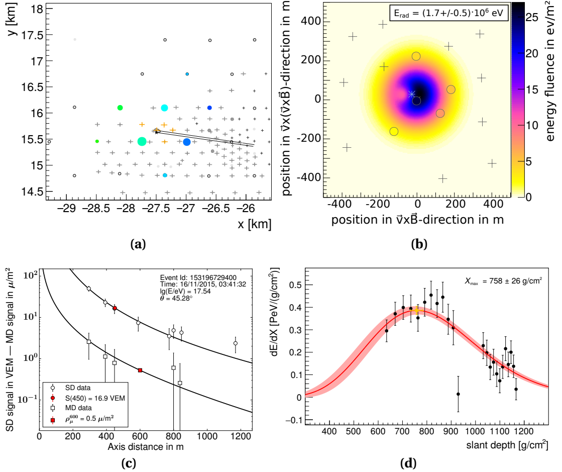
Figure 7.4: 4-fold example event The event was detected in 8 Surface Detector stations, 5 Muon Detector stations, 5 Radio Detector stations and 1 telescope (Coihueco). The arrival direction was reconstructed from the SD to a zenith angle of \theta = (45.3 \pm 0.5)^\circ and an azimuth angle of \varphi = (350.5 \pm 0.6)^\circ , the primary energy to (3.49 \pm 0.40) \times 10^{17} \text{ eV} . The radiation energy was reconstructed from the RD signal and is corrected for the zenith angle dependence to (1.88 \pm 0.52) \times 10^6 \text{ eV} . The shower maximum X_{\text{max}} was reconstructed to (758 \pm 26) \text{ g}/\text{cm}^2 from the FD signal. (a) SD and RD array (b) reconstructed two-dimensional LDF of the RD signal. (c) reconstructed one-dimensional LDFs to the SD and the MD signals. (d) Reconstructed longitudinal profile of the energy deposit of the shower in the atmosphere.
