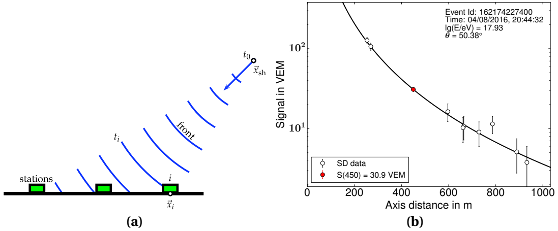
Figure 4.6: Event reconstruction of the Surface Detector (a) Direction reconstruction based on signal arrival times. The shower particles travel with a shower front of \mathcal{O}(1\text{ m}) thickness. The arrival direction is reconstructed by fitting a shower front model to the arrival time residuals in the detectors. Figure is taken from [67]. (b) Example of a lateral distribution function fitted to the signal sizes detected at different distances to the shower axis of the measured event 162174227400. The energy is reconstructed to 8.54 \pm 0.53 \pm 0.37 \cdot 10^{17} eV, based on S(450) = 30.9 \pm 1.9 \pm 1.3 VEM. The shower direction is reconstructed to a zenith of \theta = (50.4 \pm 0.4)^\circ and an azimuth of \varphi = (318.7 \pm 0.4)^\circ .
