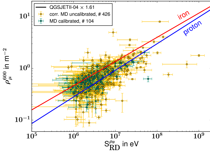
Figure 7.9: Correlation of the measured muon density and radiation energy of events measured in coincidence by AERA and the AMIGA MD in the time periods with uncalibrated and calibrated MD. For comparison, the correlation derived from air-shower simulations of proton and iron showers including detector responses of AERA and AMIGA are drawn. The measured events at the Pierre Auger Observatory contain on average 61 % more muons than predicted by the hadronic interaction model QGSJETII-04, which is corrected for in the fits shown here. The muon densities measured with the uncalibrated MD are corrected for the underestimation by 31 % compared to calibrated events.
