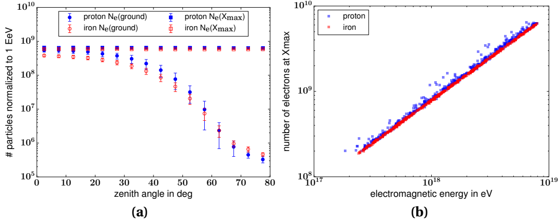
Figure 5.5: True number of electrons at X_{\text{max}} and at the ground above an energy of 250 keV.
