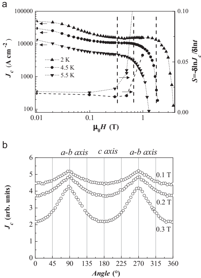
Fig. 2. (a) Magnetic field dependence of J_c and the creep rate S = -(d(\ln J_c)/d(\ln t)) in the \text{Ba}(\text{Fe}_{0.86}\text{Co}_{0.14})_2\text{As}_2 single crystal. Vertical dashed lines indicate the fast creep crossover or change in the vortex dynamics regime. (b) Angular dependent critical current density, J_c(\theta) at 9 K and \mu_0 H = 0.1, 0.2 and 0.3 T in the \text{Ba}(\text{Fe}_{0.86}\text{Co}_{0.14})_2\text{As}_2 single crystal.
