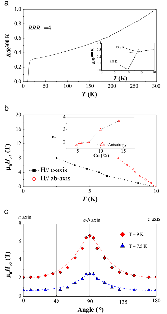
Fig. 1. (a) Temperature dependence of the normalized resistance of an annealed \text{Ba}(\text{Fe}_{0.86}\text{Co}_{0.14})_2\text{As}_2 single crystal. The inset shows a vicinity of the superconducting transition and the criteria used for the T_c determination. (b) Temperature dependence of the upper critical fields ( H_{c2} ) in an annealed \text{Ba}(\text{Fe}_{0.86}\text{Co}_{0.14})_2\text{As}_2 single crystal. Inset shows the Co doping dependence of the anisotropy ( \gamma_{T \rightarrow T_c} = H_{c2}^c/H_{c2}^{ab} ) taken from Refs. [39,40], and this work. (c) Upper critical field ( H_{c2} ) versus angle ( \theta ) at 9 K and 7.5 K. Single-band model [4] calculations with anisotropic scaling are also shown (dashed lines). Same type of fitting at the same T/T_c ratios are obtained by considering H_{irr} .
