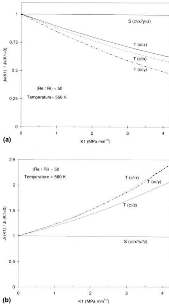
Fig. 2. (a) Flux of vacancies J_v (in units of J_v(K1=0) ) and (b) flux of interstitials J_i (in units of J_i(K1=0) ) to a crack in a Mg crystal modelled with an empirical potential vs. the intensity factor K1 . Three different crystal orientations are considered. T and S on the curves indicate the crack tip and the crack surfaces, respectively. Temperature = 560 K. R_c/R_i = 50 .
