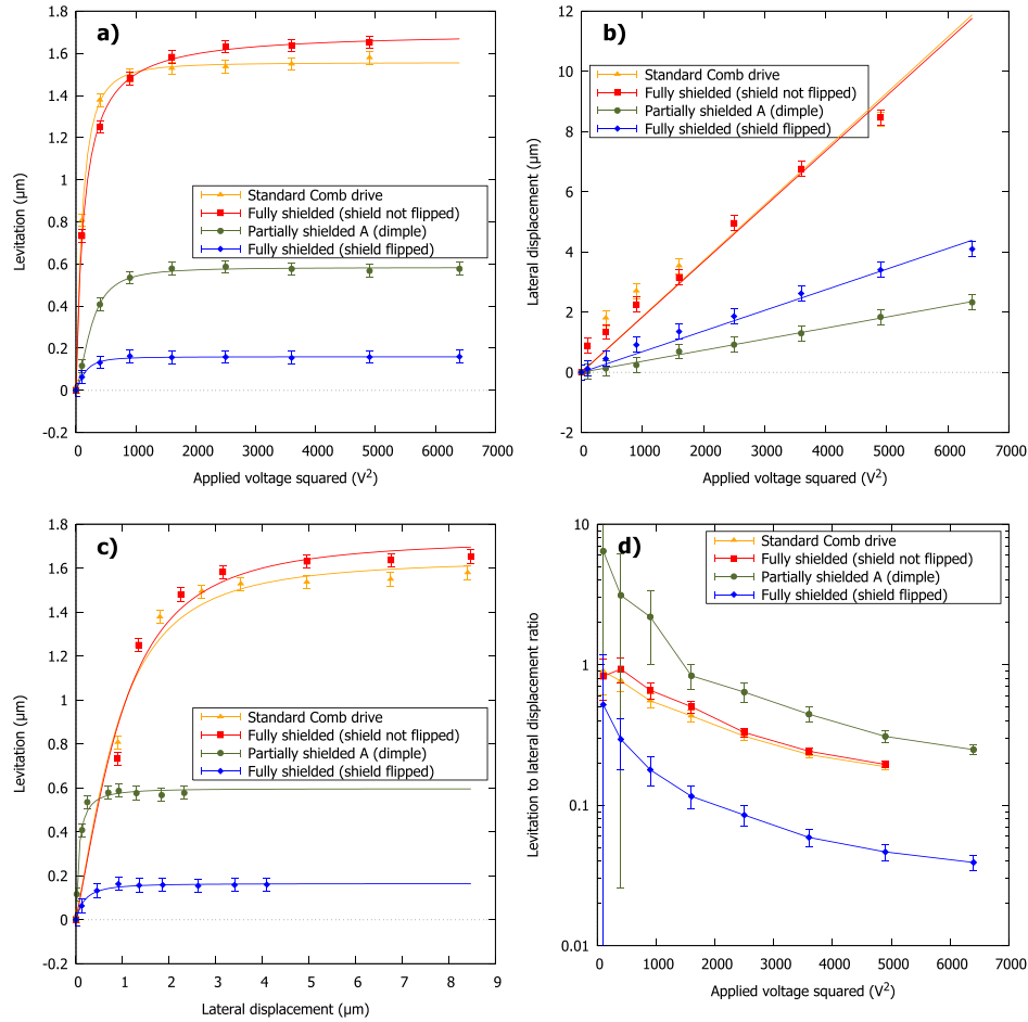
Fig. 6. a) Levitation vs. drive voltage squared for designs with its respective fits (lines). b) Lateral displacement vs. drive voltage squared for all designs. The linear fit approximates the idealized response, most valid as the levitation vanishes. After the levitation saturates the lateral displacement becomes more precisely proportional to V^2 . c) Comparison of vertical and lateral displacement for all the devices fabricated. d) Levitation to lateral displacement ratio vs. drive voltage squared.
