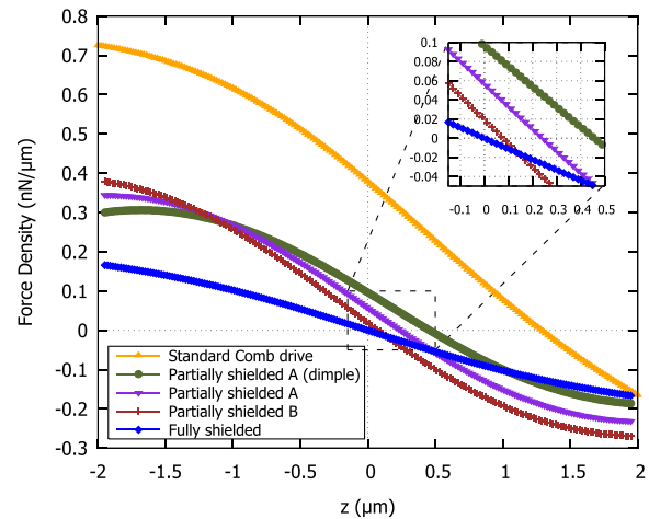
Fig. 7. Simulation of lateral force density at a given drive voltage (10 V) in the overlapped region L_0 as a function of comb finger offset. Inset: Close-up view of the zero crossing, corresponding to the expected levitation amplitude.
