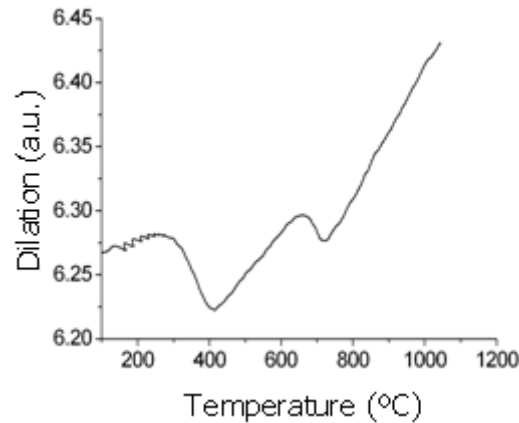
FIG 1. Dilation as a function of temperature for the sample cooled at 50 °C/h.
